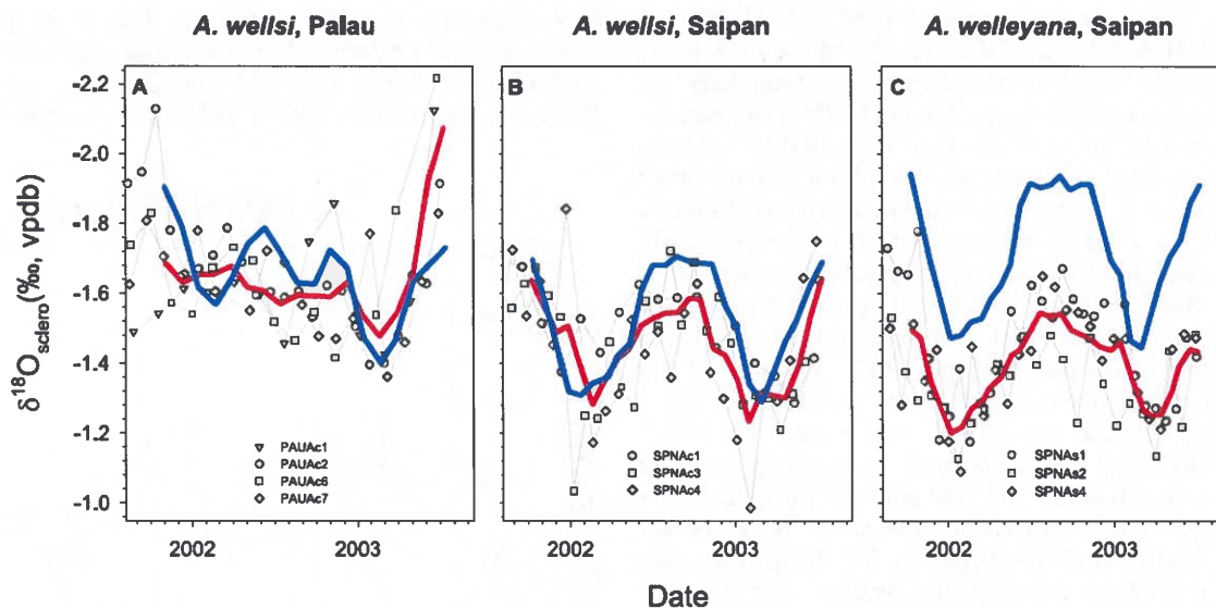
Figure 4. High-resolution sclerosponge \delta^{18}\text{O} for (a) A. wellsi in Palau, (b) A. wellsi in Saipan, and (c) A. willeyana in Saipan. Measurements made at 0.1 \text{ mm} increments in all specimens are shown with gray symbols. Each record was interpolated before calculating the average sclerosponge \delta^{18}\text{O} record (solid red line) in each panel according to methods outlined in section 2.7. Predicted equilibrium skeletal \delta^{18}\text{O} values (blue lines) were calculated by using equations by Grossman and Ku [1986] for the aragonitic A. willeyana and equations by Kim and O'Neil [1997] for the high-Mg calcitic A. wellsi , with the addition of 0.06\text{‰} for each mol% Mg according to Tarutani et al. [1969]. A. wellsi were 21 mol% Mg in this study. Seawater temperature and in situ \delta^{18}\text{O}_{\text{sw}} records (data shown in Figure 2) were interpolated in the same way as the sclerosponge data for each species and location, and the interpolated data were used to calculate the equilibrium skeletal \delta^{18}\text{O} records.
