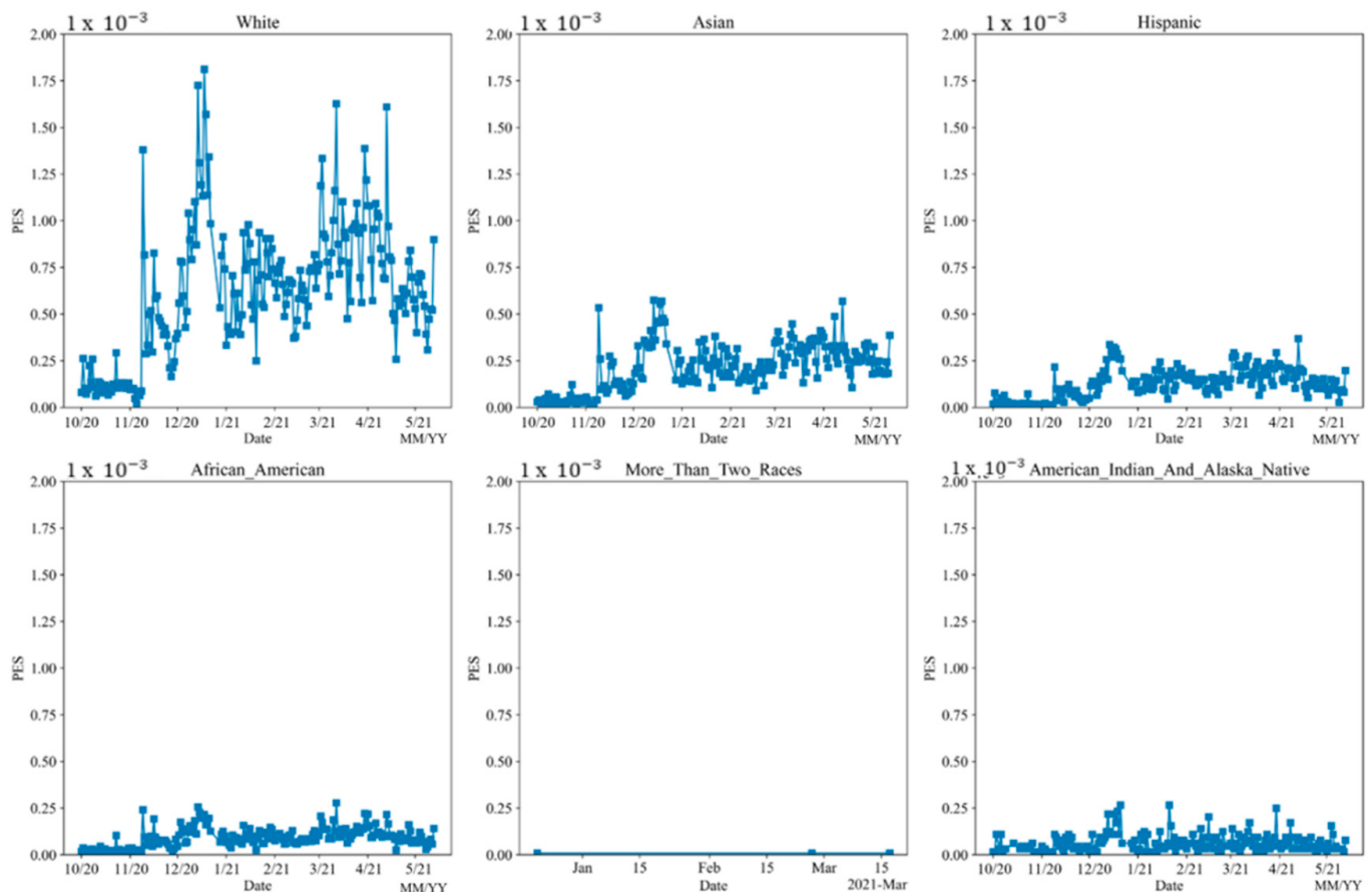
Figure 11. PES analysis on different races from 1 October 2020 to 21 May 2021.
