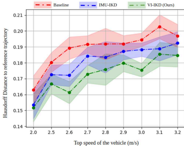
Fig. 6: Hausdorff distance (lower is better) between trajectories traced by different algorithms at different top speeds of the vehicle in the indoor evaluation environment. We see that VI-IKD is the most accurate compared to the receding horizon controller with no IKD model (baseline) and IMU-IKD [6].
