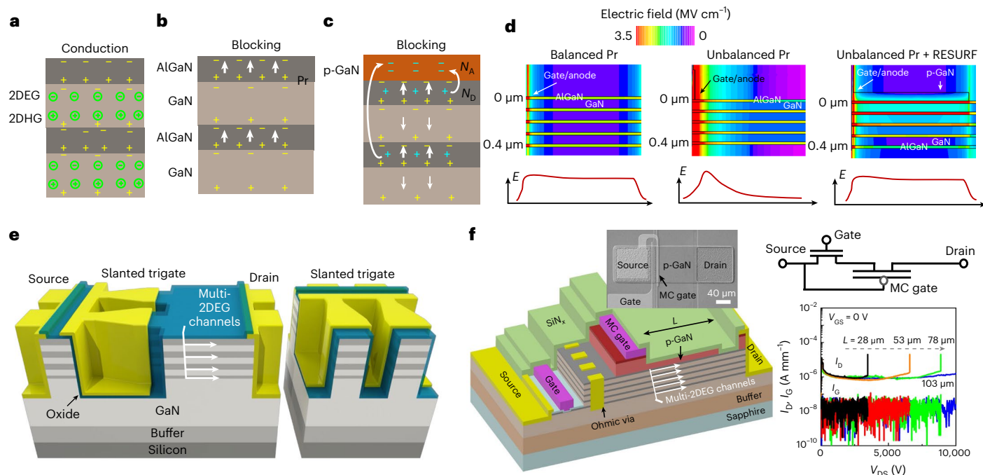
Fig. 4 | Multi-channel heterostructures and multi-channel power HEMTs. a, Illustration of an undoped multi-channel with balanced polarization charges (Pr) in the forward conduction state, in which alternate pairs of 2DEG and 2DHG are formed. b, Illustration of an undoped multi-channel with balanced polarization charges in the high-voltage blocking state, forming a polarization superjunction. c, Illustration of a doped multi-channel in the blocking state, on top of which a p-GaN RESURF layer provides acceptors ( N_A ) to balance the net donors ( N_D ) in the multi-channel. d, Simulated electric-field contours in two undoped multi-channels with and without balanced polarization charges, as well as a doped multi-channel with the p-GaN RESURF structure, all at a high blocking voltage.
