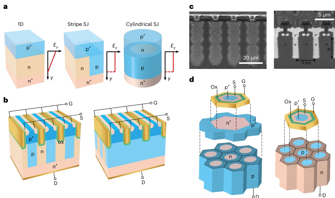
Fig. 3 | Superjunction power devices. a , Schematic of the 1D drift region, 2D superjunction and cylindrical superjunction. The electric-field distribution along the thickness direction ( E_y ) is illustrated for three drift region designs. b , Two implementations of the 2D superjunction trench MOSFET. The superjunction pillars can be parallel to the trench width or perpendicular to it. c , Cross-sectional microscopic images of a silicon superjunction (left) and a SiC superjunction (right). S, source; D, drain. d , Exploded views of two implementations of the
