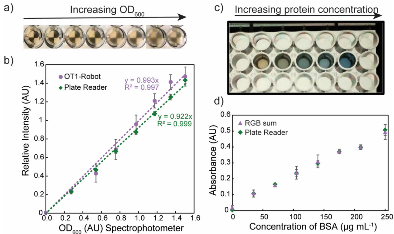
Figure 4. a) Photograph of wells measured via turbidometry-based automated OD 600 measurements; b) OD 600 measured on a traditional spectrophotometer (1 cm path length) vs. intensity measured by OT-1 robot (purple) and plate reader (green), corrected for path length; c) Photograph of Bradford assay well with variable amounts of proteins; d) Bradford assay absorbance as a function of bovine serum albumin (BSA) concentration measured via least squares regression of photography-based assay from weighted red-green-blue (RGB) sums (purple) and by plate reader (green). Error bars represent the standard error across three replicates.
