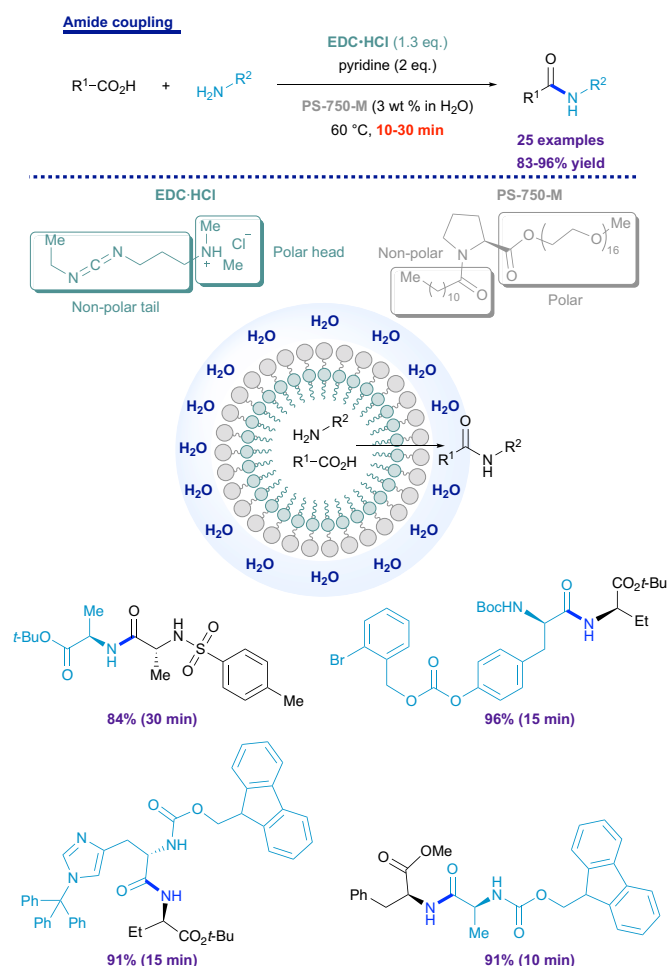
Scheme 6: Mixed micelles of PS-750-M and EDC•HCl for fast and epimerization-free amide couplings.
