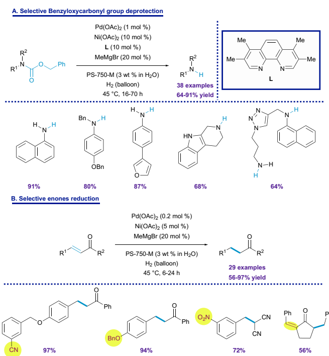
Scheme 8: Selective Ni(0)Pd(0) bimetallic catalysis in water.
