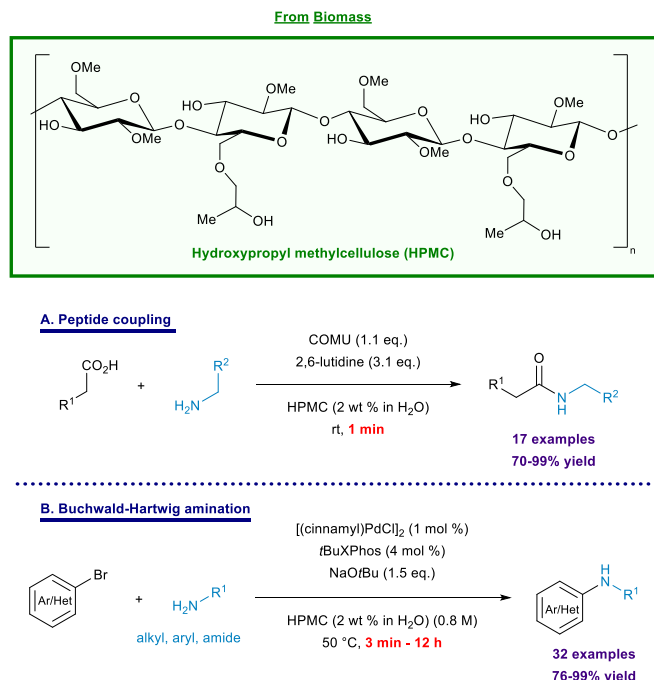
Scheme 15: Representation of Hydroxypropyl methylcellulose (HPMC) and application for A. Peptide coupling and B. Buchwald-Hartwig amination.
