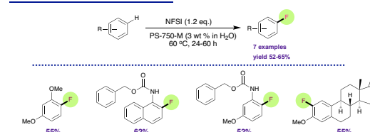
Scheme 4: Selective monofluorination of N -protected indoles and arenes.
