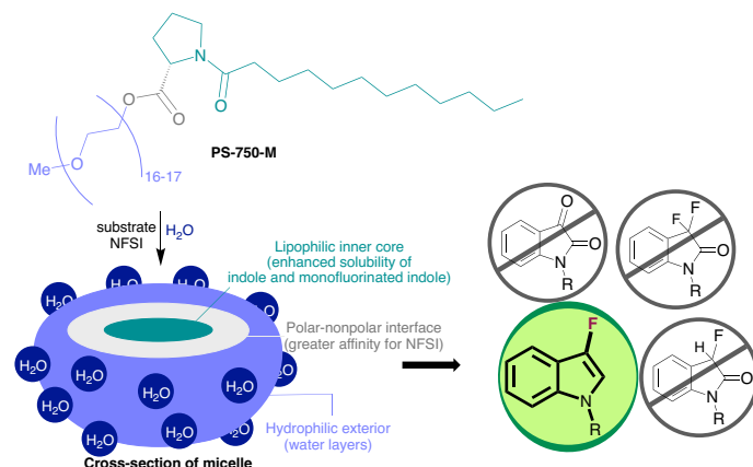
Scheme 3: Shielding and compartmentalization effect for selective monofluorination of indoles.
