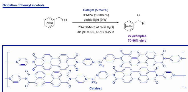
Scheme 7: Micellar photocatalysis mediated by heterogeneous catalyst.
