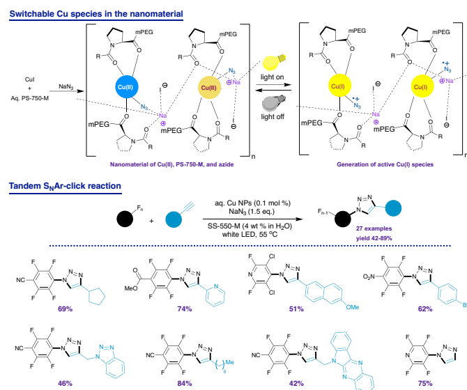
Scheme 5: Oxidation state switchable nanomaterial for ppm level Cu(I) catalysis in water.
