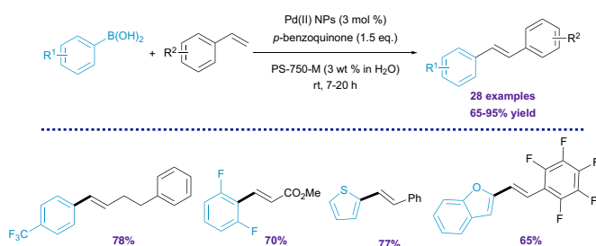
Scheme 9: Ligand-free ultrasmall Pd(0) nanoparticles for Mizoroki-Heck-type couplings.
