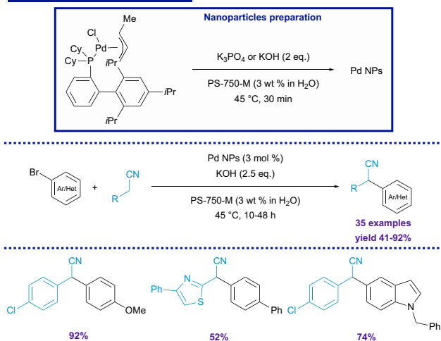
Scheme 2: Pd nanoparticles-catalyzed \alpha -arylation of nitriles.
