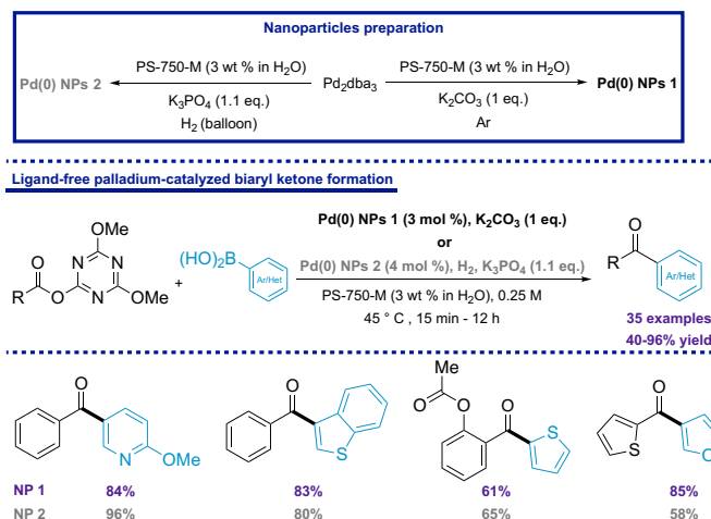
Scheme 11: Synthetic versus natural ligand-free nanoparticles for cross-couplings of water-sensitive carboxylic acid derivatives in aqueous micelles.
