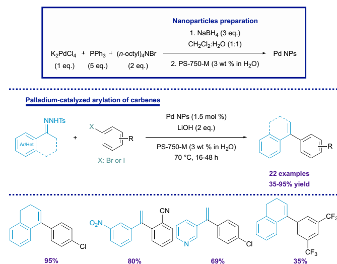
Scheme 12: Pd-catalyzed arylation of carbenes in micelles of PS-750-M.
