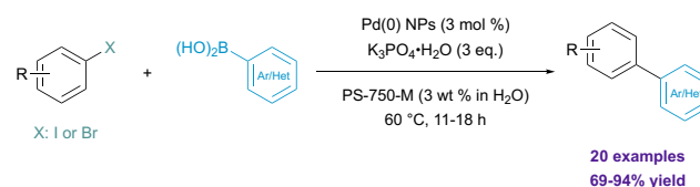
Scheme 10. Ligand-free Pd(0) nanoparticles for Suzuki-Miyaura couplings.
