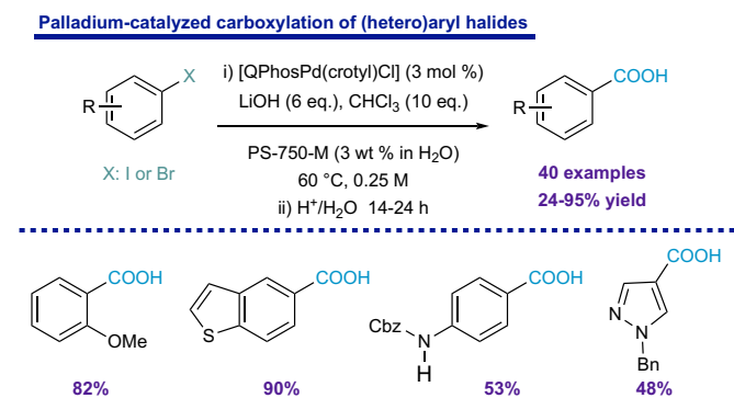
Scheme 13: Carbanion-mediated catalytic carboxylic acid formation in water.
