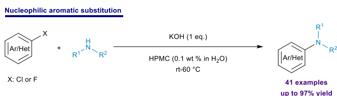
Scheme 16: Nucleophilic aromatic substitution in water using HPMC as additive.
