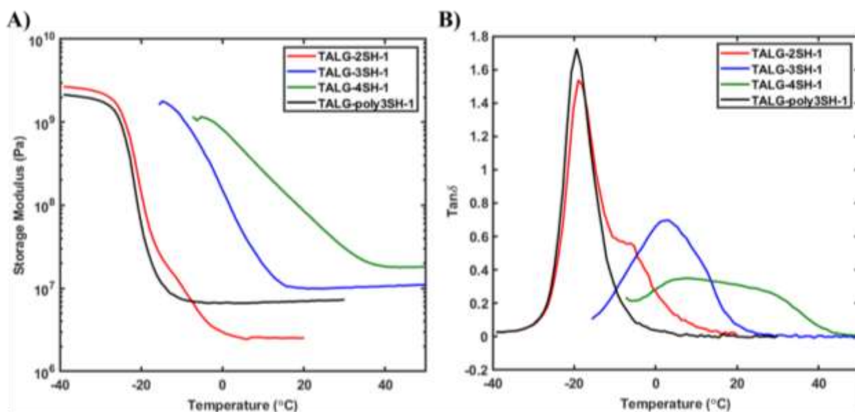
Figure 4 DMA curves depicting A) storage modulus and B) \tan \delta for 1:1 thiol:ene networks.
