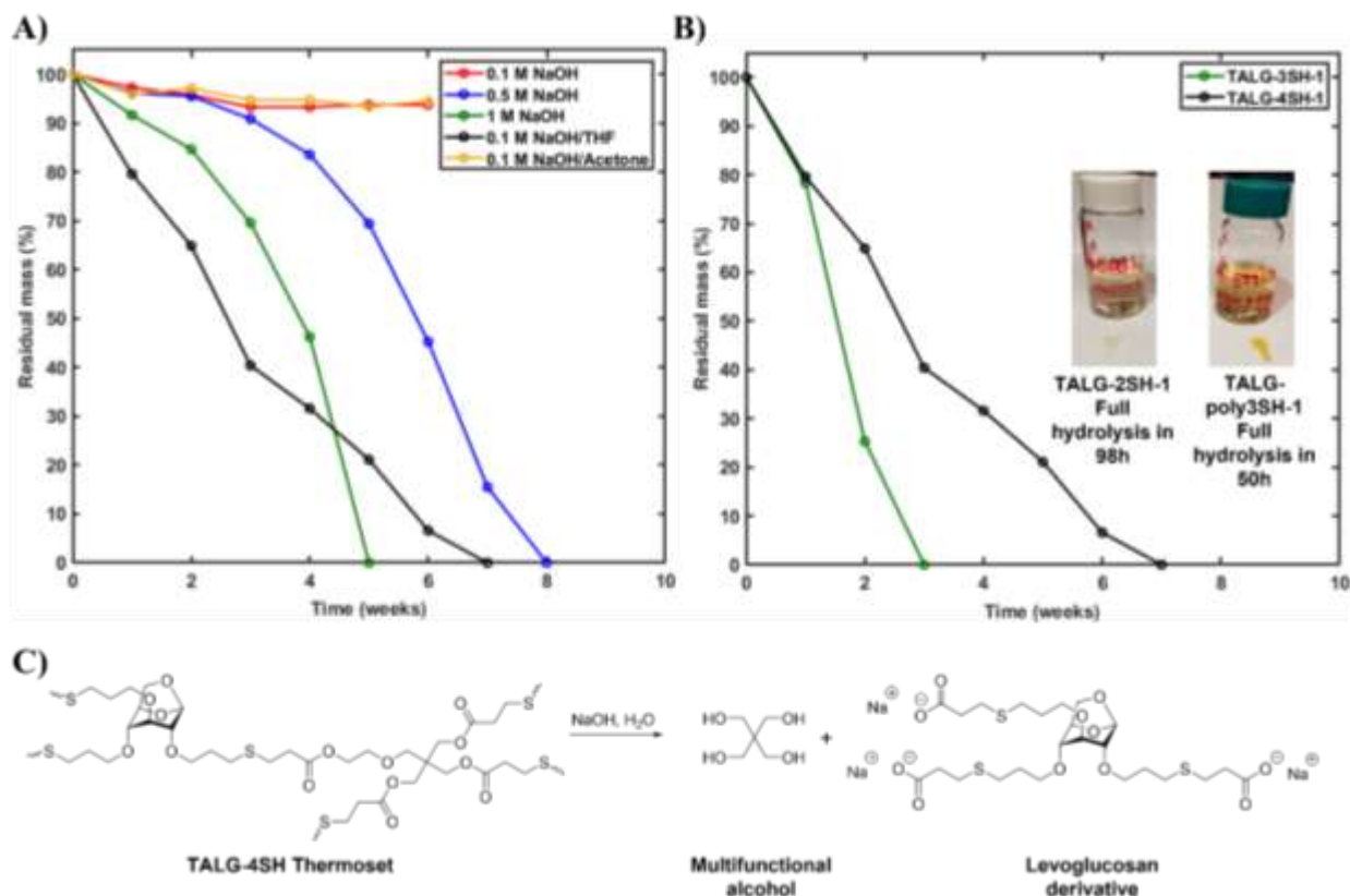
Figure 5 A) Mass loss of TALG-4SH-1 under different degradation conditions. B) Mass loss of different thermoset samples in 0.1 M NaOH/THF. C) Degradation of levoglucosan-based thermosets into alcohol and carboxylic byproducts
