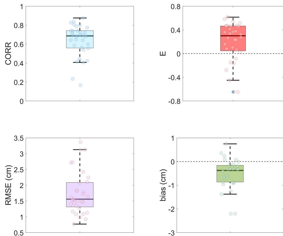
Figure 5. The statistical results of measured versus predicted \Delta DBH of all trees in the 32 plots of Harvard Forest. These results are based on the value of k_{ST} equal to 0.32 (ST: shade-tolerant) and the value of k_{SIT} equal to 0.90 (SIT: shade-intolerant). The results include four time periods of \Delta DBH: 2000–2005, 2000–2010, 2000–2015, and 2000–2010. CORR: correlation coefficient (i.e., r ); E: model efficiency; RMSE: root mean square error.
