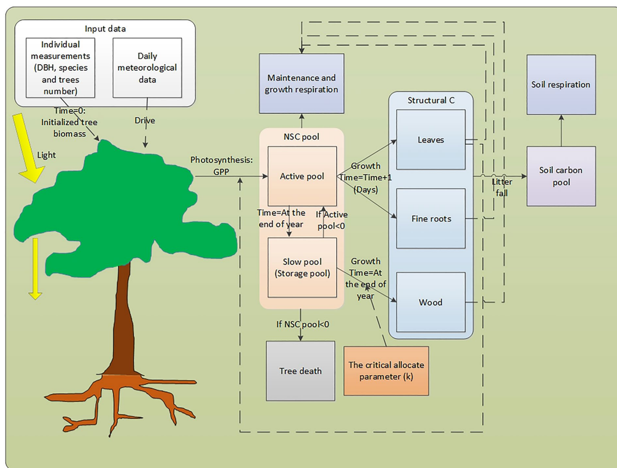
Figure 1. Schematic representation of the FORCCHN2 model. The dotted lines represent the input processes; the solid lines represent the flows of carbon. NSC: non-structural carbohydrates.
