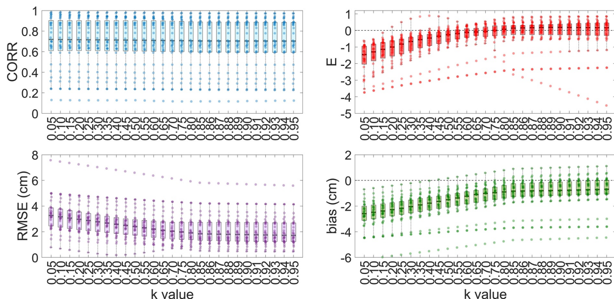
Figure 4. The statistical results of measured versus predicted ΔDBH of the shade-intolerant trees in the 32 plots of Harvard Forest. These results are based on 27 different values of the critical allocate parameter ( k ). The results include four time periods of ΔDBH: 2000–2005, 2000–2010, 2000–2015, and 2000–2020. CORR: correlation coefficient (i.e., r ); E: model efficiency; RMSE: root mean square error.
