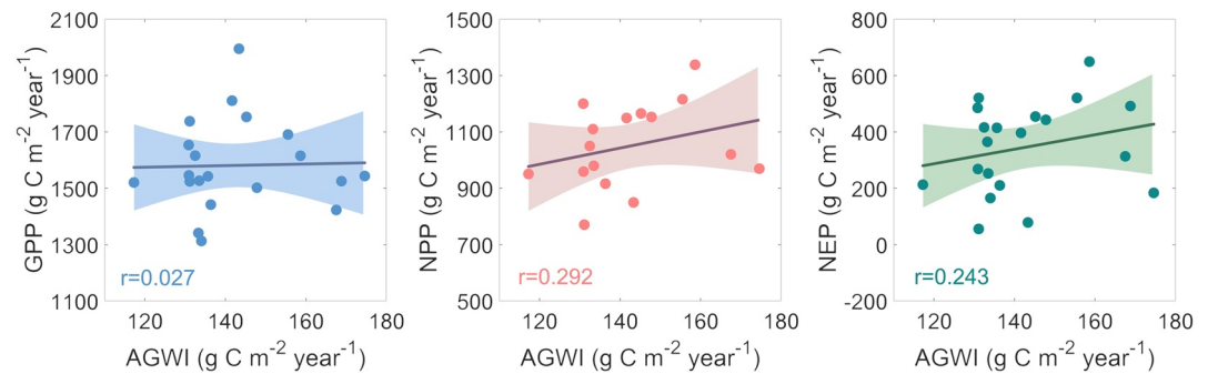
Figure 2. Correlation of annual aboveground wood growth increment (aboveground wood increment) with carbon flux at the 32 plots of Harvard Forest. The carbon fluxes include (a) the gross primary productivity (GPP), the available period is 2000–2019, (b) Net Primary Productivity, the available period is 2000–2015, and (c) Net Ecosystem Productivity, the available period is 2000–2019.
