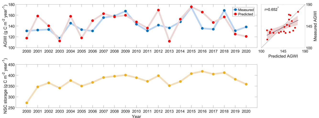
Figure 7. (a) Is measured versus predicted AGWI in Harvard Forest during 2000–2020, and the right is the corresponding scatter plot; (b) is the predicted non-structural carbohydrates storage increment at the annual scale. These results are based on the value of k_{ST} equal to 0.32 (ST: shade-tolerant) and the value of k_{SIT} equal to 0.90 (SIT: shade-intolerant). AGWI: aboveground wood growth increment; NSC: non-structural carbohydrates. * means the significance is less than 0.05.
