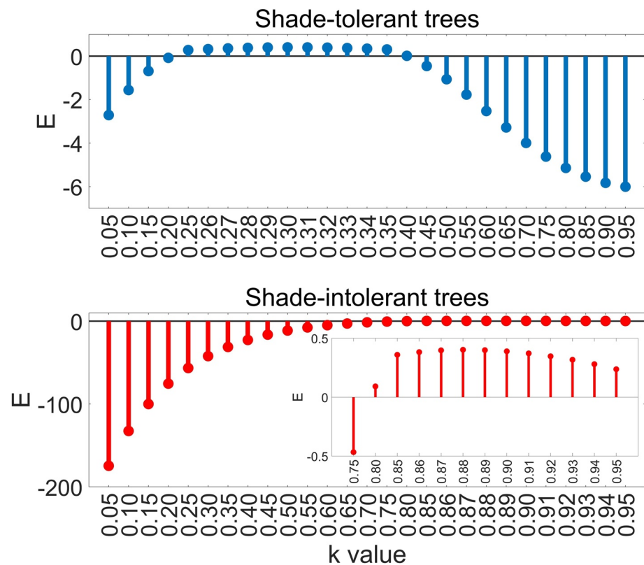
Figure 6. The model efficiency ( E ) of measured versus predicted aboveground wood increment of the shade-tolerant trees and shade-intolerant trees in all plots of Harvard Forest. These results are based on 27 different values of the critical allocate parameter ( k ).
