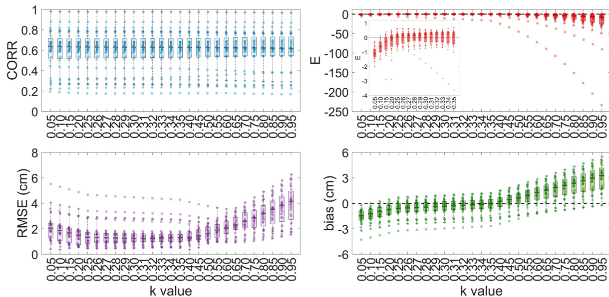
Figure 3. The statistical results of measured versus predicted ΔDBH of the shade-tolerant trees in the 32 plots of Harvard Forest. Each box has 32 data and each point represents 1 data. These results are based on 27 different values of the annually allocate parameter ( k ). The results include four time periods of ΔDBH: 2000–2005, 2000–2010, 2000–2015, and 2000–2020. CORR: correlation coefficient (i.e., r ); E: model efficiency; RMSE: root mean square error.
