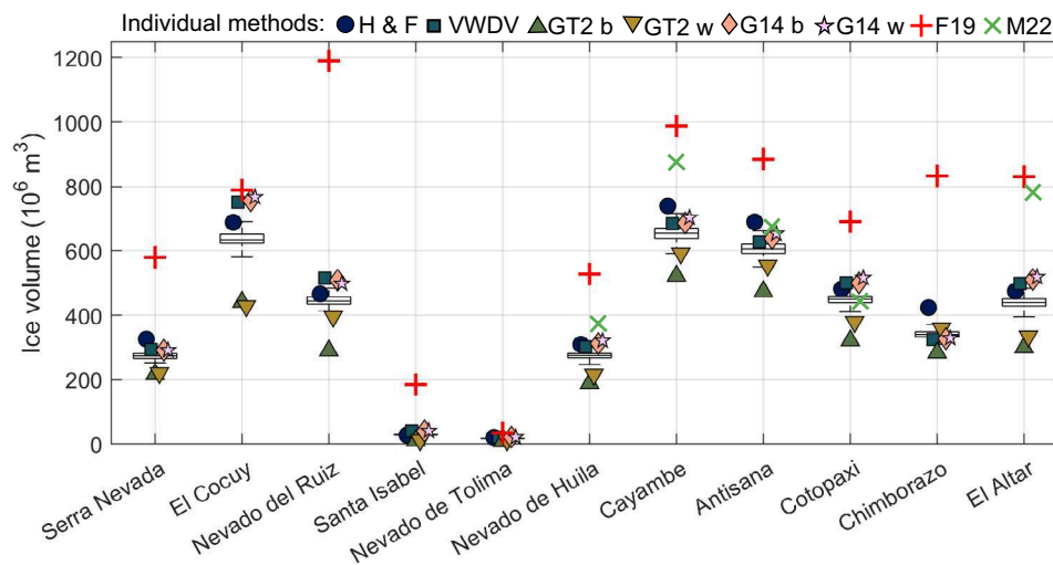
Fig. 5 Box plot showing the volume of all glaciers in Ecuador and Colombia. Boxes and error bars represent 1 standard deviation and the 95% confidence interval of the multi-model ensemble mean. Individual symbols represent mean volume estimates for each glacier from the six methods applied in this study and Farinotti et al. 35 . H F = mass-conservation-based approach 29,30 ; VWDV = fully distributed velocity-based inversion from this study; GT2 b = basal-shear-stress-based basin-divided approach 31,34 ; GT2 w = basal-shear-stress-based whole glacier approach 31,34 ; G14 b = Gantayat et al. 32 basin-divided approach 32 ; G14 w = Gantayat et al. 32 whole glacier approach 32 ; F19 = Farinotti et al. 35 volumes 35 ; M22 = Millan et al. 37 volumes 37 .
