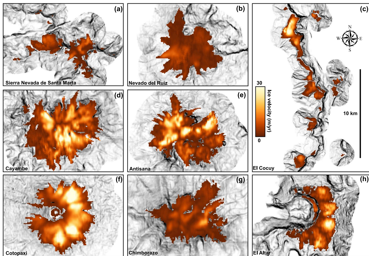
Fig. 2 Mean ice velocities of select glaciers in the Northern Andes. (a–c) Colombian glaciers. (d–h) Ecuadorian glaciers.
