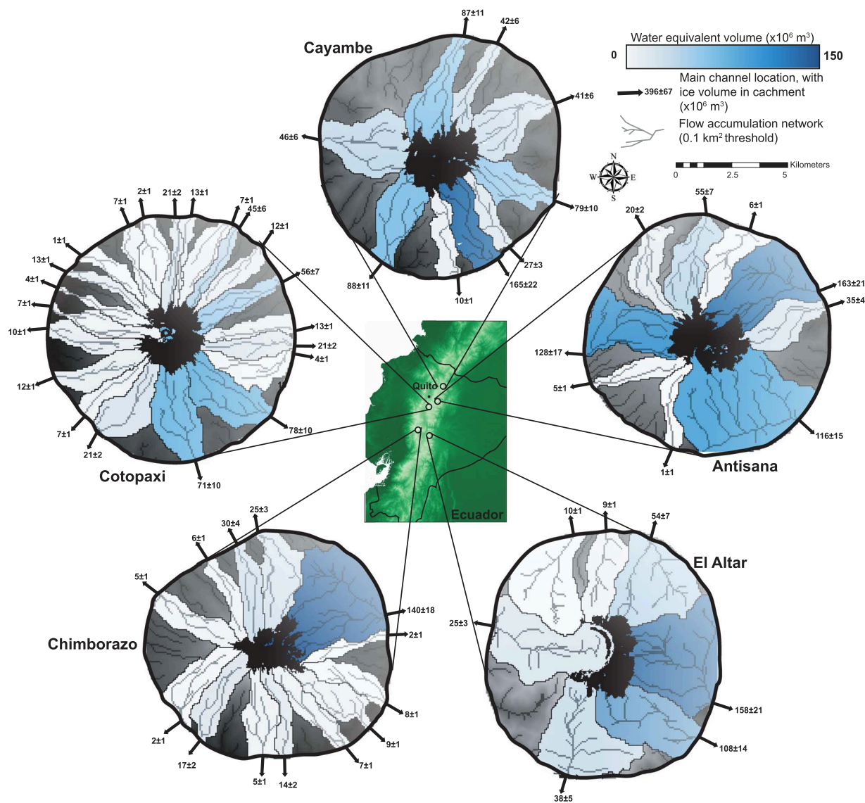
Fig. 7 Water-equivalent volumes within different catchments draining the five remaining Ecuadorian glaciers. An ice density range of 830 to 917 kg/m 3 (mean of 873.5 kg/m 3 ) was used to convert ice volumes to water-equivalent volumes 23,40,62 .
