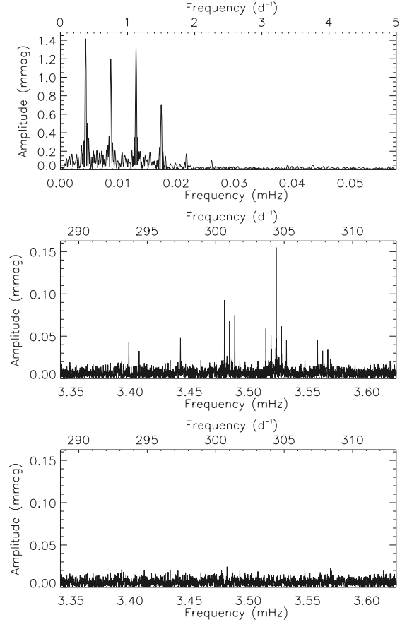
Figure 7. Top: amplitude spectrum at low frequency showing the rotation signal of TIC 350146296 and its harmonics. Middle: zoom of the pulsation modes found in this star. Bottom: the amplitude spectrum of the residuals after removing the frequencies shown in Table 6 showing no remaining significant signals.
