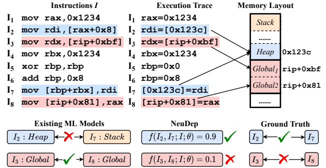
Figure 2: Motivating example of predicting memory dependencies in the function ngx_init_setproctitle from nginx-1.21.1 . I_2 and I_7 access the same heap variable (in blue); I_3 and I_8 access different global variables (in red). We find that existing ML-based approaches (learned on static code only) fail to detect I_2 and I_7 are dependent by predicting they access to different memory regions and cannot distinguish the memory accessed by I_3 and I_8 due to the prediction granularity.
