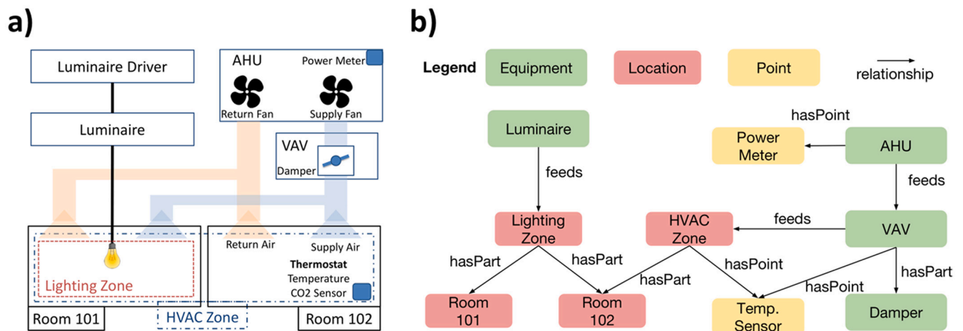
Fig. 2. Example of a Brick model: a) Example building, b) Example building modeled in Brick (visualized) [34].
