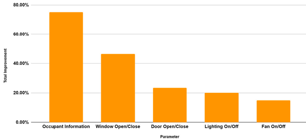
Fig. 6. Most improved occupant-related parameters using the extended Brick schema.
