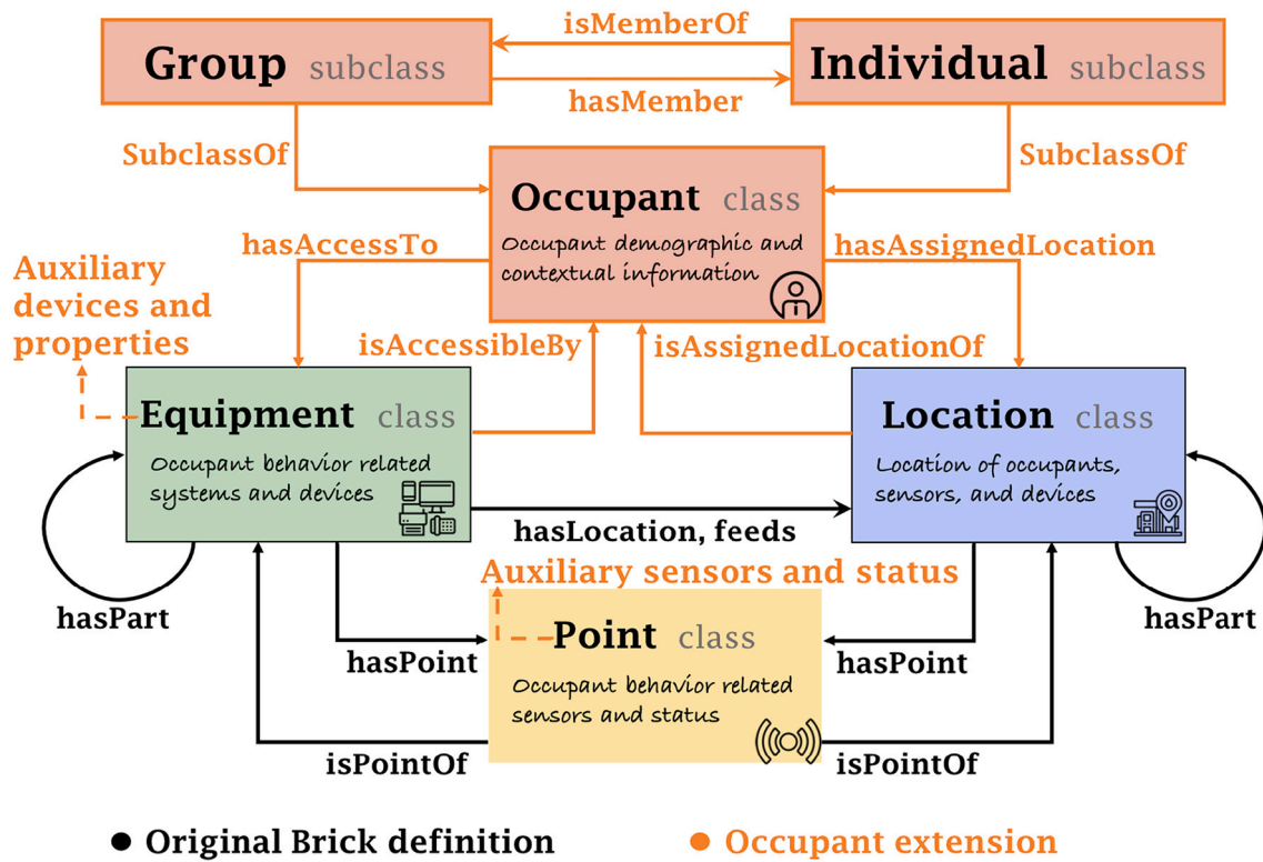
Fig. 4. Illustration of the Brick extension
