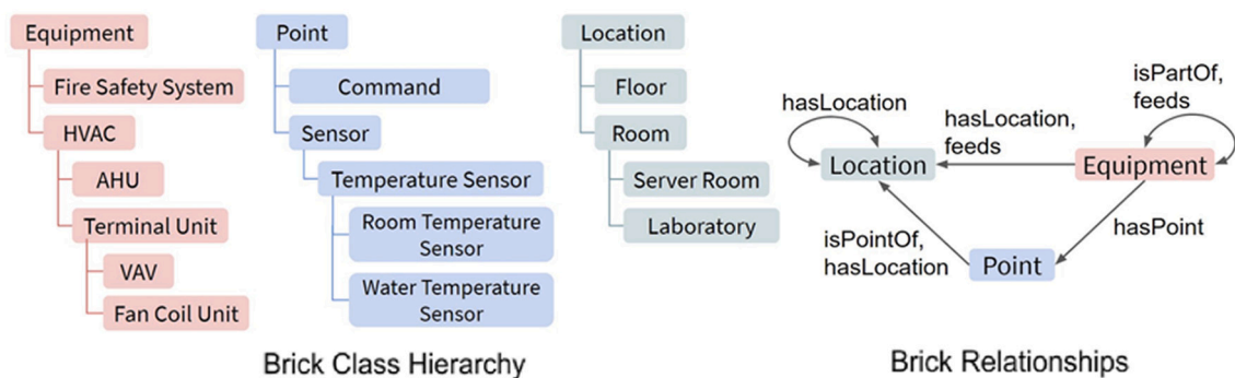
Fig. 3. Brick class hierarchy and relationships.
