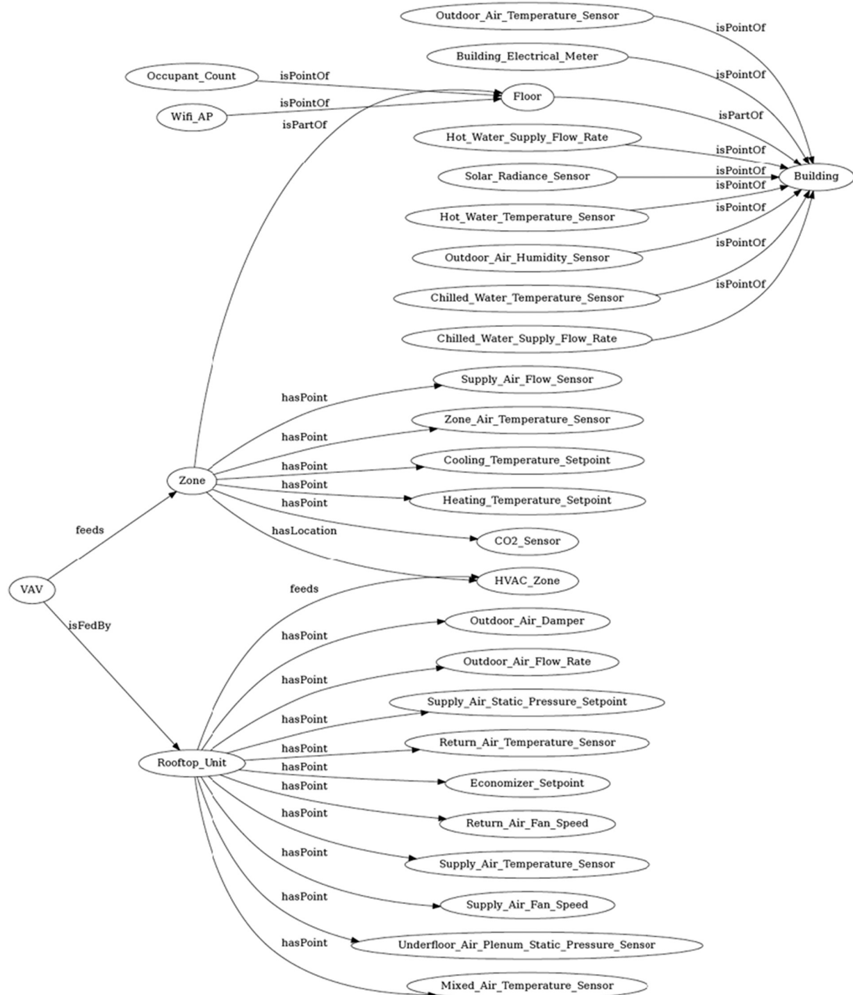
Fig. 9. Class graph of the Brick model for the Building 59 dataset. The diagram shows how instances of Brick classes (represented by nodes) relate to one another.
