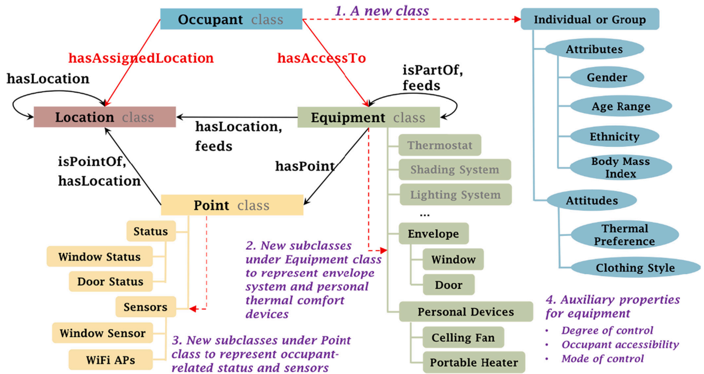
Fig. 5. Illustration of the Brick extension.
