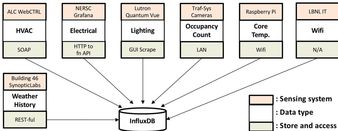
Fig. 8. Data measurements and collection systems.
