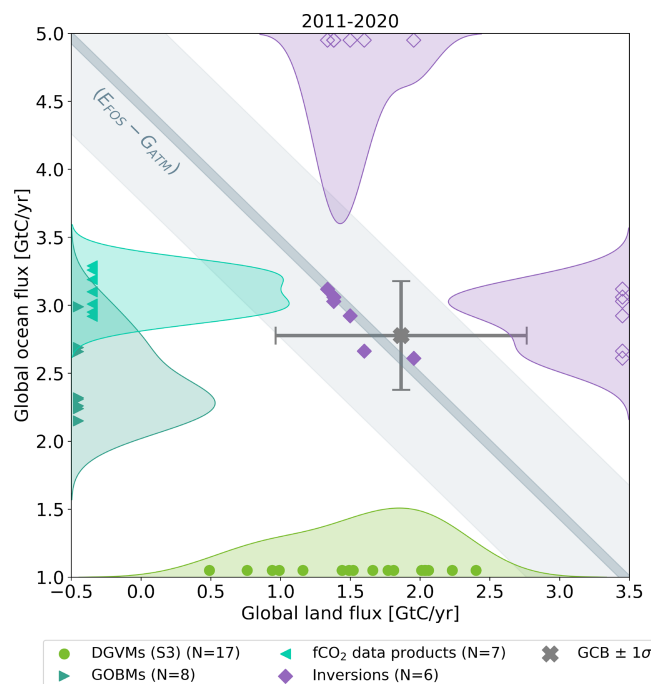
Figure 11. The 2011–2020 decadal mean net atmosphere–ocean and atmosphere–land fluxes derived from the ocean models and f\text{CO}_2 data products (y axis, right- and left-pointing blue triangles respectively) and from the DGVMs (x axis, green symbols), and the same fluxes estimated from the six inversions (purple symbols on secondary x and y axis). The grey central point is the mean ( \pm 1\sigma ) of S_{\text{OCEAN}} and ( S_{\text{LAND}} - E_{\text{LUC}} ) as assessed in this budget. The shaded distributions show the density of the ensemble of individual estimates. The grey diagonal band represents the fossil fuel emissions minus the atmospheric growth rate from this budget ( E_{\text{FOS}} - G_{\text{ATM}} ). Note that positive values are \text{CO}_2 sinks.
