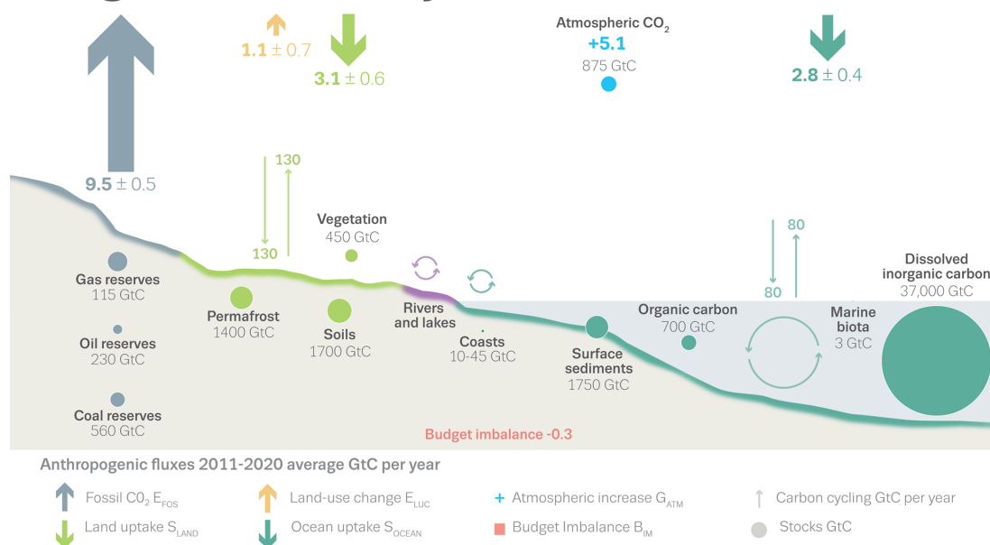
Figure 2. Schematic representation of the overall perturbation of the global carbon cycle caused by anthropogenic activities, averaged globally for the decade 2011–2020. See legends for the corresponding arrows and units. The uncertainty in the atmospheric CO 2 growth rate is very small ( \pm 0.02 GtC yr -1 ) and is neglected for the figure. The anthropogenic perturbation occurs on top of an active carbon cycle, with fluxes and stocks represented in the background and taken from Canadell et al. (2022) for all numbers, except for the carbon stocks in coasts which is from a literature review of coastal marine sediments (Price and Warren, 2016).
