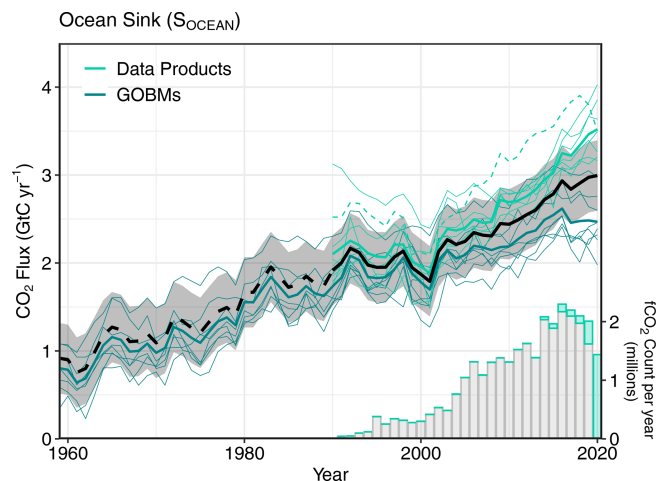
Figure 9. Comparison of the anthropogenic atmosphere–ocean CO 2 flux showing the budget values of S_{\text{OCEAN}} (black; with the uncertainty in grey shading), individual ocean models (teal), and the ocean f\text{CO}_2 -based data products (cyan; with Watson et al. (2020) in dashed line as not used for ensemble mean). The f\text{CO}_2 -based data products were adjusted for the pre-industrial ocean source of CO 2 from river input to the ocean, by subtracting a source of 0.61 GtC yr -1 to make them comparable to S_{\text{OCEAN}} (see Sect. 2.4). Bar-plot in the lower right illustrates the number of f\text{CO}_2 observations in the SOCAT v2021 database (Bakker et al., 2021). Grey bars indicate the number of data points in SOCAT v2020, and coloured bars the newly added observations in v2021.
