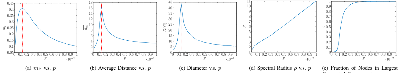
Figure 1: Robustness Measures v.s. p in G(n, p) ; n = 1,000 and dashed line shows the turning point at p = 0.0013 .
