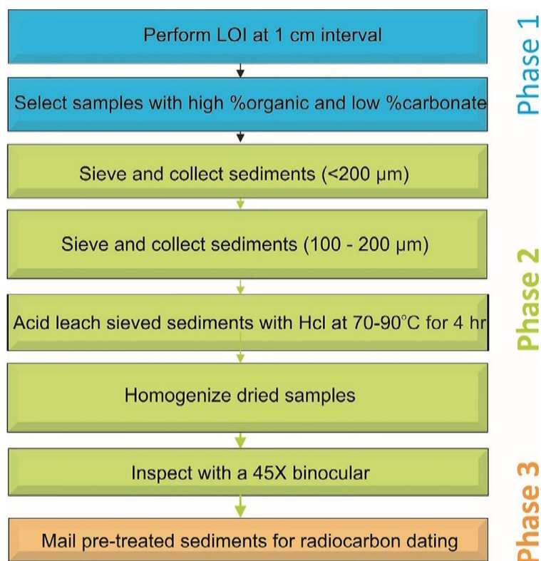
Fig. 2. Methodology flow-chart
