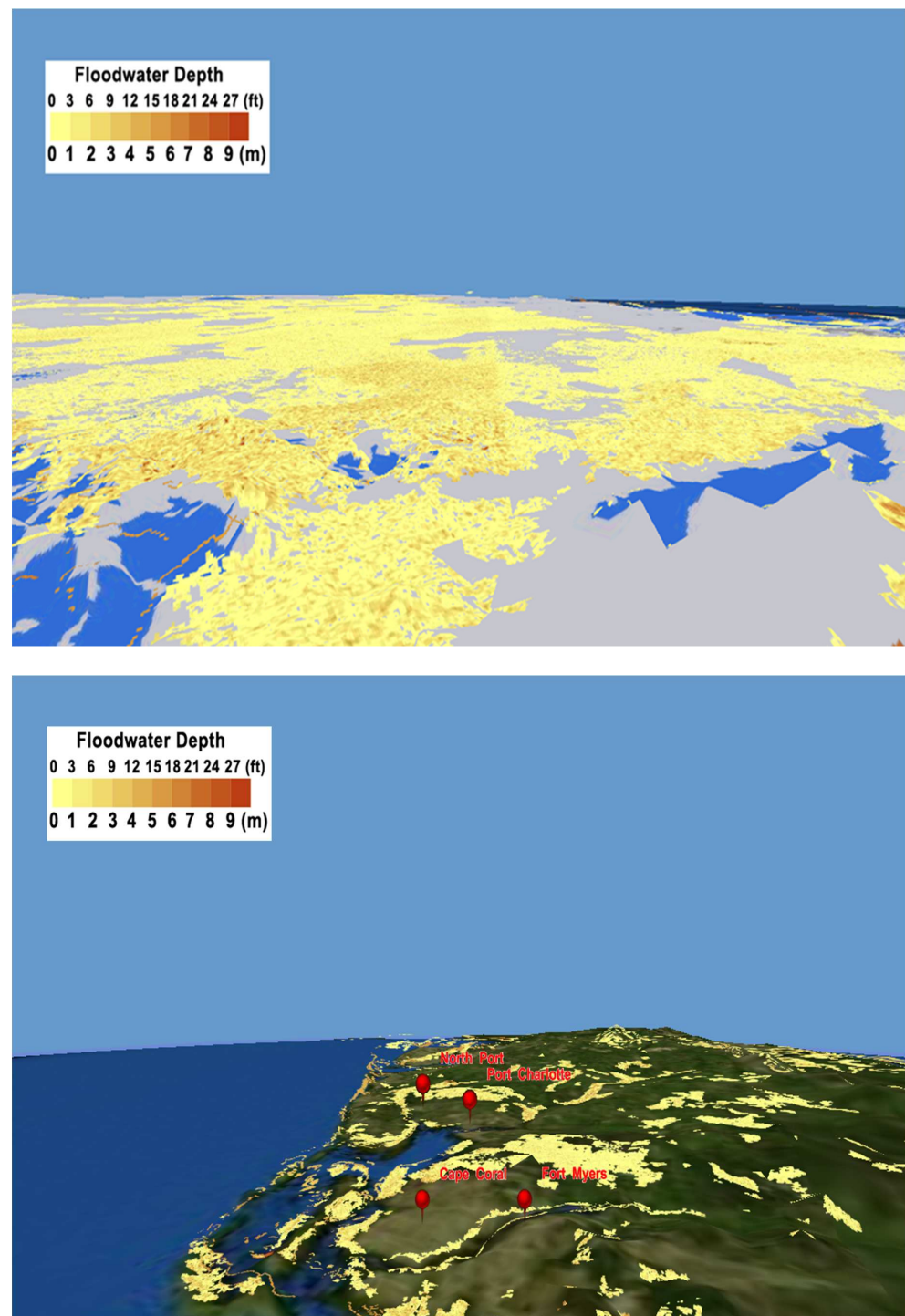
Figure 3. The 3D visualization of the VIIRS downscaled 30 m floodwater depths in southern Florida ( Upper ) and southwest Florida ( Lower ) on 30 September 2022 by using the ArcGlobe.
