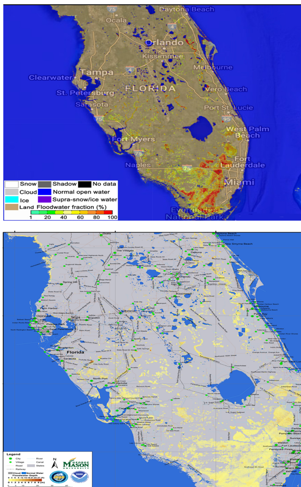
Figure 2. VIIRS flood map at the original 375 m resolution ( upper ) and the downscaled 30 m floodwater depths ( lower ) in Florida due to Hurricane Ian on 30 September 2022.
