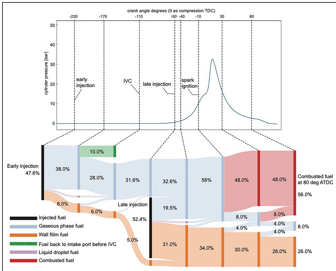
Figure 12. Sankey graph of the cold start fuel in cylinder 3 using the baseline 2-injection strategy, based on the simulations.
