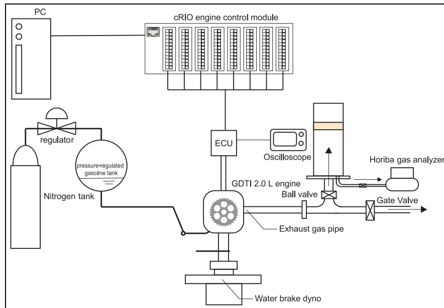
Figure 1. Experimental schematic.
