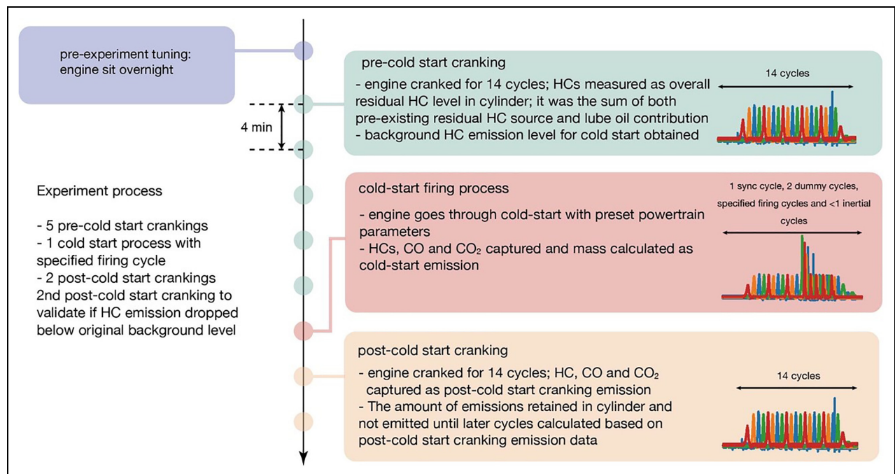
Figure 2. Experimental process.
