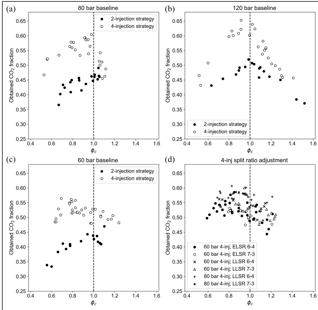
Figure 5. CO 2 carbon mass fraction with change of calculated combustive equivalence ratio.
