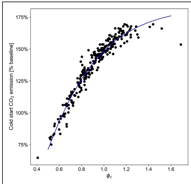
Figure 7. Cold start emitted CO 2 with change of combustive equivalence ratio.
