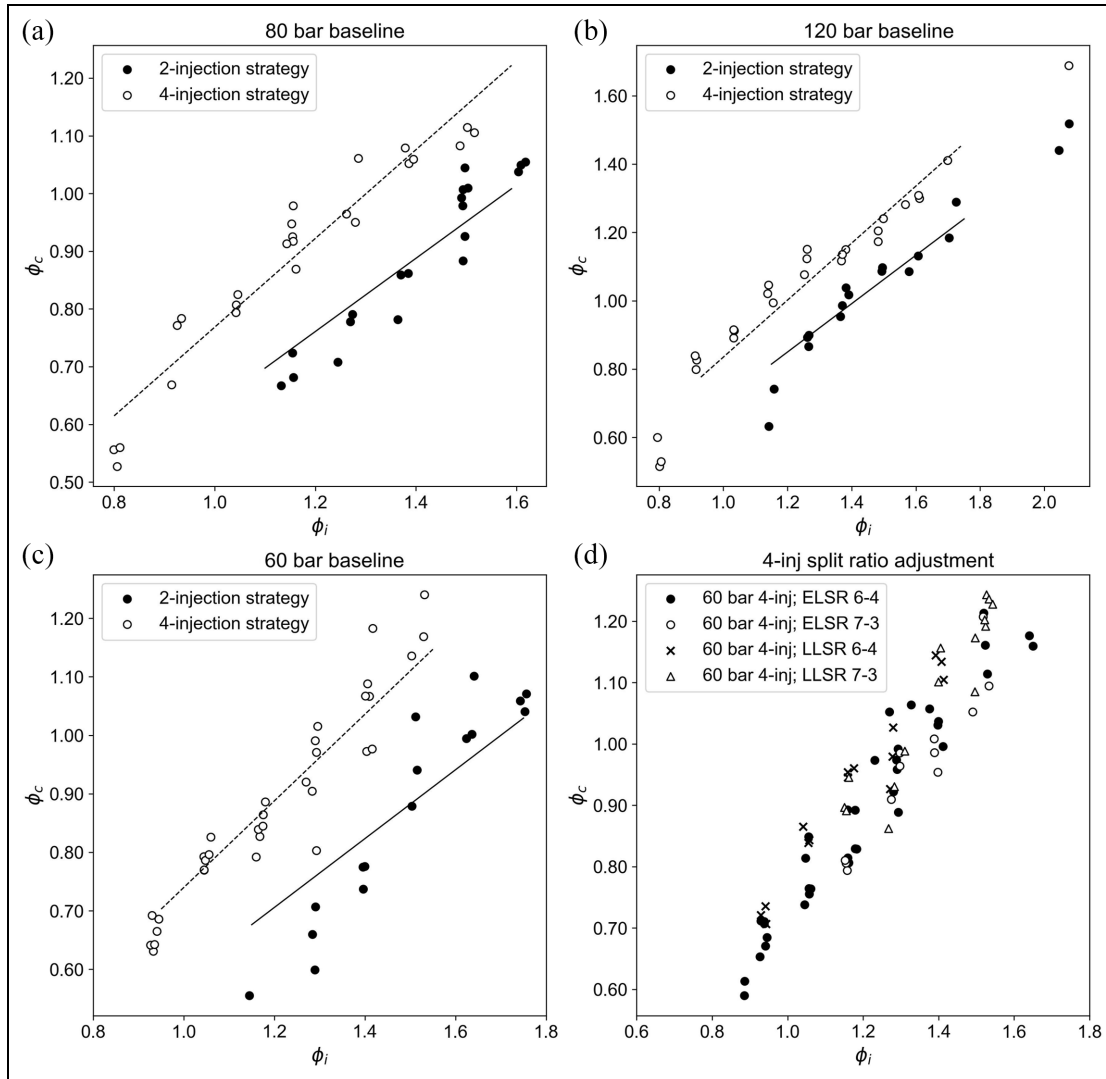
Figure 8. Combusted equivalence ratio change with injected equivalence ratio.
