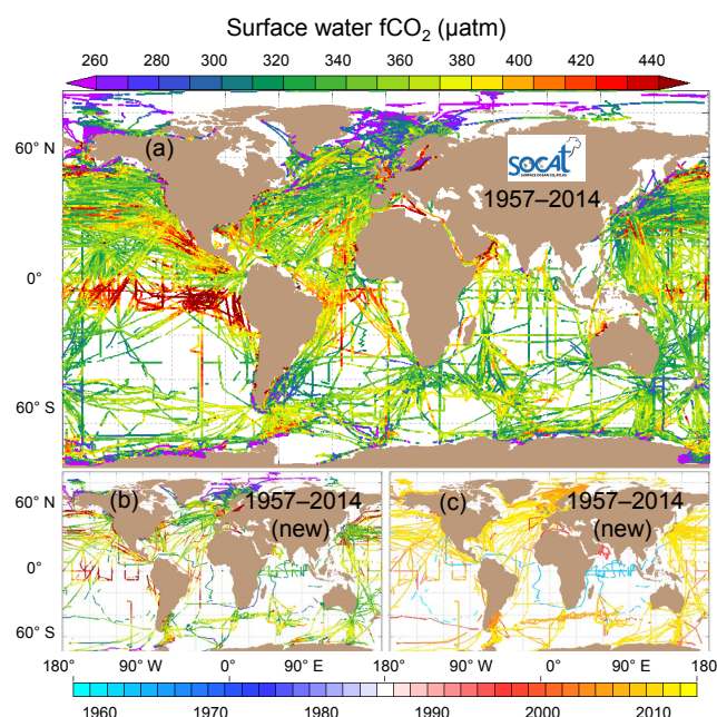
Figure 1. Global distribution of (a) all and (b) newly added surface water f\text{CO}_2 values (µatm) and (c) the timing of the newly added data sets in SOCAT version 3 with data set flags of A to E. Version 3 has data sets from 1957 to 2014.
