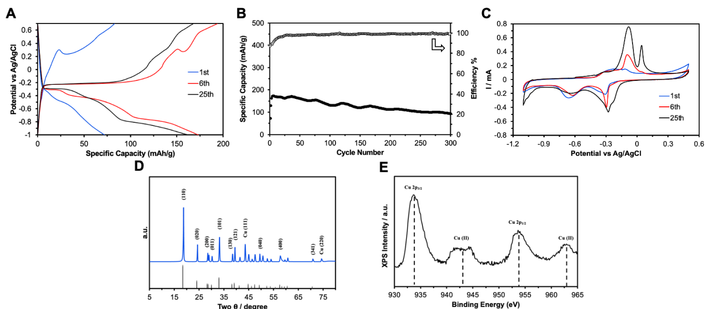
Figure 1. Electrochemical performance of Cu in 16 m KF. (A) GCD potential profiles for the 1 st , 6 th , and 25 th cycle at 500 mA/g. (B) Cycling performance. (C) CV results for the 1 st , 6 th , and 25 th cycle at 1 mV/s. (D) Ex situ XRD pattern of the charged electrode. (E) XPS spectrum of the charged electrode.
