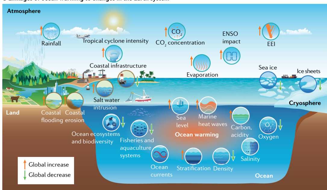
Fig. 1 | The role of ocean warming in the climate system. a | Principal processes and feedback loops (Fx) between ocean warming and physical and biogeochemical processes of the Earth system. The between Earth system components indicates cycle and/or system coupling. b | Schematic representation of the linkage between ocean warming and multiple observed changes in the Earth system. Orange upward arrows indicate a global increase in the particular process, and green downward arrows a global decrease. Ocean warming is a key component of the Earth system, bridging key climate cycles and driving changes in Earth system processes and components.
