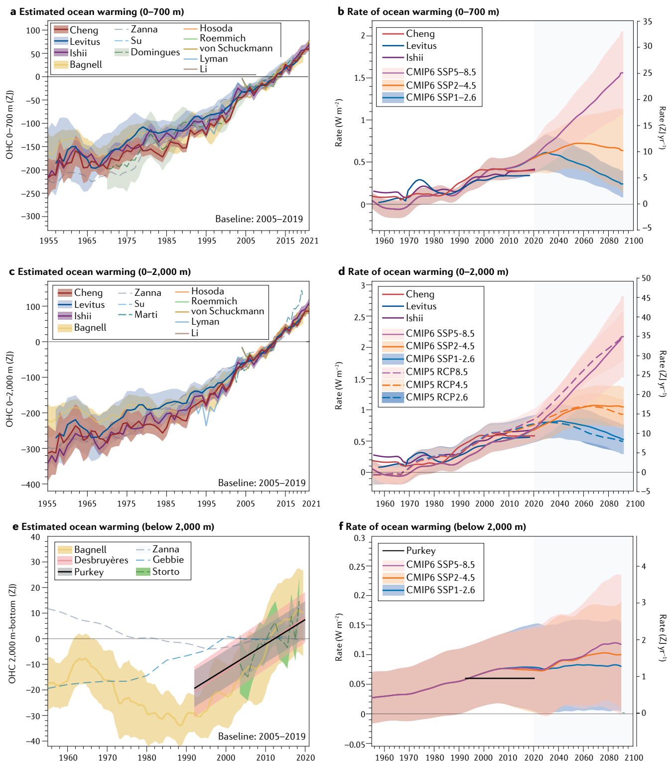
Fig. 2 | Observed and projected ocean heat content changes. a | Observed change in global annual 0–700-m ocean heat content (OHC) from 1955 to 2021, using various time series (listed by first author) 36,51,54,55,58,59,61–64,68,269 ; Zanna represents the average of three estimates using different sea surface temperature datasets. Solid and dashed lines represent direct and indirect estimates, respectively, and shading indicates the 90% confidence intervals ( \pm 1.6\sigma ). OHC anomalies are relative to a 2005–2019 baseline. b | Select observed (1955–2021) and modelled (1955–2100) rates of 0–700-m OHC change. Model time series are from CMIP6 and CMIP5 (for 0–2,000 m only),
