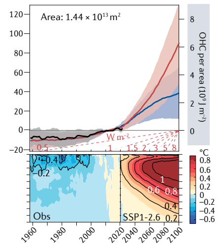
h Arctic Ocean OHC ( 65^\circ\text{N} to 90^\circ\text{N} )
