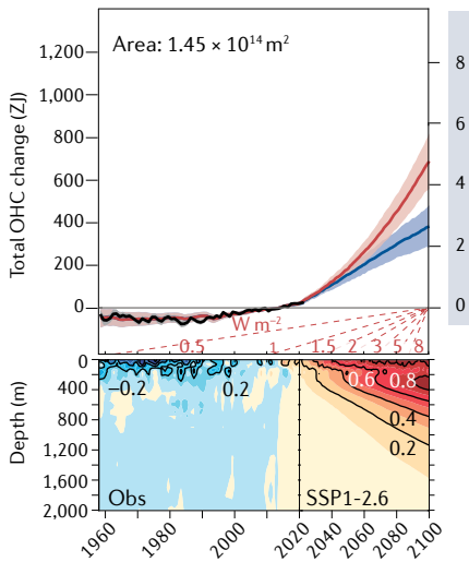
f Southern oceans OHC ( 78^\circ\text{S} to 35^\circ\text{S} )
