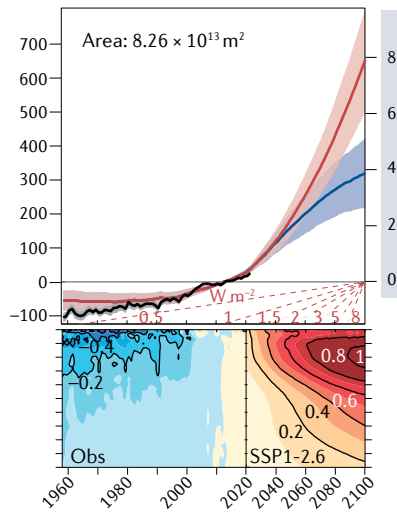
g Mediterranean Sea OHC
