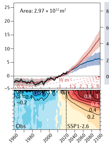
g Mediterranean Sea OHC
