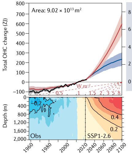
f Southern oceans OHC ( 78^\circ\text{S} to 35^\circ\text{S} )
