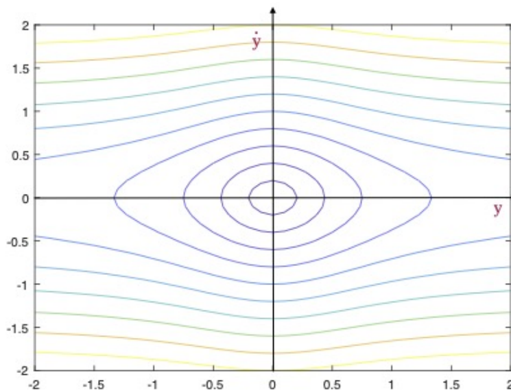
Figure 2: The level sets where the energy E(y, \dot{y}) at (5.13) is constant.
