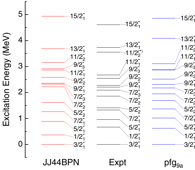
FIG. 7. Comparison of the experimental level energies of negative parity states in ^{63}\text{Cu} with those calculated using the jj44bnpn and the pf g_{9a} interactions in the shell model framework.
