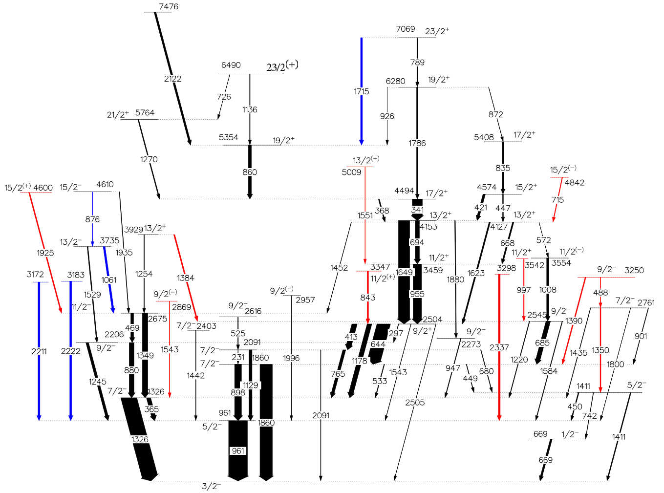
FIG. 3. Level scheme of ^{63}\text{Cu} , as resulting from the present work. The new transitions observed herein are marked in red. The previously known ones are from the work of Rai et al. [14]. The transitions represented by blue lines are tentative ones and weakly observed in the present study. Of these, the 876- and the 1715-keV were reported by Rai et al. [14] while the 1061, 2211, and 2222-keV are being newly proposed following the current investigation. The width of an arrow represents the intensity of the respective transition.
