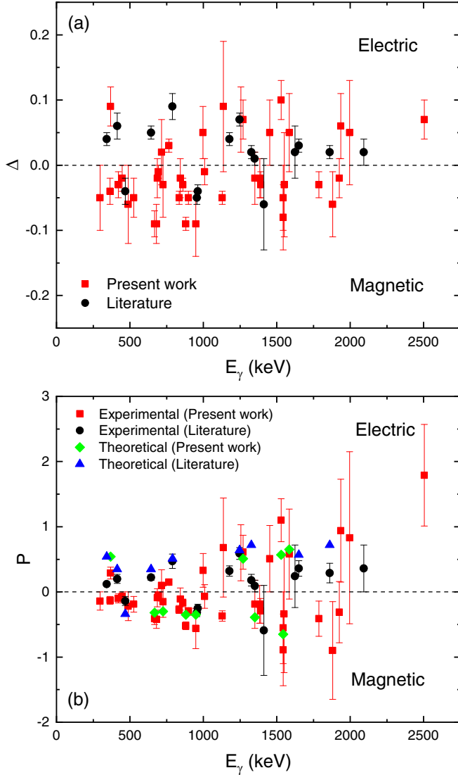
FIG. 2. (a) Polarization asymmetry ( \Delta ) and (b) experimental and theoretical polarization ( P ) values, for different transitions of ^{63}\text{Cu} as observed in the present experiment. The theoretical polarization has been calculated for the pure stretched transitions only. The transitions for which electric and magnetic nature have been identified newly in this work are marked accordingly (“Present work”) in the two figures. The electric and magnetic character of the other (“Literature”) transitions were previously known and have been confirmed in the present work. Not all the previously known transitions have been included in these plots. All the \Delta and P values, however, are recorded in Table I.
