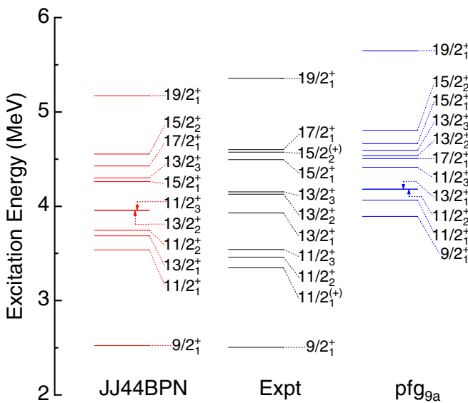
FIG. 8. Comparison of the experimental level energies of positive parity states in ^{63}\text{Cu} with those calculated using the jj44bnpn and the pf g_{9a} interactions in the shell model framework.
