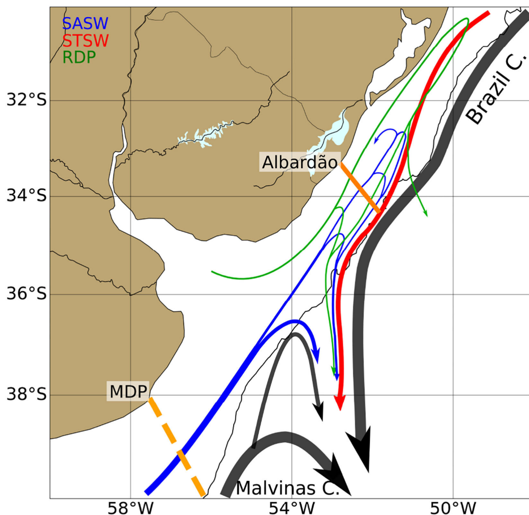
FIGURE 1 | Schematic circulation diagram of the Southwest Atlantic Shelf between 30 and 40°S. The Mar del Plata (MDP) and Albardão transects are indicated by an orange dashed and solid line, respectively. The gray line indicates the 200 m isobath. SASW, Subantarctic Shelf Water (blue); STSW, Subtropical Shelf Water (red); RDP, Río de la Plata water (green). Adapted from Berden et al. (2020) with permission.
