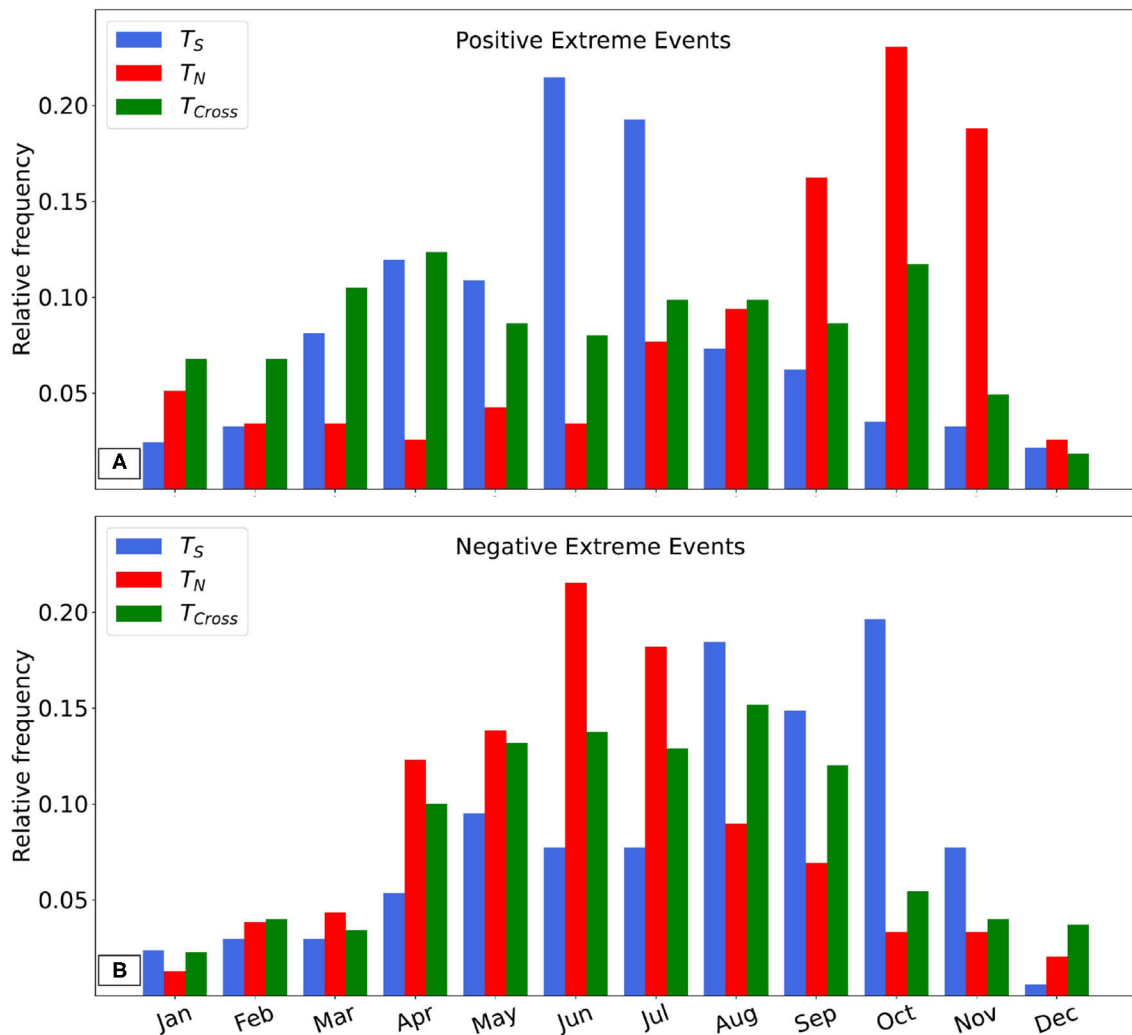
FIGURE 9 | Histogram of monthly binned extreme transport events through 40°S ( T_S , blue), 30°S ( T_N , red), and cross-shore ( T_{Cross} , green). (A) Positive extreme events. (B) Negative extreme events.
