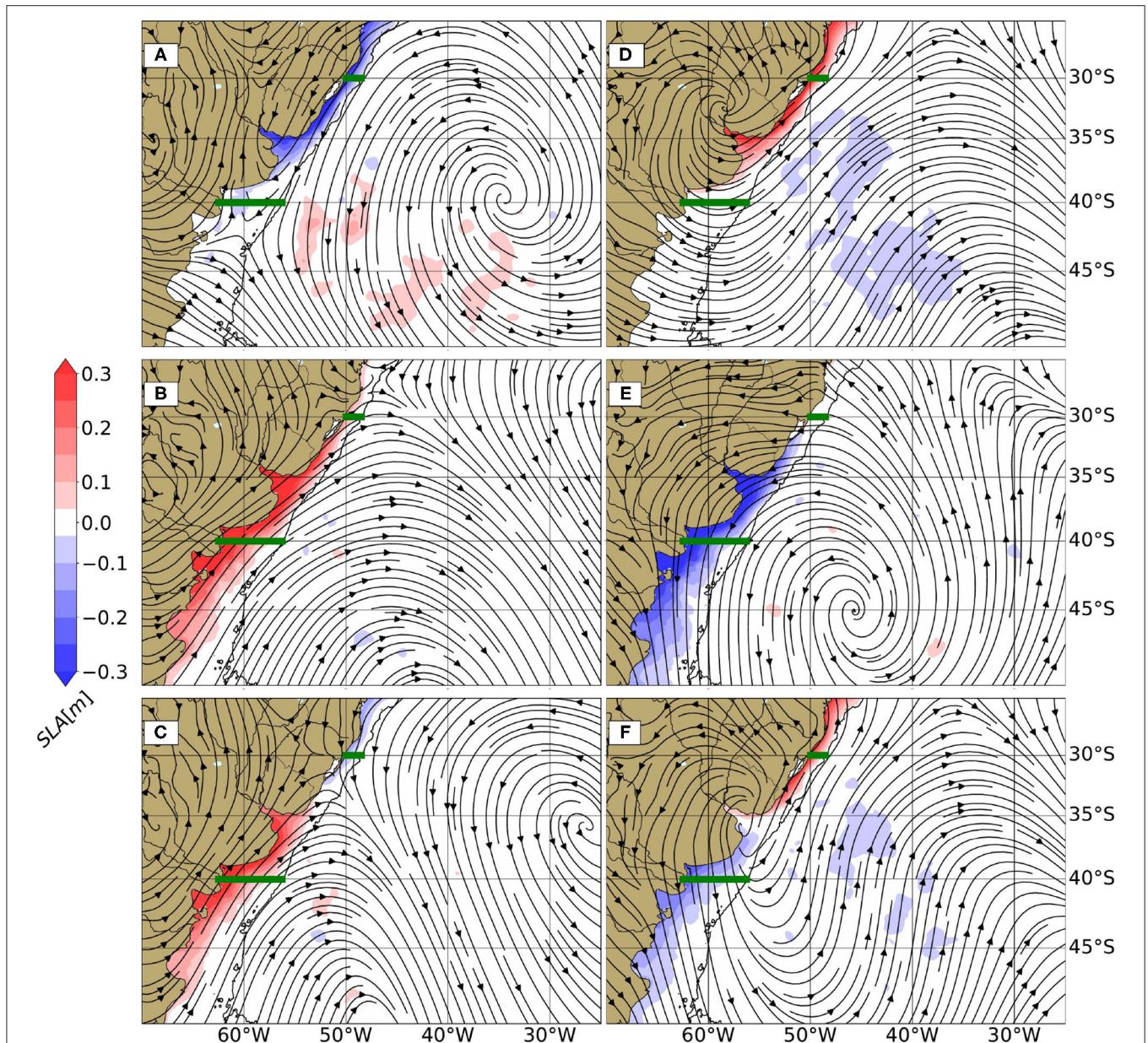
FIGURE 10 | Composite of model derived sea level anomaly (background color shading) and black streamlines show surface wind patterns during positive (A) and negative (D) extreme T_N events. (B) and (E), same as (A,D) for T_S . (C) and (F), same as (A,D) for T_{Cross} . The 200 m isobath is indicated by a gray line.
