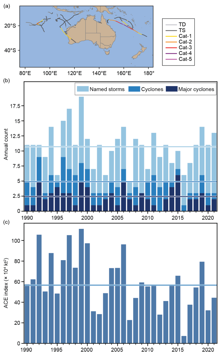
Fig. 4.38. Annual TC statistics for the Australian basin for 1990–2021: (a) storm tracks for 2021, (b) number of named storms, cyclones, and major cyclones, and (c) ACE ( \times 10^4 \text{ kt}^2 ). The 1991–2020 means (horizontal lines) are included in both (b) and (c). Classifications are based on the SSHWS.
