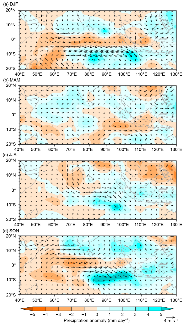
Fig. 4.20. Precipitation (mm day -1 ) and surface wind (m s -1 ) anomalies relative to 1991–2020 during (a) Dec 2020–Feb 2021, (b) Mar–May 2021, (c) Jun–Aug 2021, and (d) Sep–Nov 2021. (Sources: monthly GPCP precipitation analysis [ https://psl.noaa.gov/data/gridded/data.gpcp.html ] and JRA-55 atmospheric reanalysis [Ebita et al. 2011].)
