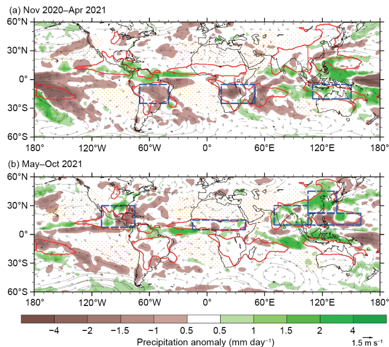
Fig. 4.15. Seasonal mean precipitation anomalies (mm day -1 ) and 850-hPa wind anomalies (m s -1 ) for (a) the SH summer monsoon season: Nov 2020–Apr 2021 and (b) the NH summer monsoon season: May–Oct 2021. Climatological mean was made for 1991–2020. Red lines outline the monsoon precipitation domain defined in the text. The dotted area represents the dry region where the local summer precipitation rate is below 1 mm day -1 . Rainfall data were taken from the Global Precipitation Climatology Project (GPCP; Huffman et al. 2009).
