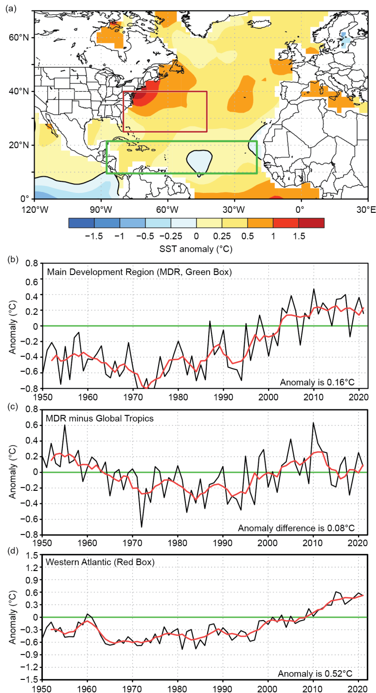
Fig. 4.24. (a) Aug–Oct 2021 SST anomalies (°C). (b–d) Time series of Aug–Oct area-averaged SST anomalies (black) and 5-pt running mean of the time series (red); (b) In the MDR (green box in (a) spanning 20°–87.5°W and 9.5°–21.5°N); (c) difference between the MDR and the global tropics (20°S–20°N); and (d) in the western North Atlantic (red box in (a) spanning 42.5°–80°W and 25°–40°N). Anomalies are departures from the 1991–2020 period means. (Source: ERSST-v5 [Huang et al. 2017].)
