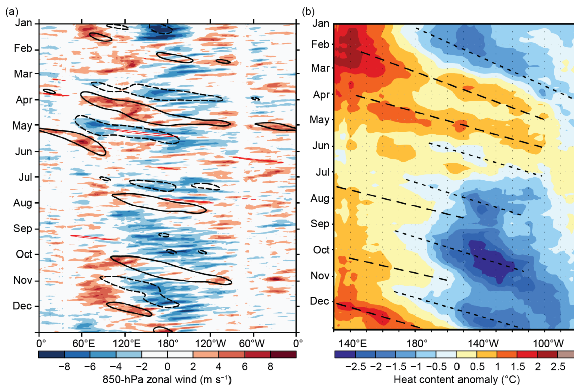
Fig. 4.9. (a) Time–longitude section for 2021 of anomalous 850-hPa zonal wind ( \text{m s}^{-1} ) averaged between 10^\circ\text{N} and 10^\circ\text{S} . Contours identify anomalies filtered for the MJO. (b) Time–longitude section for 2021 of anomalous equatorial Pacific Ocean heat content ( ^\circ\text{C} ), calculated as the mean temperature anomaly between 0 and 300-m depth. Yellow/red (blue) shading indicates above- (below-) average heat content. Relative warming (dashed lines) and cooling (dotted lines) due to downwelling and upwelling equatorial oceanic Kelvin waves are indicated. Anomalies are departures from the 1991–2020 base period pentad means. Data in (b) are derived from an analysis system that assimilates oceanic observations into an oceanic general circulation model (Behringer et al. 1998).
