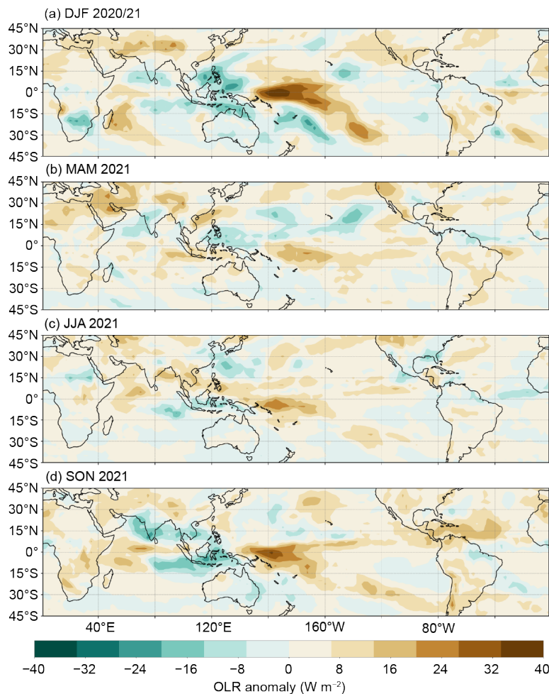
Fig. 4.6. Outgoing longwave radiation (OLR) anomalies (shaded, \text{W m}^{-2} ), during (a) DJF 2020/21, (b) MAM 2021, (c) JJA 2021, and (d) SON 2021. Anomalies are departures from the 1991–2020 period monthly means. Data are from the NCEP/NCAR Reanalysis (Kalnay et al. 1996).
