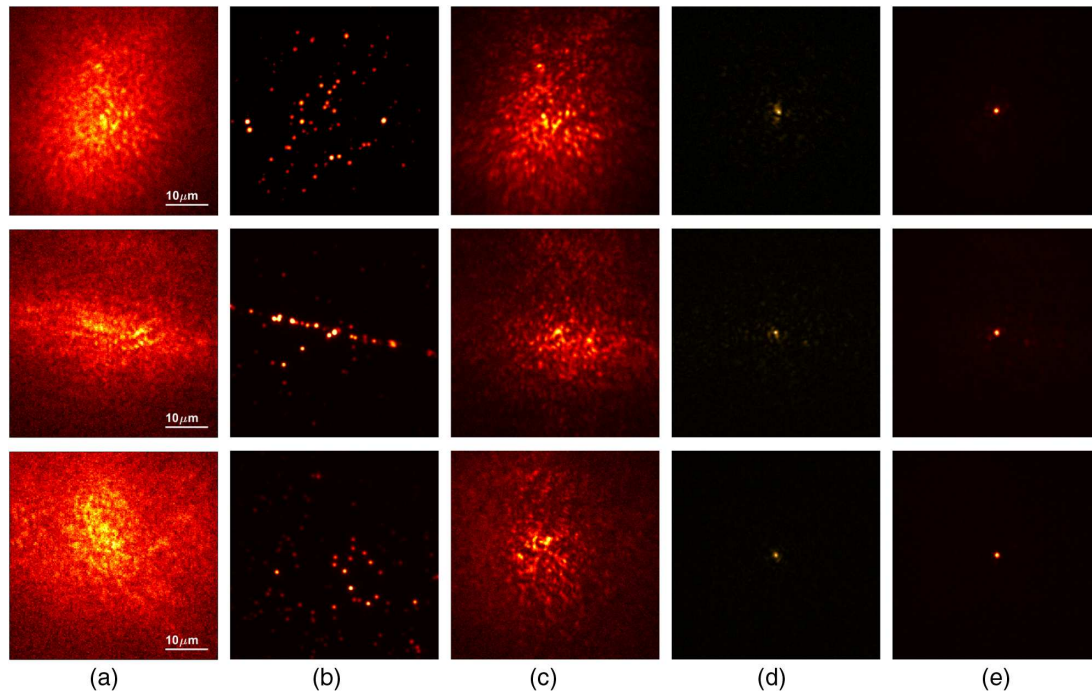
Fig. 4. Analyzing focusing inside a tissue: Each row visualizes a different experiment on a different tissue slice. (a) Main camera when SLMs are blank, demonstrating initial speckles. (b) Validation camera when illumination SLM is blank, demonstrating the enlightened bead layout at the emission wavelength. (c) Speckles from one bead (imaging SLM is blank and illumination SLM is corrected), demonstrating the amount of aberration. (d) Validation camera when illumination is corrected, demonstrating that most light gets into a single spot (excitation wavelength). (e) Main camera when both SLMs are corrected, demonstrating focusing in a single spot.
