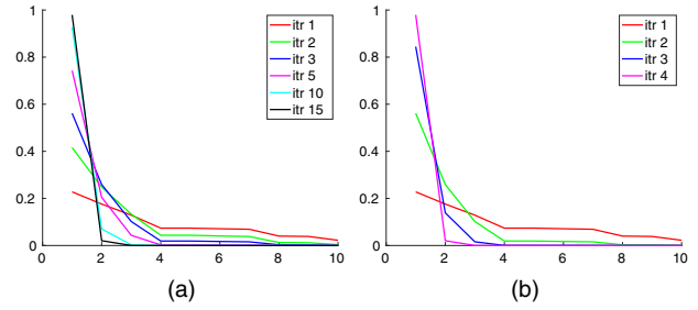
Fig. 2. Simulating coherent and incoherent convergence: We plot the power of scatterers |\mathbf{v}_k^{(t)}|^2 , for different iterations of the iterative phase conjugation algorithm. As predicted by theory, the incoherent case converges into a one-hot vector within a smaller number of iterations (compare four incoherent iterations to 15 coherent ones). The x axis of our plot corresponds to scatterer index k , where for ease of visualization we sort these in decreasing order of power.
