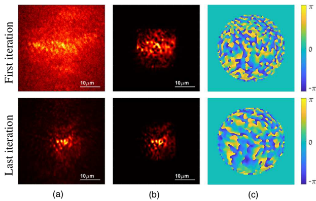
Fig. 5. Phase reconstruction: (a) Speckle image captured by the main camera in the first and last iteration of the algorithm. (b) Intensity of the recovered aberration correction in the sensor plane. In the first iteration, when multiple incoherent beads are excited, we cannot fully explain the image as a single coherent wavefront. However, as the algorithm converges to excite a single bead, the recovered wavefront better matches with the captured image. (c) Phase of the recovered aberration correction in the Fourier plane, which is the mask presented on the SLM.
