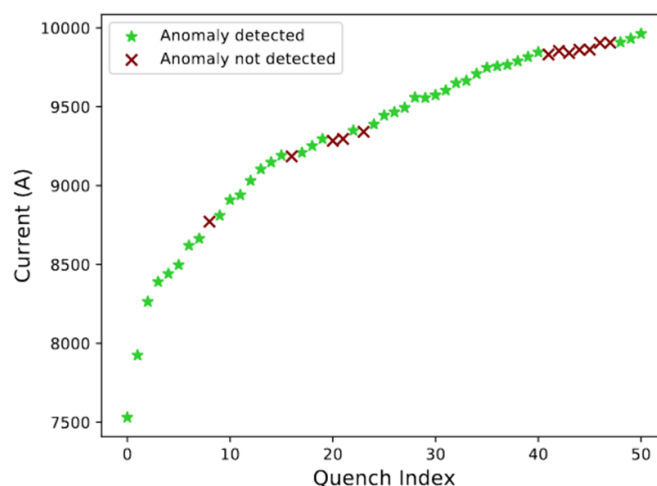
Figure 13. Anomaly events detected by a prototype machine learning algorithm in post-processing analysis of acoustic data taken during the training of MDPCT1b magnet. Anomalous events are detected in the majority (77%) of quenches. © [2021] IEEE. Reprinted, with permission, from [74].
