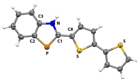
Fig. 1 X-ray crystal structure of compound 3c . Selected bond lengths (Å) and bond angles (°) of 3c : P=C 1 1.745(5), P–C 2 1.800(5), N–C 1 1.353(7), N–C 3 1.381(6), C 2 –C 3 1.395(7), C 1 –C 8 1.449(8), C 1 –P–C 2 88.8(2), N–C 1 –P 113.1(4), C 1 –N–C 3 114.8(4).
