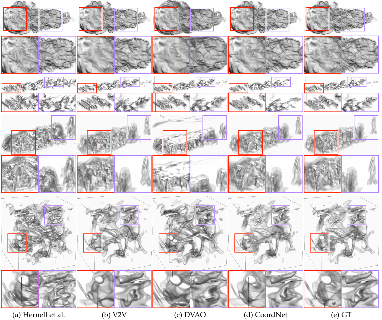
Fig. 12: Volume rendering results of LAO volumes for the AOP task. Top to bottom: argon bubble, half-cylinder (6400, VM), Tangaroa (VM), and vortex. The quantitative scores are displayed in Table 9.
