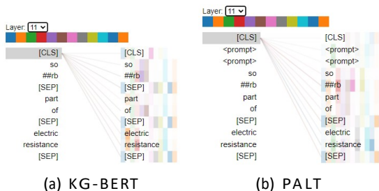
Figure 6: Comparison between the attention weights of PALT and KG-BERT. In this example, PALT correctly predicts it as negative and KG-BERT fails.
