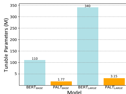
Figure 2: Compare the number of tunable parameters of PALT and BERT.
