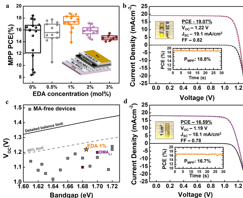
Figure 2. Photovoltaic device results. (a) Inset: Schematic of the perovskite solar cell device architecture we employ. Main: Efficiencies of solar cells made with 0–3 mol % EDA as an additive to the perovskite solution after 30 s of operation. (b) JV curves of the EDA-1 device under 1 sun simulated solar illumination, recorded in forward (from short to open circuit) and reverse (from open to short circuit) sweep directions. The inset tracks the PCE over 30 s of MPP-tracked device operation. Inset picture shows the device pixel area (0.25 cm 2 ). (c) Open-circuit voltage ( V OC ) results from the literature of wide-gap devices made with FA 1− x Cs x Pb(I 1− x Br x ) 3 compositions. The additives used in the best performing devices are noted next to the V OC values. Purple data are from ref 23 using DMA + . Brown points are from ref 36 using the same perovskite composition as this work (FA 0.83 Cs 0.17 Pb(I 0.75 Br 0.25 ) 3 ). All references used in part (c) are given in Table S2. (d) JV curves of the EDA-1 large area champion device under 1 sun simulated solar illumination, recorded in forward (from short to open circuit) and reverse (from open to short circuit) sweep directions. The inset tracks the PCE over 30 s of MPP-tracked device operation. Inset picture shows the device pixel area (1 cm 2 ).
