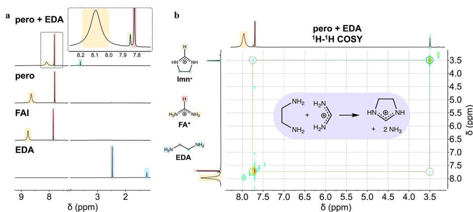
Figure 4. Chemical origins of EDA effects (a) ^1\text{H} solution NMR spectra of (bottom to top) ethylenediamine (EDA), formamidinium iodide (FAI), and (\text{FA}_{0.83}\text{Cs}_{0.17})\text{Pb}(\text{I}_{0.75}\text{Br}_{0.25})_3 without (pero) and with 10 mol % EDA added (pero + EDA). (b) ^1\text{H} – ^1\text{H} correlation spectroscopy (COSY) of (\text{FA}_{0.83}\text{Cs}_{0.17})\text{Pb}(\text{I}_{0.75}\text{Br}_{0.25})_3 with 10 mol % EDA added. Off-diagonal correlation indicates corresponding ^1\text{H} chemical environments are spin–spin coupled. All materials are dissolved in d_6 DMSO. The inset highlighted in purple shows the overall reaction of \text{FA}^+ with EDA to produce \text{Imn}^+ and ammonia.
