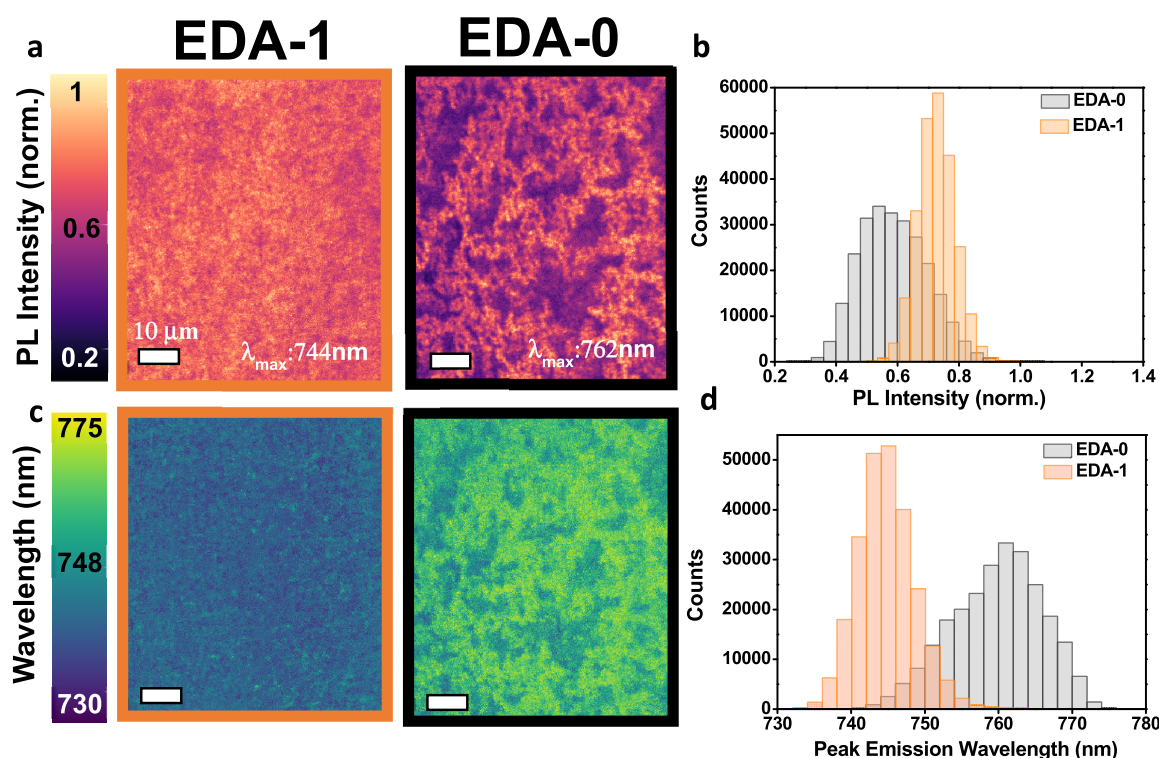
Figure 3. Halide heterogeneity on the microscale. (a) Hyperspectral PL intensity map of the EDA-0 (black box) and EDA-1 (orange box). PL images are shown at the maximum emission wavelength ( \lambda_{\text{max}} ) for each sample as stated on the figure (EDA-0 \lambda_{\text{max}} = 762 \text{ nm} , EDA-1 \lambda_{\text{max}} = 744 \text{ nm} ). Excitation was achieved with a white lamp with short pass filter at 500 nm. The emission was recorded using a 500 nm dichroic and 550 nm long pass filter. (b) Histogram of the PL intensity distribution at the maximum emission wavelength for EDA-0 (gray) and EDA-1 (orange) samples. (c) Peak emission wavelength map of the EDA-0 and EDA-1 films. (d) Histogram of the distribution of peak emission wavelengths for the EDA-0 (gray) and EDA-1 (orange) samples.
