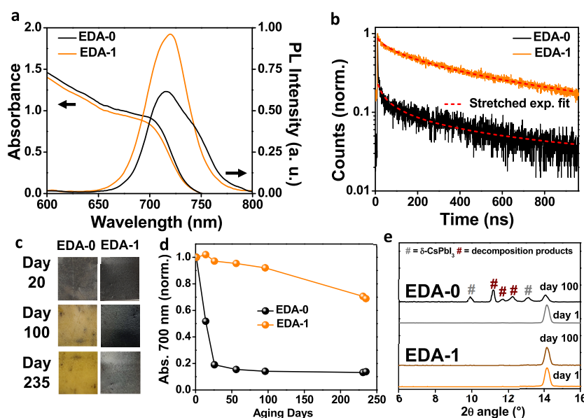
Figure 1. Material characterization and phase stability. (a) UV–vis spectra and normalized PL emission from films of \text{FA}_{0.83}\text{Cs}_{0.17}\text{Pb}(\text{I}_{0.75}\text{Br}_{0.25})_3 without EDA (EDA-0, black) and with 1% EDA (EDA-1, orange). The PL spectra are obtained using an integrating sphere coupled with a 532 nm laser. (b) Time resolved photoluminescence measurements using a 405 nm laser at 1 MHz pulse frequency. The fitting (dashed red line) was done using a stretched exponential decay. (c) Visual degradation of EDA-0 and EDA-1 exposed to air for 235 days. Samples were left unencapsulated in ambient air in the dark at an average room temperature of 19.5 °C and relative humidity of 31%. (d) Absorbance from UV–vis of EDA-0 (black) and EDA-1 (orange) at 700 nm during ambient aging. (e) XRD patterns in the 2\theta = 6\text{--}16^\circ region of the fresh EDA-0 (gray) and EDA-1 (orange) and after 100 days of ambient aging (EDA-0: black, EDA-1: brown).
