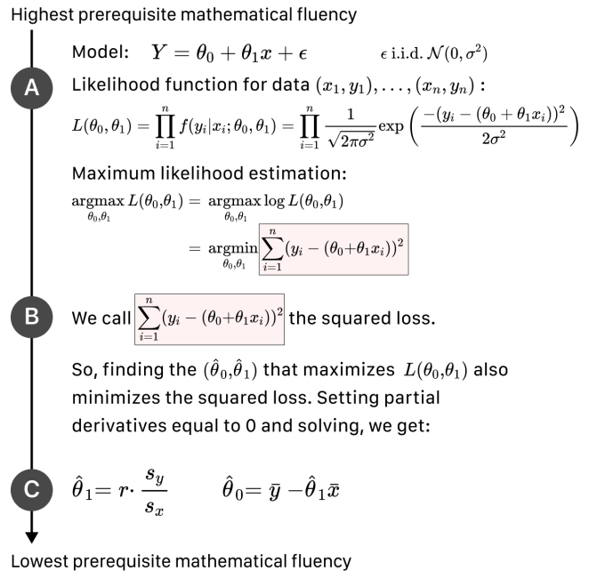
Figure 2: This sketch of a derivation for the simple linear model parameters highlights several possible pedagogical approaches. Instructors can start with (a) likelihood principle, (b) loss minimization, or (c) a closed-form solution.
