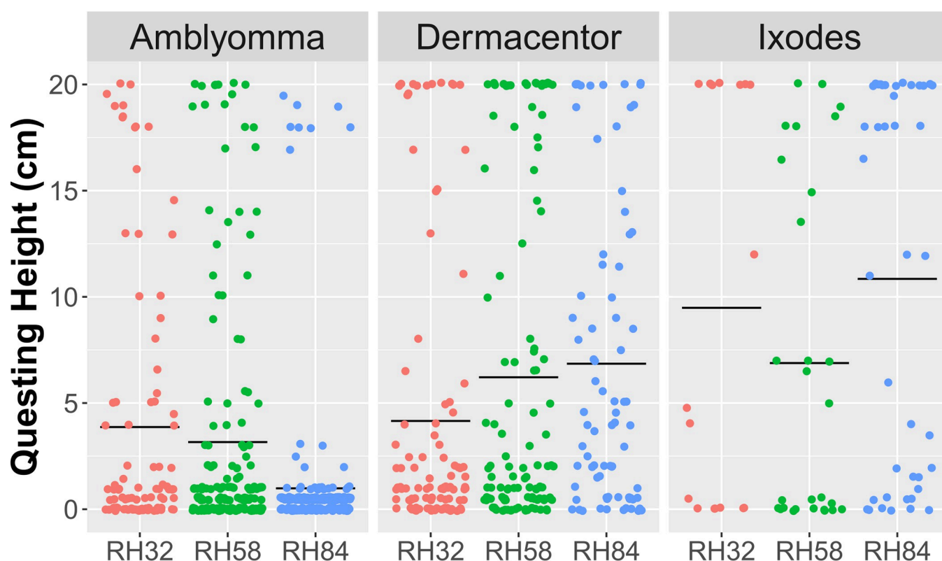
Fig 4. Questing heights of individual ticks in nine experimental groups. Each dot represents a single instance of tick questing; horizontal lines represent the average questing heights of each group. Questing height was negatively associated with RH in Amblyomma ( H = 24.765 , df = 2 , P < 0.001 ), positively associated with RH in Dermacentor ( H = 11.248 , df = 2 , P = 0.004 ), and not associated with RH in Ixodes ( H = 5.065 , df = 2 , P = 0.079 ).
