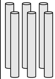
Fig 1. The experimental setup. Each cylinder represents a plastic tube containing one tick, and each rectangle represents an airtight container with a constant RH maintained by a humidity control pack. There were nine distinct groups based on species and RH. Each container with six ticks was replicated four times for a total sample of 24 ticks per group.
