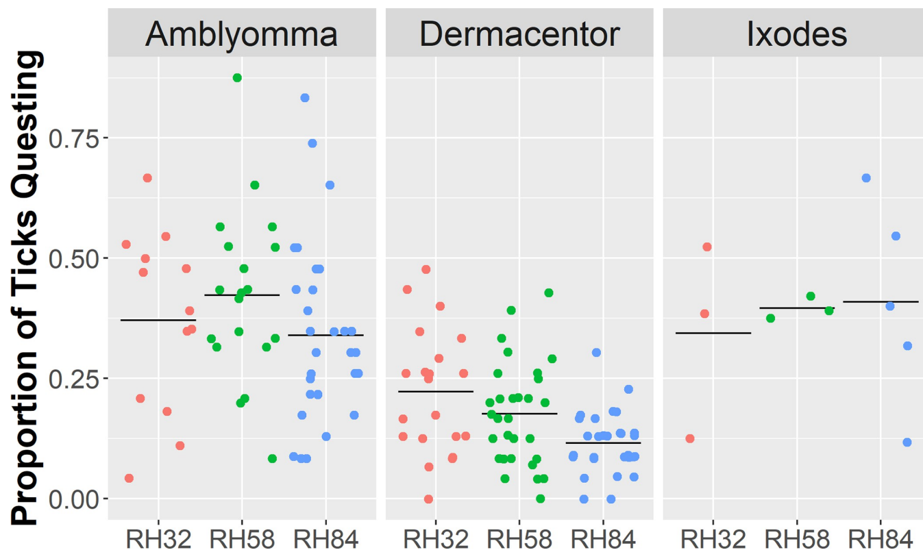
Fig 5. Questing frequencies in nine experimental groups. Each dot represents the proportion of ticks questing out of all living ticks within each experimental group on a particular day; the horizontal lines represent the average questing frequencies of each group. Questing frequency increased with drier conditions in Dermacentor ( H = 8.792 , df = 2 , P = 0.012 ), but not in Amblyomma ( H = 3.026 , df = 2 , P = 0.220 ) or Ixodes ( H = 0.194 , df = 2 , P = 0.908 ).
