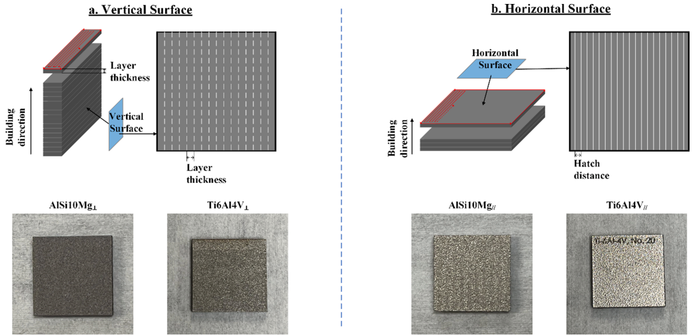
Fig. 2. Design of L-PBF experiments in this study: (a) vertical surface (surface parallel to the building direction) samples (b) horizontal surface (surface parallel to the building platform) samples.
