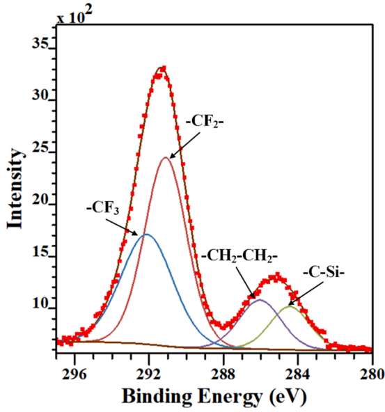
Fig. 10. Surface chemical functionalization characterized using core-level XPS analysis of C 1s at the aluminum alloy surface, showing the existence of \text{-CF}_2\text{-} , \text{-CF}_3 superhydrophobic functional groups.
