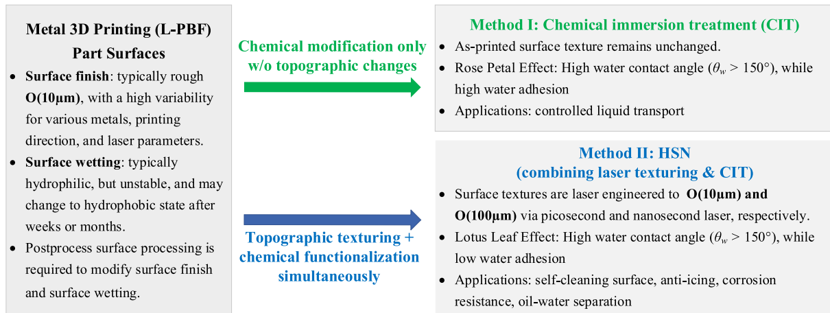
Fig. 1. Proposed superhydrophobic surface processing methods for metal 3d printed parts.
