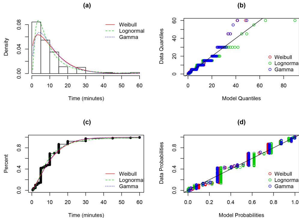
Figure 2. Expected preparation time from survey data and fitted models: (a) data histogram and probability density function, (b) quantile–quantile plot, (c) cumulative density function, and (d) probability–probability plot.
