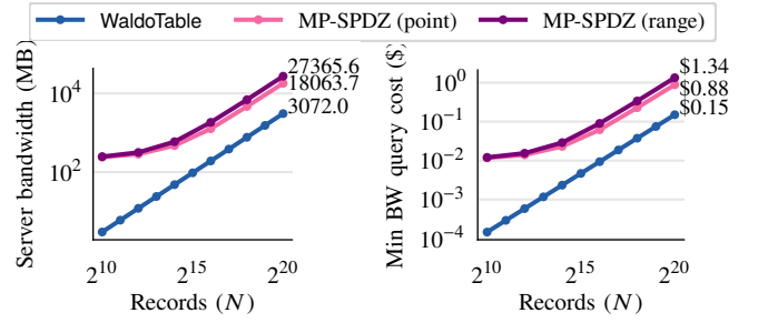
Fig. 10: Overhead and cost of total bandwidth between servers for a WaldoTable query with 8 predicates. We use the minimum AWS egress bandwidth cost of $0.05/GB [11] to compute the cost (bandwidth pricing is based on total egress bandwidth per month).
