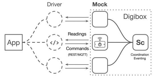
Figure 2: Application and mocks exchange messages in Digibox.
