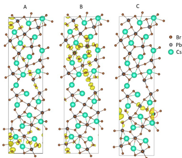
Figure 5. Charge densities of states for the configuration shown in Figure 3B: (A) state 339, (B) state 340 (HOMO), and (C) state 341 (LUMO). States 339 and 340 are HOMO-1 and HOMO and form the conduction band edge. They are more delocalized and contain contributions from grain boundary atoms. The deep electron trap state, LUMO, shown in (C) is localized around the circled Pb atom that has overly extended Pb-Br bonds (Figure S6A). The deep electron trap (C) is localized in the sub-boundary layer, similarly to the shall electron trap shown in Figure 4C.
