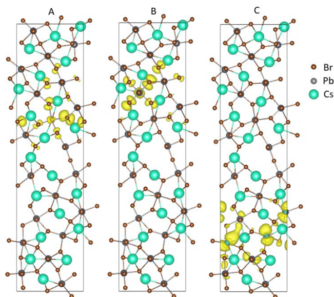
Figure 4. Charge densities of the trap states for the configuration shown in Figure 3A: (A) state 339, (B) state 340 (HOMO), and (C) state 341 (LUMO). The trap states are localized one or two layers away from the boundary. The boundary itself is sufficiently sparse and flexible to form the bonds needed to heal defects. The sub-boundary layers are distorted but cannot heal defects as well as the boundary itself. The hole trap shown in (B) is localized on a few Br atoms of the sub-boundary layer, in contrast to the hole trap of the optimized structure localized at the boundary (Figure 2A).
