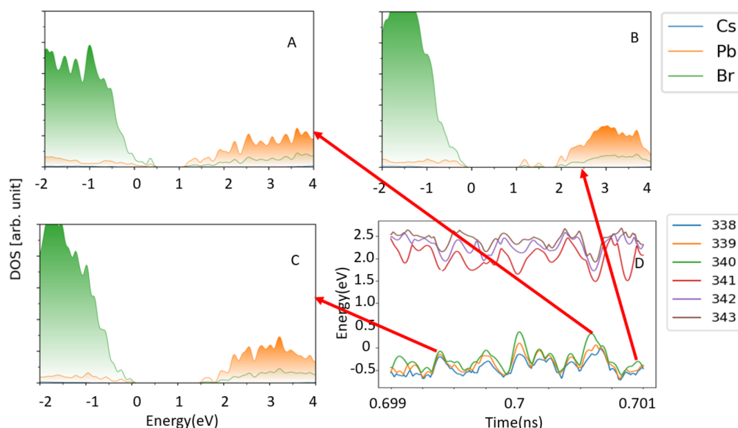
Figure 3. (A–C) Projected densities of states (DOS) at different points along a 2 ps part of the 1.5 ns trajectory (Figure S1). The zero energy is set at the valence band maximum. (D) Orbital energy levels along the 2 ps part of the 1.5 ns trajectory. The ab initio calculations are performed every 2 fs. The points in (D) are chosen from regions with good match between the machine learning and ab initio energies (Figure S2A). Trap states appear and disappear. Other examples are shown in Figure S3.
