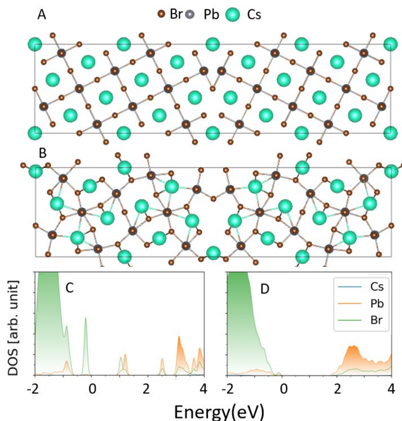
Figure 1. (A) Unoptimized \Sigma 5(210) grain boundary in \text{CsPbBr}_3 . (B) Optimized grain boundary. (C) Density of states (DOS) of the unoptimized structure (corresponds to A) and (D) DOS of the optimized structure (corresponds to B). A significant structural relaxation occurs at the boundary, and all midgap states disappear after the optimization. Note that the system contains two equivalent grain boundaries due to periodic boundary conditions, in the middle and at the edges of the shown structures.
