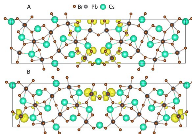
Figure 2. Charge densities of (A) HOMO and (B) LUMO in the optimized \Sigma 5(210) grain boundary structure. Although the states are strongly localized at the boundary, they are shallow traps (Figure 1D). The state energies are close to the corresponding bands, and the charges can easily escape into bands and undergo efficient long-range transport.
