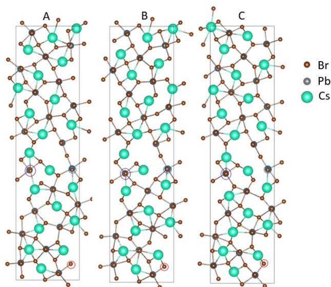
Figure 6. Geometric structures corresponding to the DOS shown in Figure 3. Parts A–C corresponds to parts A–C of Figure 3. Dangling bonds appear and disappear from time to time, giving rise to deep and shallow trap states and resulting in the reduced bandgap for some points along the trajectory. Geometric features of the marked atoms have high mutual information with the electronic energy levels (Table S1). The atoms are at the grain boundary and not sub-boundary, even though the deep trap states are localized in the sub-boundary (Figures 4 and 5) because most of the time the traps are not deep, and shallow traps are localized at the boundary (Figure 2). Note that the system has two grain boundaries, in the middle and top/bottom edges of the image, because of periodic boundary conditions.
