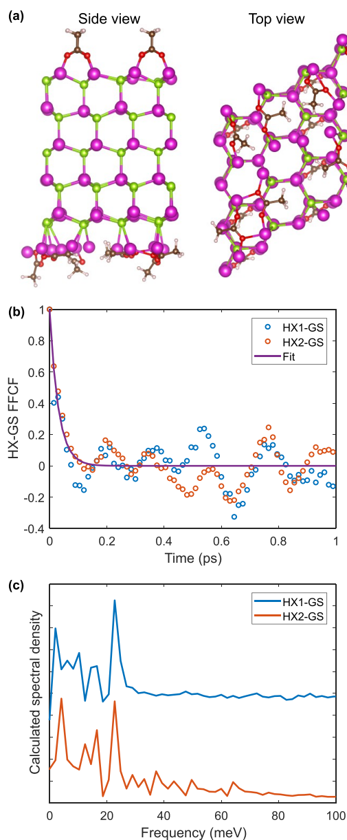
Figure 5. (a) Side and top views of the optimized 5-ML CdSe NPL structure, capped with acetic acid. The Cd, Se, O, C, and H atoms are denoted with purple, green, red, brown, and gray spheres, respectively. (b) Normalized FFCF of the energy gap HX1-GS (blue) and HX2-GS (red) transitions, obtained from the quantum-mechanical calculations. Both FFCFs are fitted simultaneously with a single-exponential function, yielding a lifetime of \sim 30 fs. (c) Fourier transformations of the calculated HX-GS FFCFs, where the HX1-GS plot is translated vertically for clarity.
