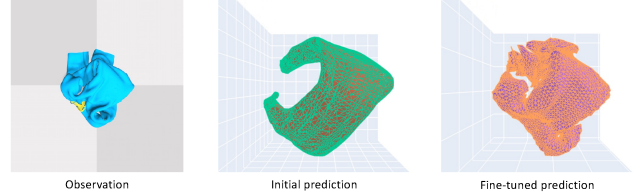
Fig. 3: An example showing the benefits of test-time finetuning: The network is able to correctly estimate the main cloth structure, but the initial predicted mesh may be overly smooth (center). Test-time finetuning significantly improves the quality of predicted mesh (right). For more examples, see our project website .
