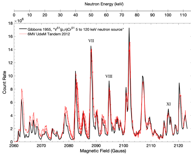
FIG. 4. Neutron yield of the ^{51}\text{V}(p,n)^{51}\text{Cr} reaction as a function of the magnetic field and corresponding neutron energy. The black curve is taken from [21], and is consistent with measurements done with the Tandem at the Université de Montréal [22] in red. The resonances VII, VIII, and XI chosen for the analysis are also indicated.
