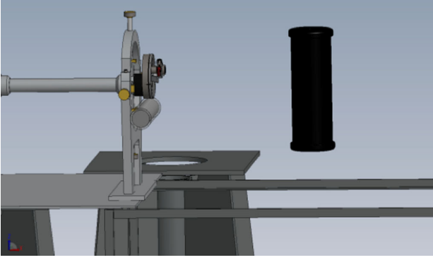
FIG. 9. Experimental setup at the Université de Montréal for measuring the neutron flux. Two ^3\text{He} counters were used: one directly below the ^{51}\text{V} target and one suspended directly downstream of the target.
