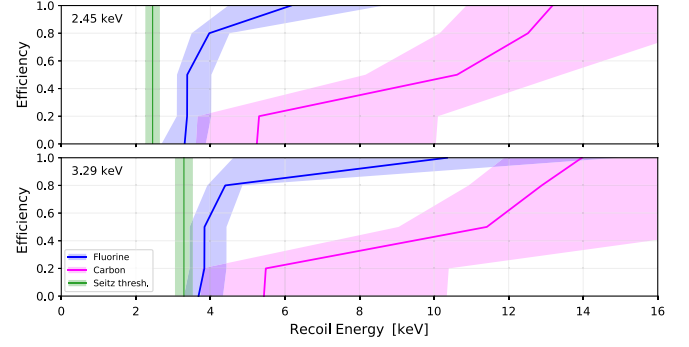
FIG. 12. Best-fit and 1\sigma error bands for the nucleation efficiency curves of fluorine (blue) and carbon (magenta), at the thresholds used in the PICO-60 WIMP search [5]. Error bands indicate the 1\sigma range of each knot position, so that every efficiency curve within 1\sigma of the best fit falls in the shaded area (but not every curve falling in the shaded area is within 1\sigma of the best fit). The corresponding Seitz thresholds are shown as a vertical green line, with the green band indicating the systematic threshold uncertainties described in Table IV.
