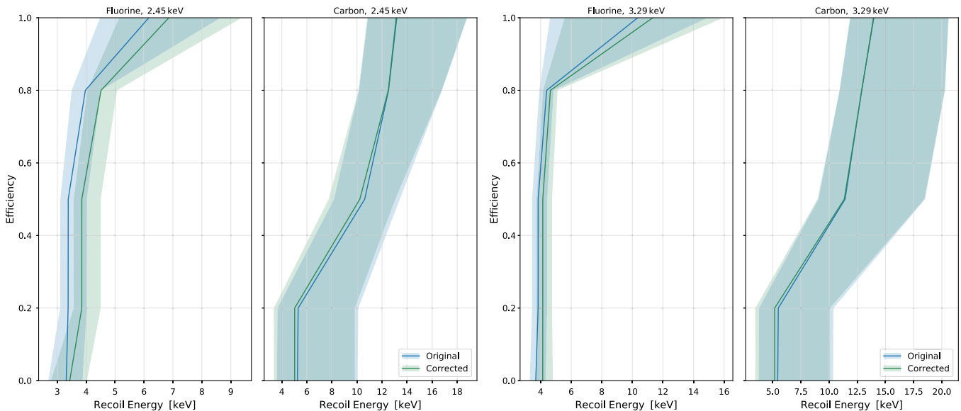
FIG. 22. Original (blue) and bias-corrected (green) nucleation efficiency curves and 1\sigma error bands for fluorine and carbon at thermodynamic thresholds of 2.45 keV (left) and 3.29 keV (right).
