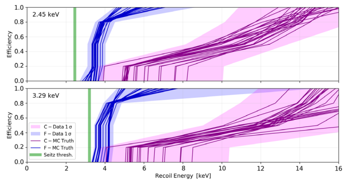
FIG. 19. Monte Carlo inputs for 25 “extended” parametrically simulated datasets, compared to the 1\sigma error bands from the fit to the real data.
