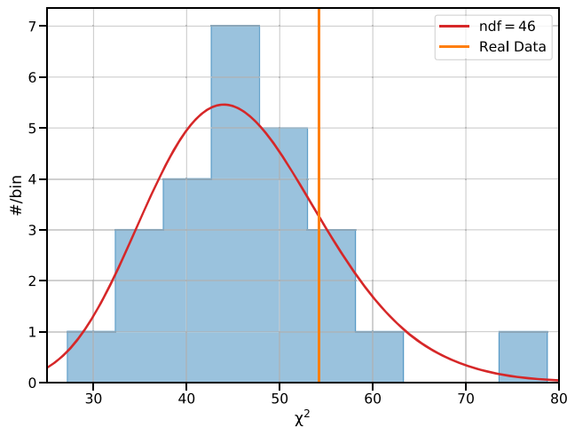
FIG. 16. \chi^2 data for the 25 simulated datasets (blue histogram), the best-fit \chi^2 distribution to that data (red curve), and the value of \chi^2 obtained for the real data (orange line). Based on the best-fit \chi^2 distribution, the real data give a p value of 0.19.
