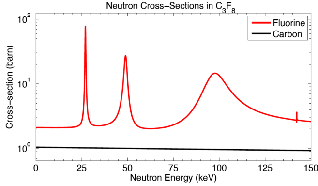
FIG. 2. Neutron-carbon and neutron-fluorine elastic scattering cross sections as a function of neutron energy, taken from [20], for the neutron energy range used during detector calibration.
