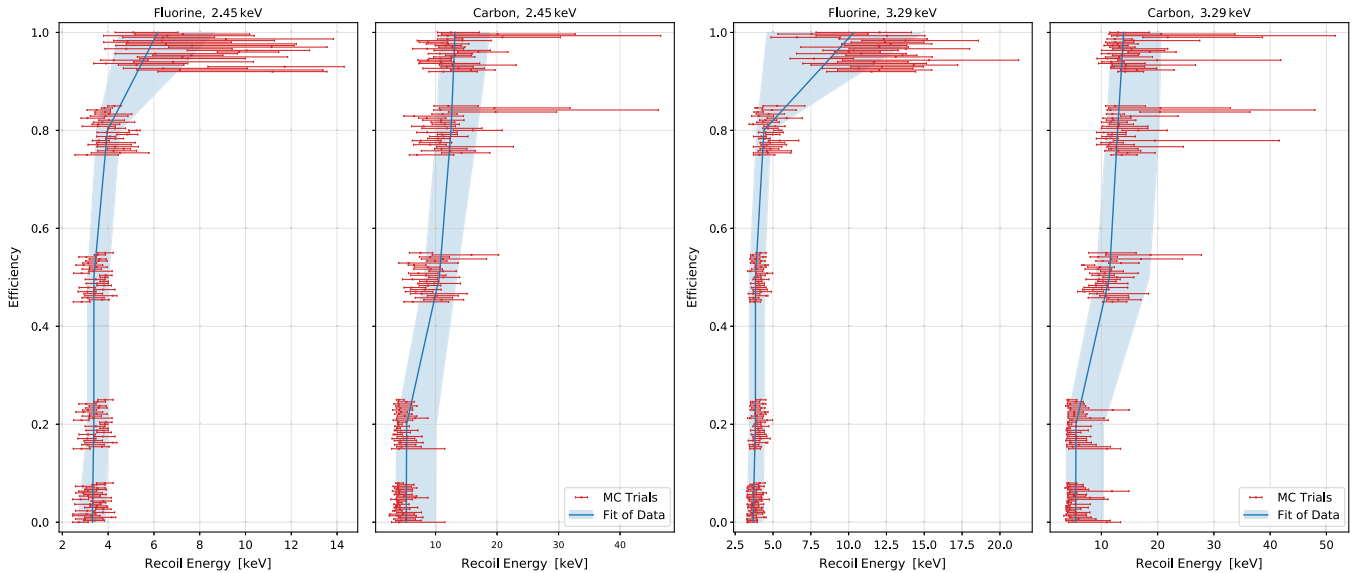
FIG. 15. Fits of 25 simulated datasets (red) compared to the best fit and 1\sigma band of the actual data (light blue) for the thresholds of 2.45 keV (left) and 3.29 keV (right).
