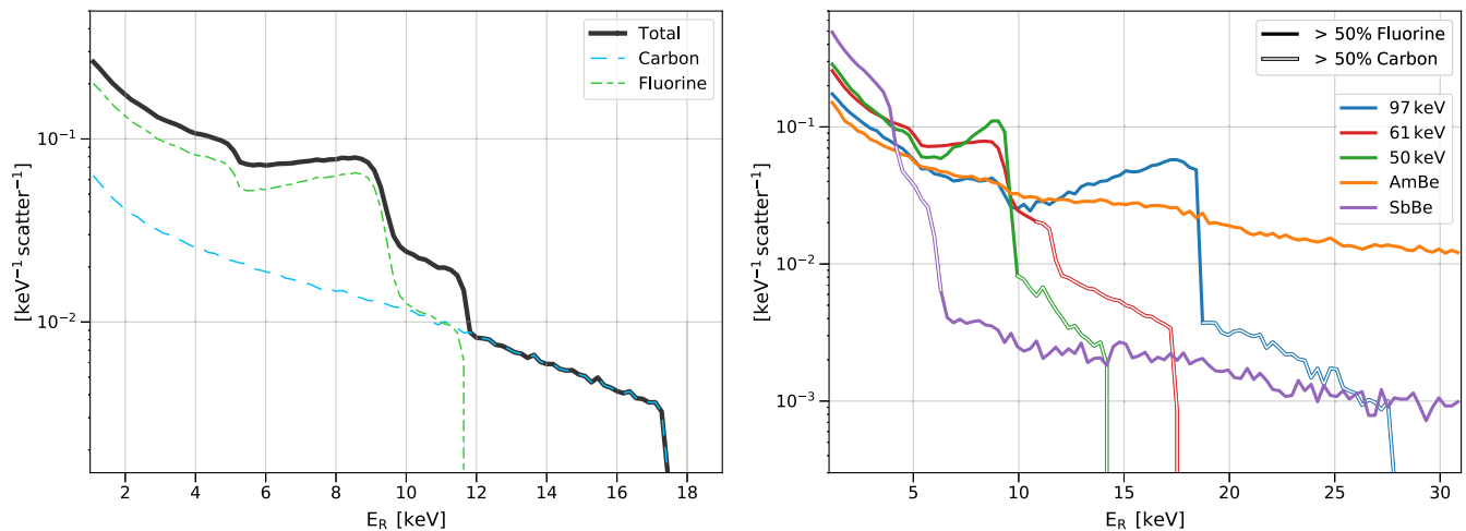
FIG. 8. Left: simulated recoil energy spectrum for the 61 keV beam experiment (2013) showing the separate contributions of scatters off of fluorine and carbon. Right: simulated recoil energy spectra for the 97 keV (2013), 61 keV (2013), and 50 keV (2014) beam experiments, as well as the SbBe and AmBe experiments. The dominance of scattering off of fluorine or carbon atoms is indicated by solid or hollow lines respectively. The spectra in the left and right panels are normalized to the total number of scatters in each simulation off of either target species.
