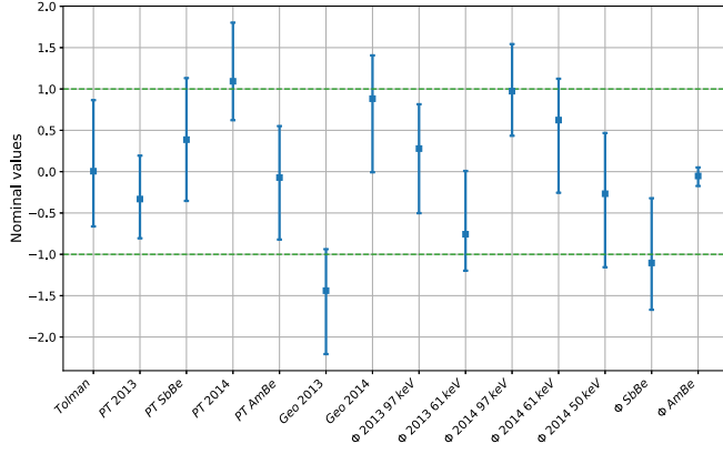
FIG. 14. Posterior constraints on nuisance parameters. Each nuisance parameter on this plot has a Gaussian prior with mean of 0 and standard deviation of 1. 11 of 14 best-fit values fall within the 1\sigma prior band, and in all cases the 1\sigma posterior error bars overlap with the 1\sigma prior band. The rightmost point, representing the neutron flux from the AmBe source in PICO-2L, is highly constrained by the data, largely due to the high-bubble-multiplicity resolved in that dataset.
