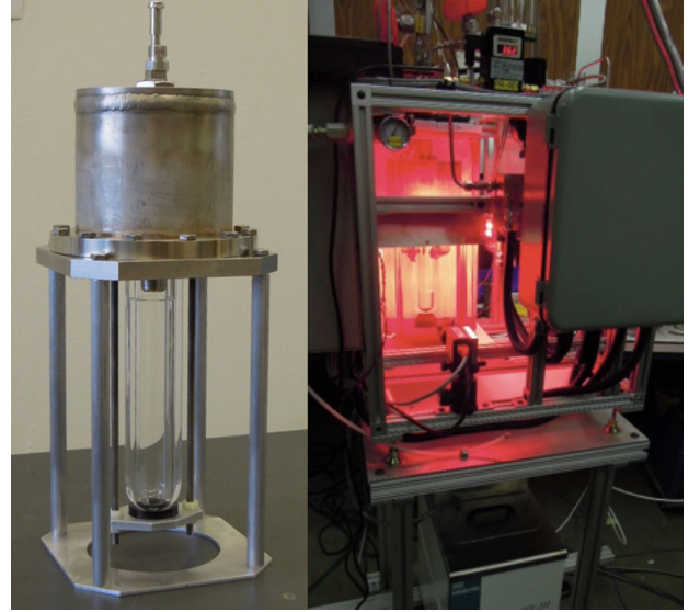
FIG. 3. PICO-0.1L detector. Left: the quartz vessel mounted to its hydraulic “top hat” containing the bellows used for pressure control of the chamber. Right: the complete setup of the chamber inside its thermal bath equipped with two piezoelectric sensors, two cameras and two LED panels, and CompactRIO-based pressure- and temperature-control system.
