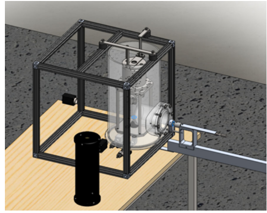
FIG. 6. Experimental setup of the SbBe calibration at the Université de Montréal. The PICO-0.1L test chamber is aligned with a graduated source rail to measure the SbBe source position. A ^3\text{He} counter is placed beside the bubble chamber to verify the neutron flux at the chamber.
