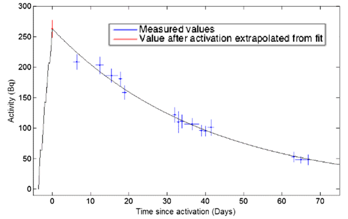
FIG. 10. ^{51}\text{Cr} activity in the ^{51}\text{V} target after exposure to the proton beam. These data were taken at a proton beam energy corresponding to 50-keV neutron production, with a fresh ^{51}\text{V} target (no ^{51}\text{Cr} activity prior to exposure). A single-parameter fit with fixed ^{51}\text{Cr} half-life gives the activation rate of the target when exposed to the beam.
