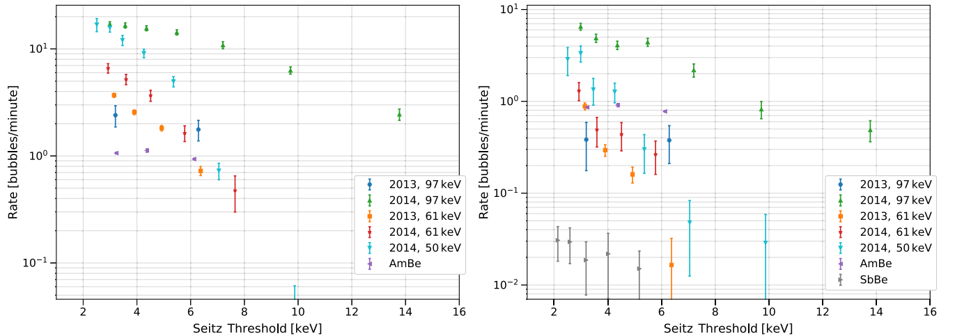
FIG. 7. Background-subtracted measured rates of events with one or more bubble (left) and with two or more bubbles (right), in units of bubbles per minute (counting each bubble separately in multibubble events). Error bars show statistical uncertainty only. The background rates subtracted were approximately 0.2 single bubbles/minute for beam data (much less for higher multiplicity events), 0.004 2 bubble events per minute for the SbBe data, and 0 for the AmBe data (below the sensitivity of the background measurement). Data at Seitz thresholds greater than 3.6 keV are not included in the full analysis, but the trends with Seitz threshold illustrate the relative sensitivity of each dataset to the underlying nuclear recoil detection threshold.
