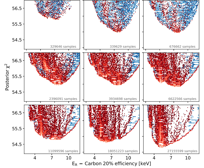
FIG. 17. The sampled \chi^2 (or -2 \log \mathcal{L} ) distribution projected into x_{C,20\%,2.45 \text{ keV}} —the carbon recoil energy with 20% nucleation efficiency at a thermodynamic threshold of 2.45 keV—showing the progressive sampling of the distribution over many epochs (blue) with the events selected to start the next epoch shown in red. The cumulative number of points evaluated is indicated in each frame.
