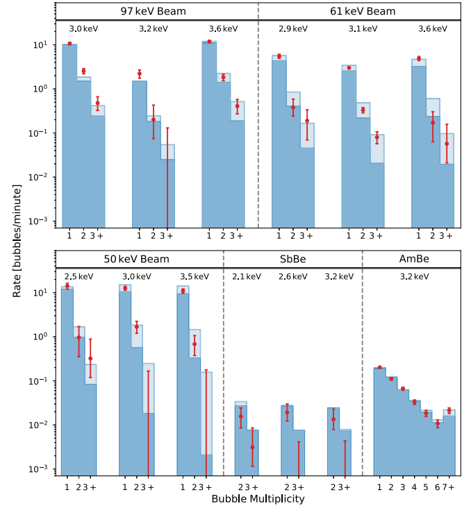
FIG. 13. Comparison between the measured bubble rate (in bubbles per minutes) and fit of the data. The red points are the experimental data points with Feldman-Cousins 1\sigma confidence intervals as error bars on the Poisson mean in each bin [28]. The blue histograms are the result of the MCNP/GEANT4 simulations convolved with the bubble efficiency curves fit to the data; the empty blue bars represent the \pm 1\sigma error window of the fit.
