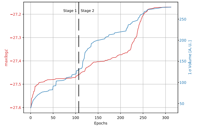
FIG. 18. Progression of the maximum log-likelihood and “ 1\sigma ” volume of the likelihood function.
