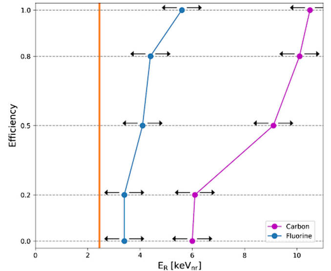
FIG. 11. Cartoon showing the piecewise linear model used in this analysis. Each blue (purple) dot represents a movable set point of fluorine (carbon) at efficiencies of 0, 0.2, 0.5, 0.8, and 1. In this analysis, the carbon threshold is required to lie to the right of the fluorine threshold, which in turn must lie to the right of the Seitz threshold (orange vertical line).
