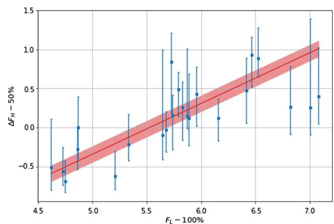
FIG. 20. Bias of the 50% efficiency point of fluorine at 3.29 keV vs the true value of the fluorine 100% efficiency point at 2.45 keV thermodynamic threshold. The Monte Carlo trial results are shown in blue, and a linear fit to the points with 1\sigma error band are shown in red.
