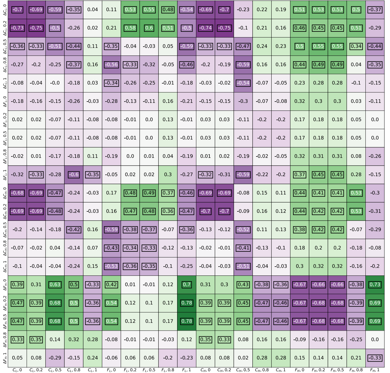
FIG. 21. Spearman correlation coefficient for the bias of every parameter of interest (y axis) vs the simulation input value (x axis). The color scale is indicative of this coefficient as well for easier visualization, and instances of a statistically significant correlation are boxed. Note that in this variable abbreviation, “C” or “F” indicate the target atom, “L” or “H” indicate the thermodynamic threshold fencepost as 2.45 or 3.29 keV respectively (“Low” or “High”), and the numeric value is the efficiency fencepost.
