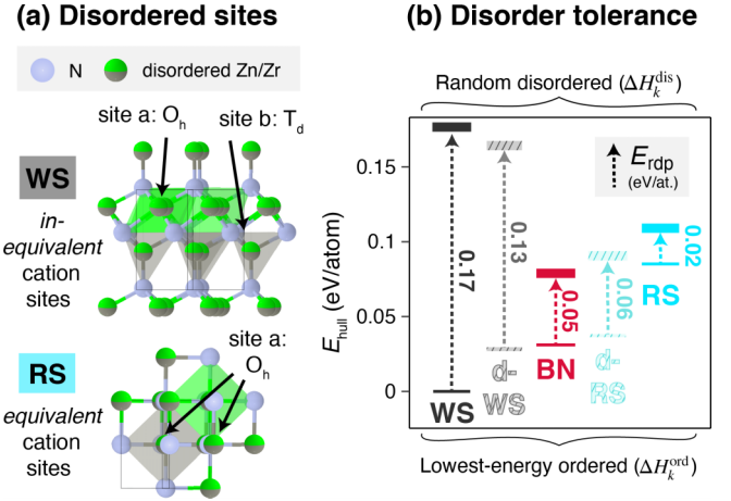
FIG. 5. (a) Schematic of the WS- and RS-derived structures with cation site disorder as an example of structures with inequivalent and equivalent cation sites, respectively. (b) Comparison of formation energies of the lowest-energy ordered polymorph structure ( \Delta H_k^{\text{ord}} ) and of the random disordered structure ( \Delta H_k^{\text{dis}} ) for each prototype class plotted in Fig. 3. The E_{\text{rdp}} descriptor is shown, with a lower E_{\text{rdp}} correlating to the higher-disorder tolerances in the BN and RS structures that are observed experimentally (see SM [18]).
