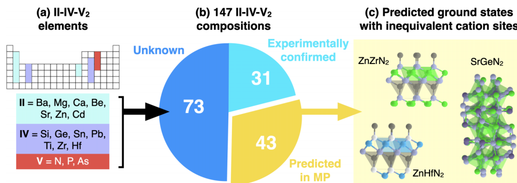
FIG. 7. Assessment of the role of cation disorder tolerance in emerging ternary pnictides. (a) Elements within the II-IV- V_2 composition space. (b) The distribution of composition spaces within the Materials Project (MP) database. (c) Three example systems from the “predicted in MP” category where cations occupy symmetrically inequivalent lattice sites.
