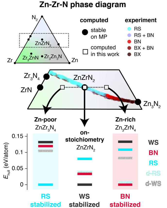
FIG. 6. Ternary phase diagram of Zn-Zr-N and a closeup of the \text{Zn}_{1-x}\text{Zr}_x\text{N} region, with computed compounds from the Materials Project designated. Colored circles depict the approximate composition and associated phases of experimental data from this work (see Fig. 2). Computed compositions from this study are represented with unfilled squares in the phase diagram, and for each composition the lowest formation energy structure for a given class is plotted with colored bars.
