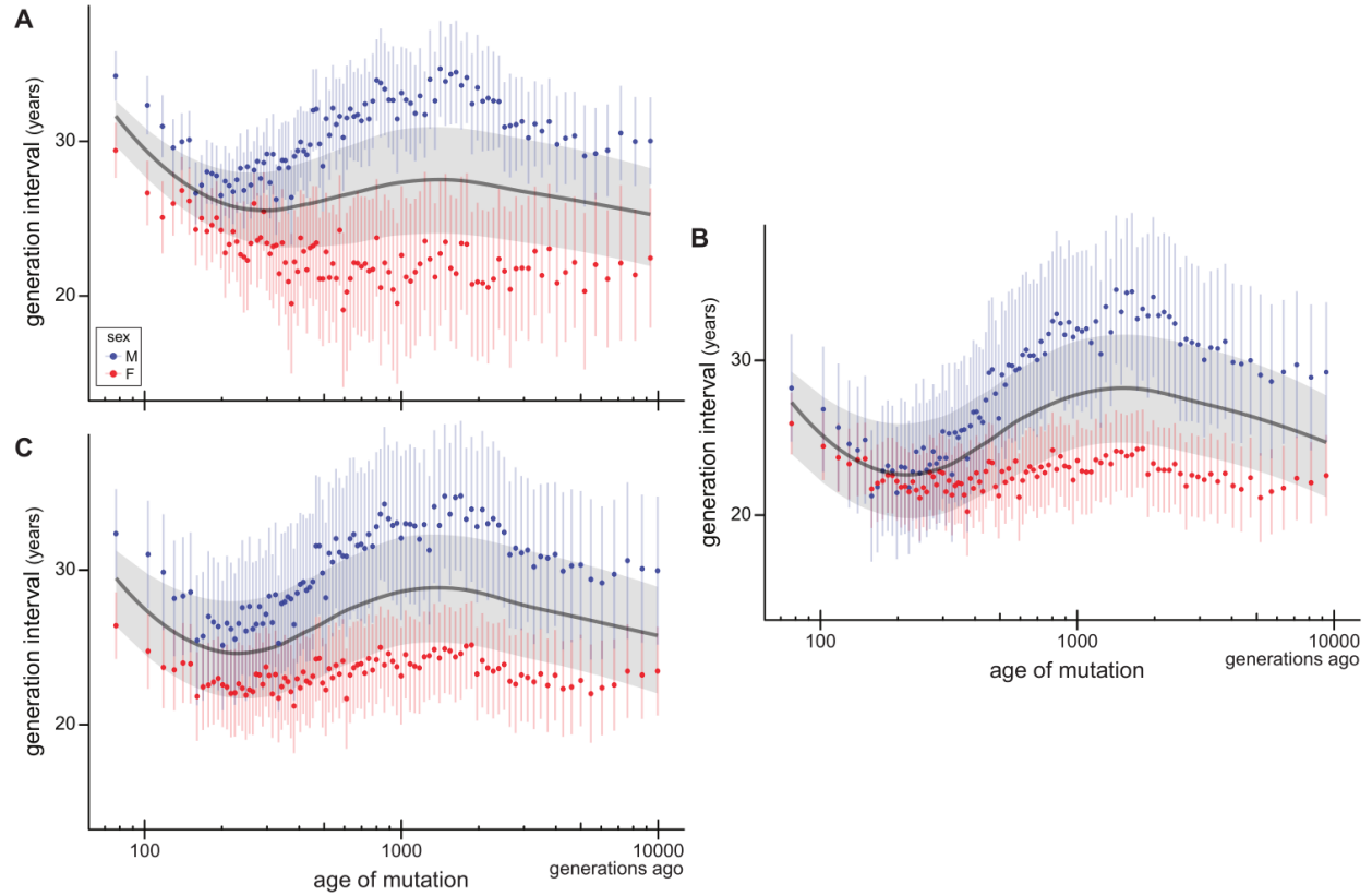
Figure S12. Generation intervals estimated with relaxed assumptions
