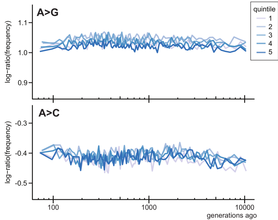
Figure S11. No accumulation of effects from biased gene conversion through time
