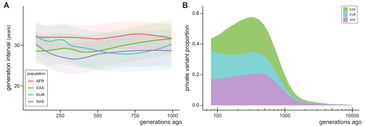
Figure S5. Population-specific estimates from private variants
