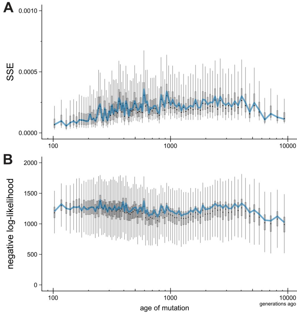
Figure S6. Goodness-of-fit through time
