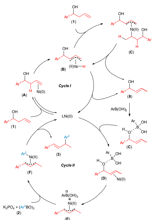
Scheme 10. Proposed mechanism.
