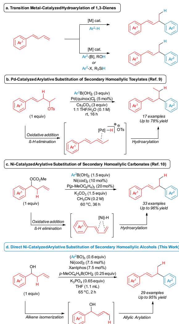
Scheme 1 Transition metal-catalyzed formation of allylic arenes via hydroarylation and arylative substitutions.
