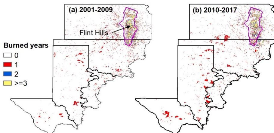
Fig. 3. Number of burned years across the southern Great Plains within the time period (a) 2001–2009, (b) 2010–2017. Data source: MODIS product FireCCI51.
