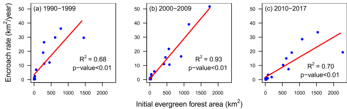
Fig. 9. Scatterplot of mean annual encroachment rate ( \text{km}^2/\text{year} ) versus initial evergreen forest area ( \text{km}^2 ) for the temporal stage (a) 1990–1999, (b) 2000–2009, and (c) 2010–2017. Fitted regression lines and details are overlaid on respective scatterplots. Each point represents one of the 18 ecoregions under study.
