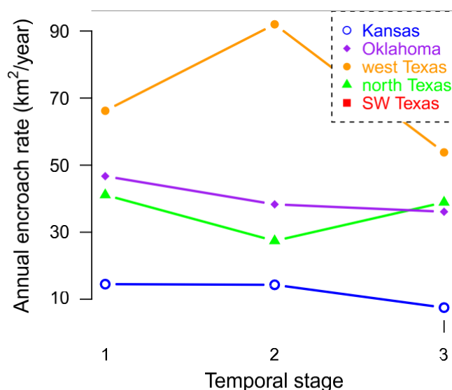
Fig. 8. Comparison of mean annual encroachment rate ( \text{km}^2/\text{year} ) of evergreen forest among the five sub-regions over the three temporal stages. In the x-axis, 1 represents the temporal stage 1990–1999, 2 represents 2000–2009, 3 represents 2010–2017.
