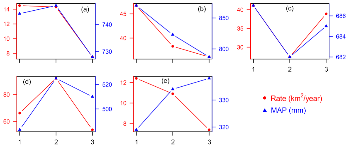
Fig. 10. Comparison of mean annual encroachment rate ( \text{km}^2/\text{year} ) with concurrent average MAP for (a) Kansas, (b) Oklahoma, (c) north Texas, (d) west Texas, (e) southwest Texas. In the x-axis, 1 represents the temporal stage 1990–1999, 2 represents 2000–2009, 3 represents 2010–2017.
