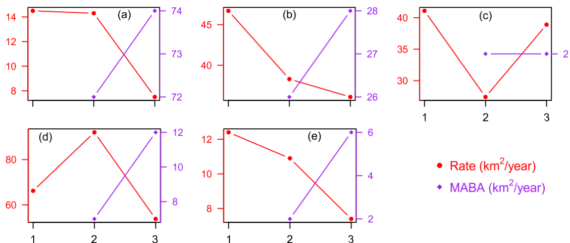
Fig. 11. Comparison of mean annual encroachment rate ( \text{km}^2/\text{year} ) with concurrent mean annual burned area (MABA, \text{km}^2/\text{year} ) for (a) Kansas, (b) Oklahoma, (c) north Texas, (d) west Texas, (e) southwest Texas. In the x-axis, 1 represents 1990–1999, 2 represents 2000–2009, 3 represents 2010–2017.
