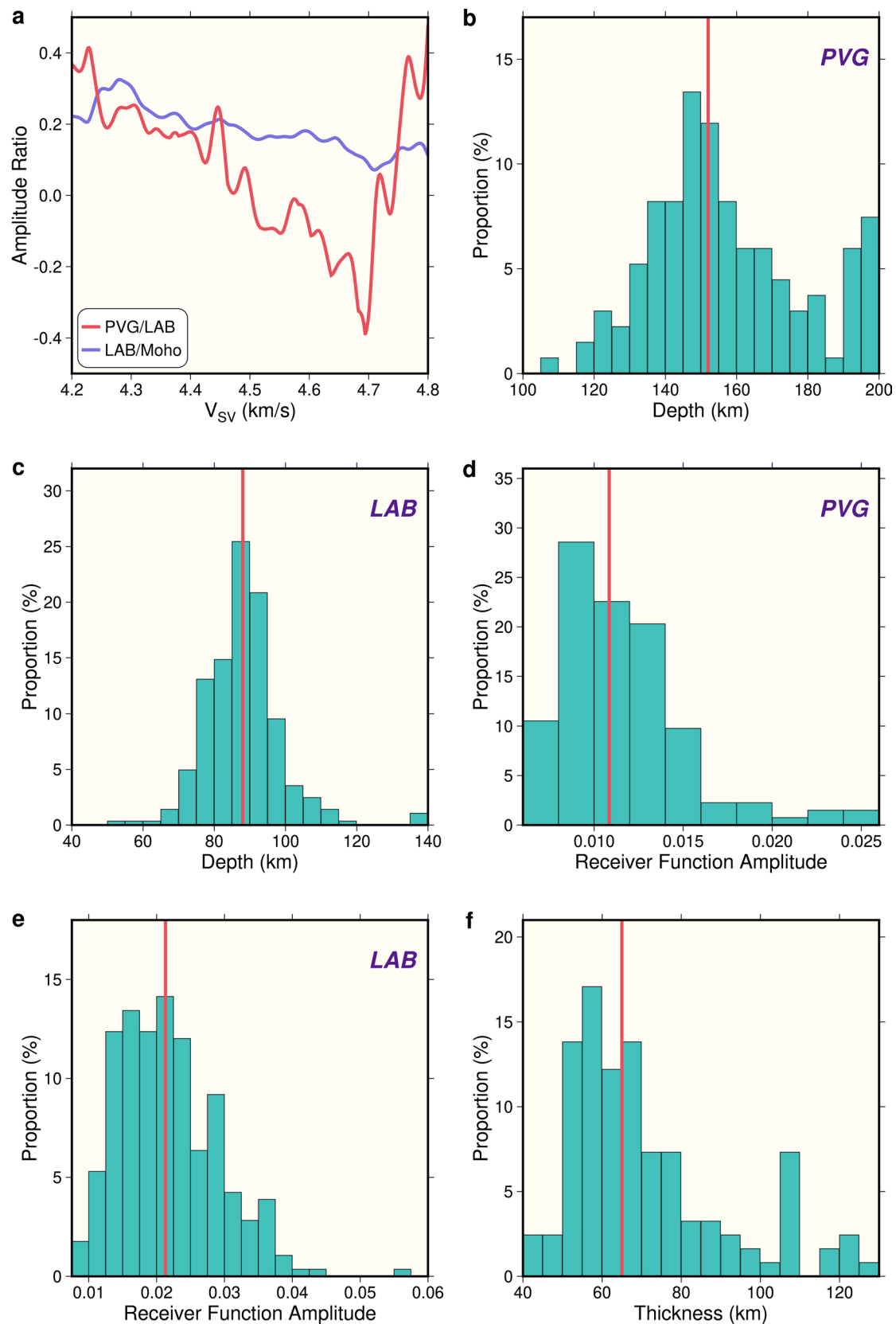
Extended Data Fig. 4 | Properties of the PVG and NVG (LAB) phases. a.
