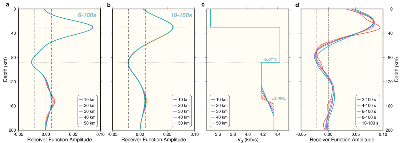
Extended Data Fig. 5 | The effects of waveform frequency content. Synthetic Sp receiver functions for the velocity models in c were filtered by 6–100 s (a) and 10–100 s (b) bandpass filters before deconvolution. Colors correspond to velocity gradients from the LVZ to the underlying asthenosphere over 10 to 50 km depth ranges (as shown in c). Horizontal dotted lines show the center of V_s discontinuities. Vertical dashed lines mark zero amplitude for receiver functions. The vertical dotted-dashed lines in a & b show the median NVG and PVG amplitudes (Extended Data Fig. 4) of the observed phases when filtered over 10–100 s. This analysis shows that the 10–100 s filter receiver functions are
