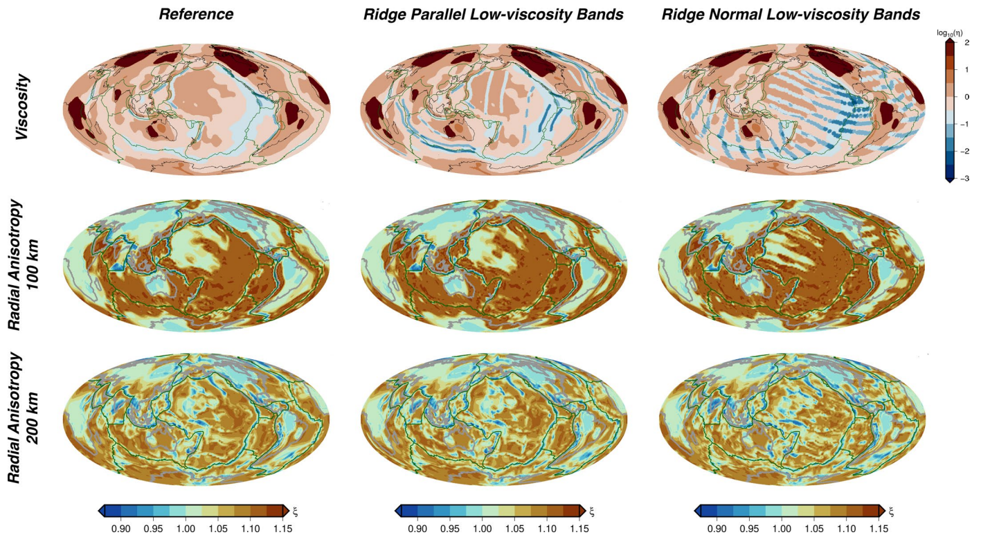
Extended Data Fig. 10 | Modelled 3D radial anisotropy with localized asthenospheric viscosity layering. Model results in this figure are all from ref. 43 . The first row shows the relative mantle viscosity at 134 km depth, and in the corresponding second and third columns, low-viscosity bands parallel or perpendicular to the mid-ocean ridges are present at depths between 100 and
