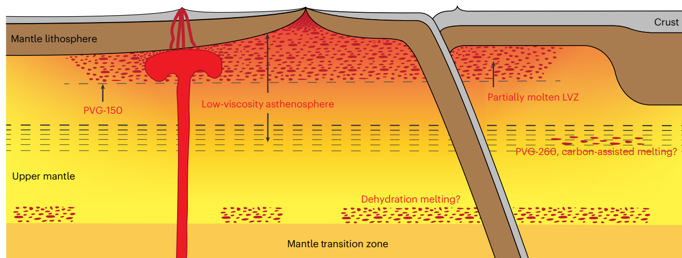
Fig. 5 | Interpretation of the observed PVG-150 and PVG-260 mantle velocity gradients. The PVG-150 (shallow dashed horizontal line) represents the base of a melt-rich LVZ within the asthenosphere that has little impact on viscosity. The overall low viscosity of the asthenosphere, including its gradual lower boundary
