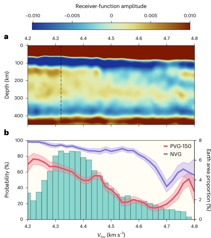
Fig. 2 | The relationship between receiver-function phases and asthenospheric V_{sv} . a , Receiver functions binned by average V_{sv} (ref. 22 ) at depths of 110–130 km beneath the station. A clear PVG-150 phase is observed where V_{sv} is less than 4.32 km s -1 (dashed line). b , The probabilities (curves) that a PVG-150/LAB phase at the bottom/top of the LVZ is observed versus average mantle V_{sv} at depths of 110–130 km. The shaded envelopes indicate one standard deviation. Histogram shows the proportions of Earth area with a given average V_{sv} (scale at right).
