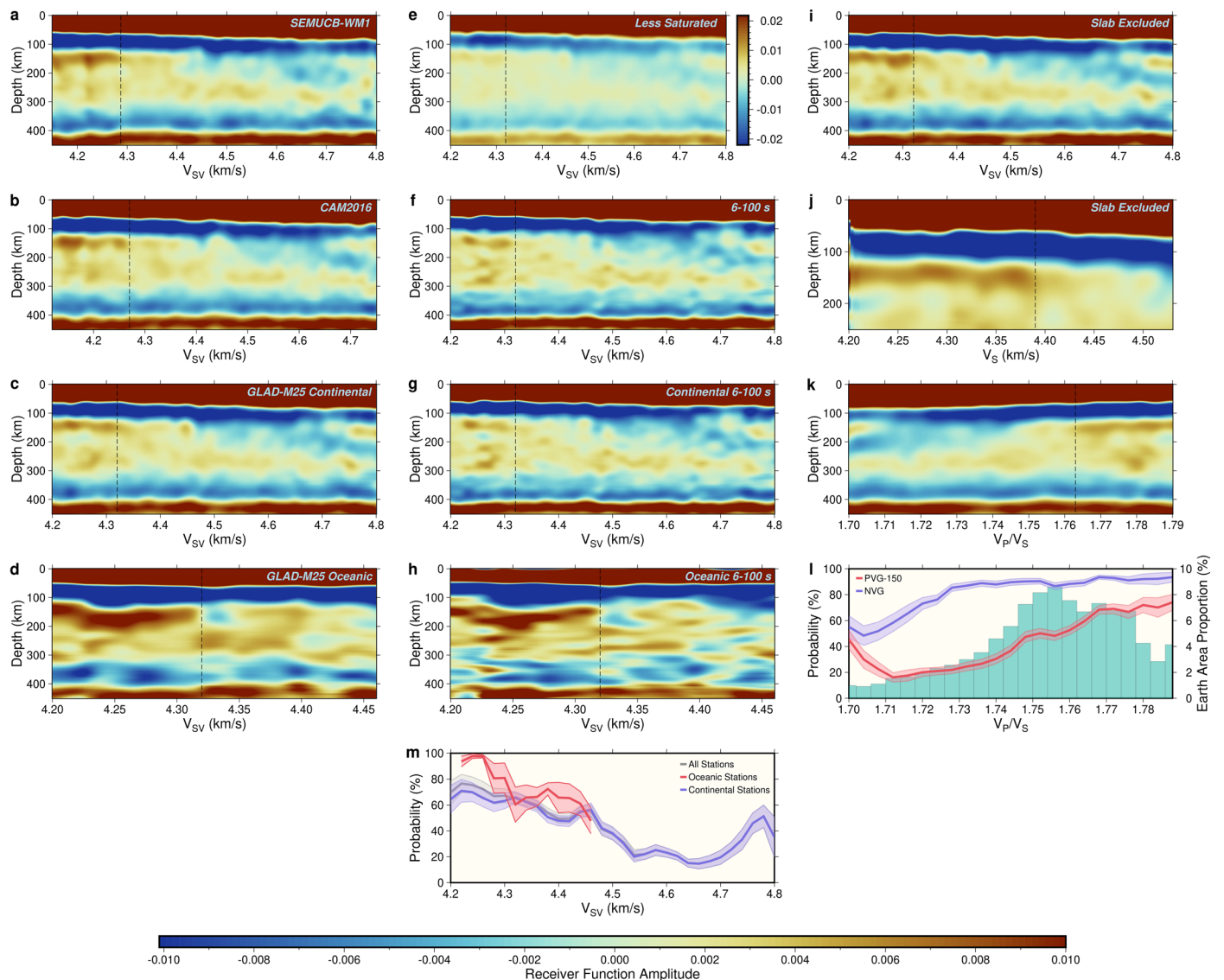
Extended Data Fig. 3 | Relationships between receiver functions and mantle properties. a–b. Observed receiver functions binned by average V_{SV} at 110–130 km depths beneath the station, similar to Fig. 2a, but based on different reference velocity models: (a) SEMUCB-WM1 (ref. 21 ) (b) CAM2016 (ref. 2 ). c–d. Similar to Fig. 2a, with the same reference model 22 , but using only the 644 continental stations (c) or only the 74 oceanic stations (d) . A station was designated as oceanic if its crustal type in CRUST1.0 (ref. 65 ) is normal oceanic, oceans 3 Myr and younger, melt affected ocean and oceanic plateaus, or oceanic plateau with continental crust. e. The same as Fig. 2a, but with a less saturated color scale to show the NVG phase better. f–h. Similar to Fig. 2a and panels c and d , respectively, but filtered with a 6–100 s bandpass filter instead of 10–100 s.
