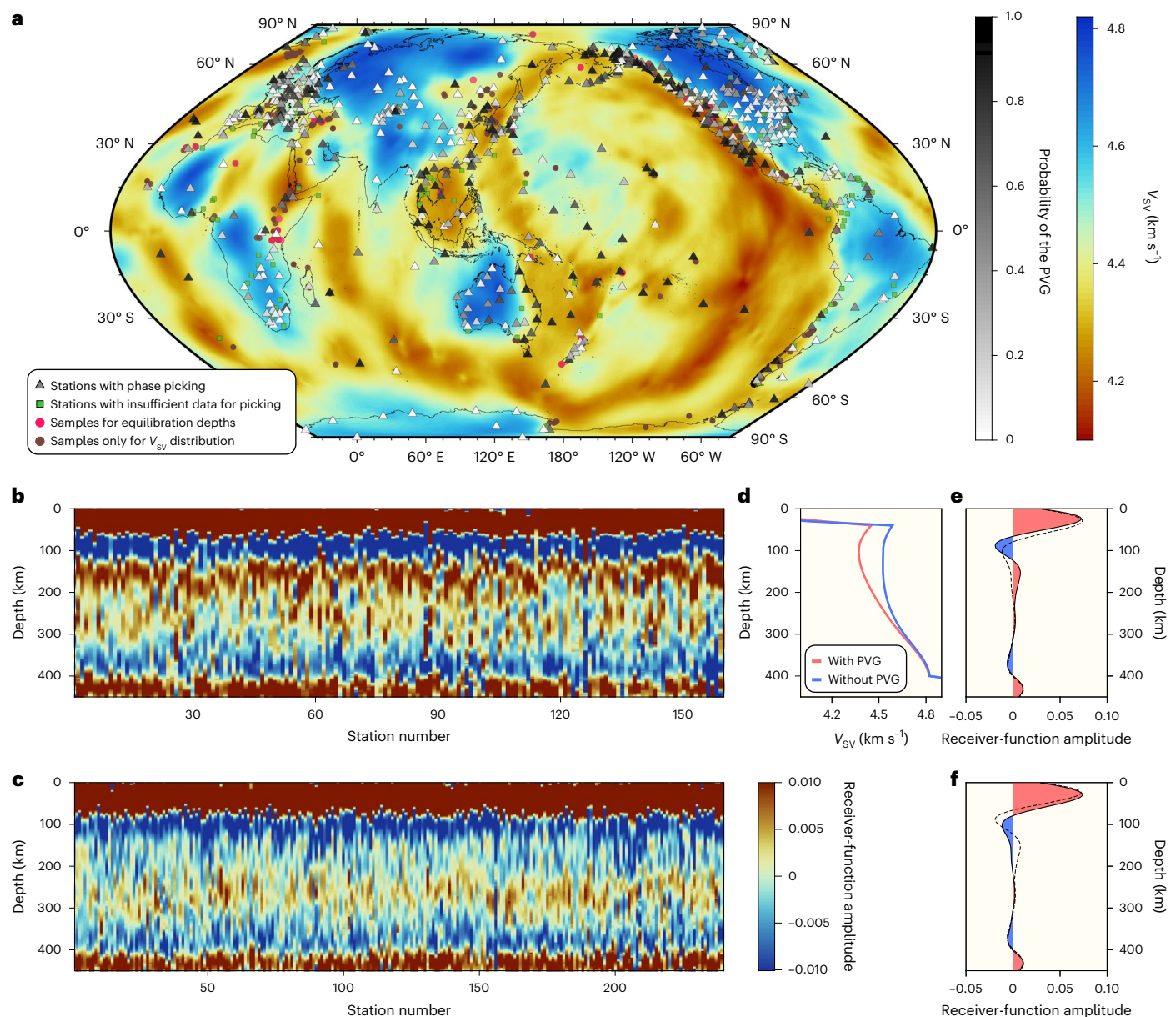
Fig. 1 | Globally distributed receiver functions. a , Stations shaded by PVG-150 probability (triangles) or without sufficient data for probability quantification (squares). Background shows average V_{sv} at 110–130 km depths 22 . Dots are basalt samples used for distributions of melt equilibration depths (Fig. 3d) and sample V_{sv} (Fig. 3d inset). b, c , Sp receiver functions for single stations with ( b ) and
