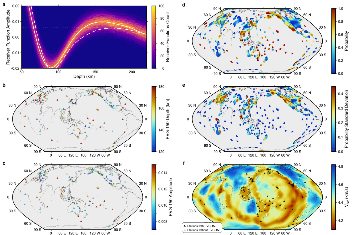
Extended Data Fig. 1 | Probabilities of the PVG-150 phase. a. Example of estimating the probability of the PVG-150 phase from the S_p receiver function at station SMAI (Antarctic Peninsula) in network AI. The solid line shows the receiver function amplitude. The background shows the heat map for the 3,000 perturbed receiver functions. The dashed line shows one of the perturbed receiver functions, whose maximum amplitude is below the threshold amplitude for picking of 0.006 (dotted line). In this case, no PVG-150 phase is picked, although the original stacked receiver function has an amplitude much higher than the threshold. Among all perturbed receiver functions, 96.9% produce a picked PVG-150 phase. The other dotted line shows zero amplitude. b. Map of the depth of the PVG-150 phase for those with probabilities over 0.8 (Fig. 1a). c.
