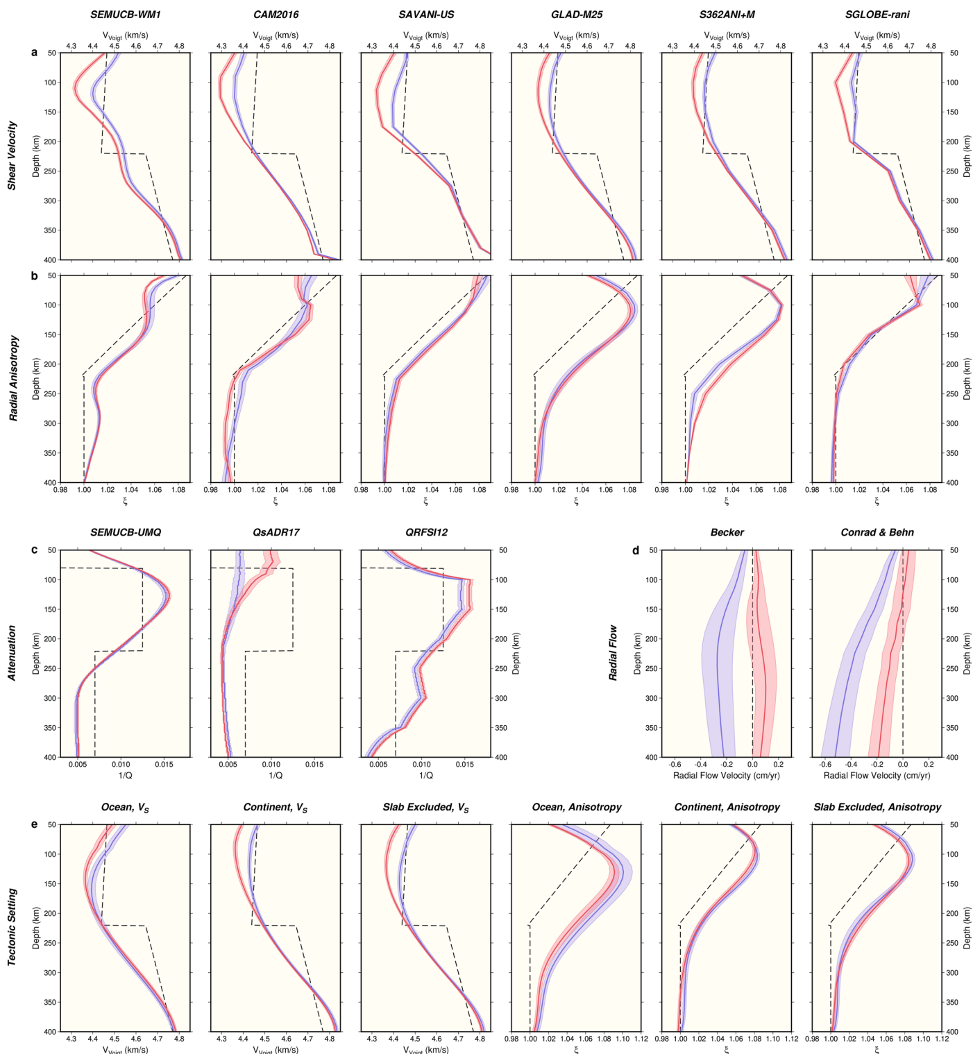
Extended Data Fig. 8 | Mantle property contrasts between areas with and without the PVG-150 phase. The first three rows show differences in weighted averaged (Eq. 4) profiles of V_{\text{Voigt}} (a), \xi (b), attenuation (c) and radial mantle flow velocity (d) for stations with (red lines) and without (blue lines) the PVG-150 phase. The fourth row (e) shows differences in weighted averaged profiles of V_{\text{Voigt}} and \xi for different tectonic settings. Transparent areas show one standard deviation for the averaged profiles. Black dashed lines are reference values from PREM 27 . For V_{\text{Voigt}} and \xi , columns are for velocity models SEMUCB-WM1 (ref. 21),
