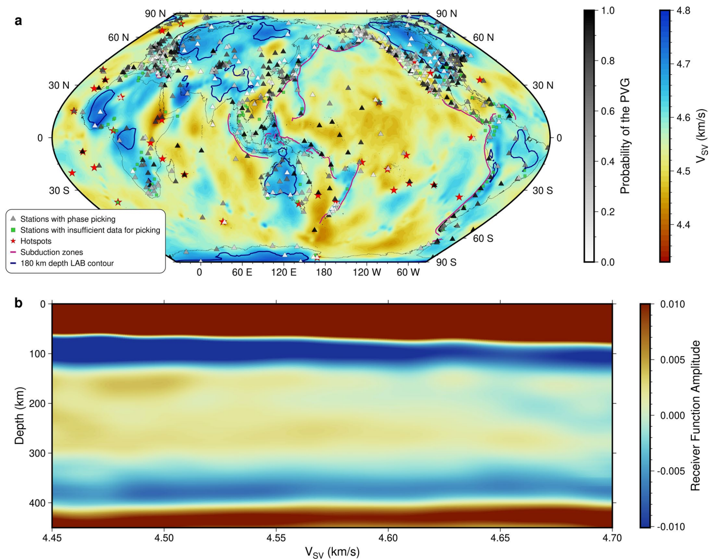
Extended Data Fig. 2 | The PVG-260 phase. a. Map similar to Fig. 1a, but in this case PVGs were picked between 230 and 350 km depths, which is the potential depth range for X-discontinuities 25 . The background V_{SV} 22 is at 260 km depth. Hotspots 61–63 , subduction zones 64 and the rim of cratons represented by the 180
