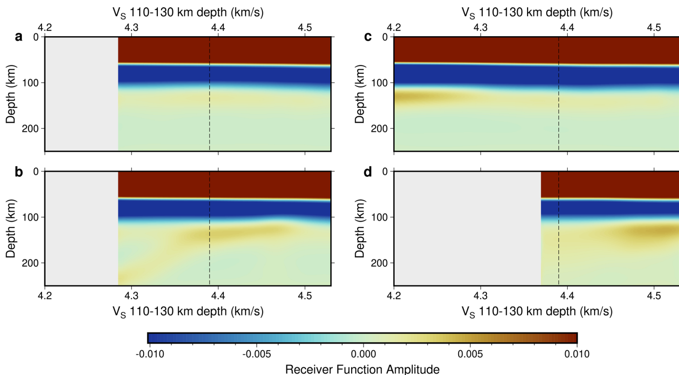
Extended Data Fig. 7 | Binned synthetic receiver functions. a. Predicted receiver functions similar to Fig. 3b, but produced from velocities that are those in Fig. 3a minus the poroelasticity effect of partial melt 33 . b. Similar to a, but velocities also include the effects of a small amount of melt on diffusion
