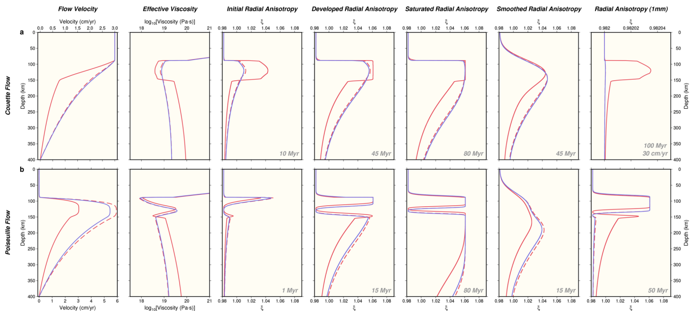
Extended Data Fig. 9 | 1D modeling of radial anisotropy assuming different effects of partial melt. First and second rows illustrate the 1D models of mantle Couette (a) and Poiseuille flow (b) (1,450 °C cases). The first column shows the solution for mantle flow velocity, and the second column is the equivalent mantle viscosity. The 3 rd to 5 th columns show predicted \xi for different points in time: early in strain accumulation; when radial anisotropy has developed to resemble the observed profiles; and when anisotropy has reached its saturation level over a broad depth range. The time intervals of strain accumulation for these three stages are labelled in the bottom right corners. The sixth column shows the product of the fourth column convolved with a Gaussian whose standard
