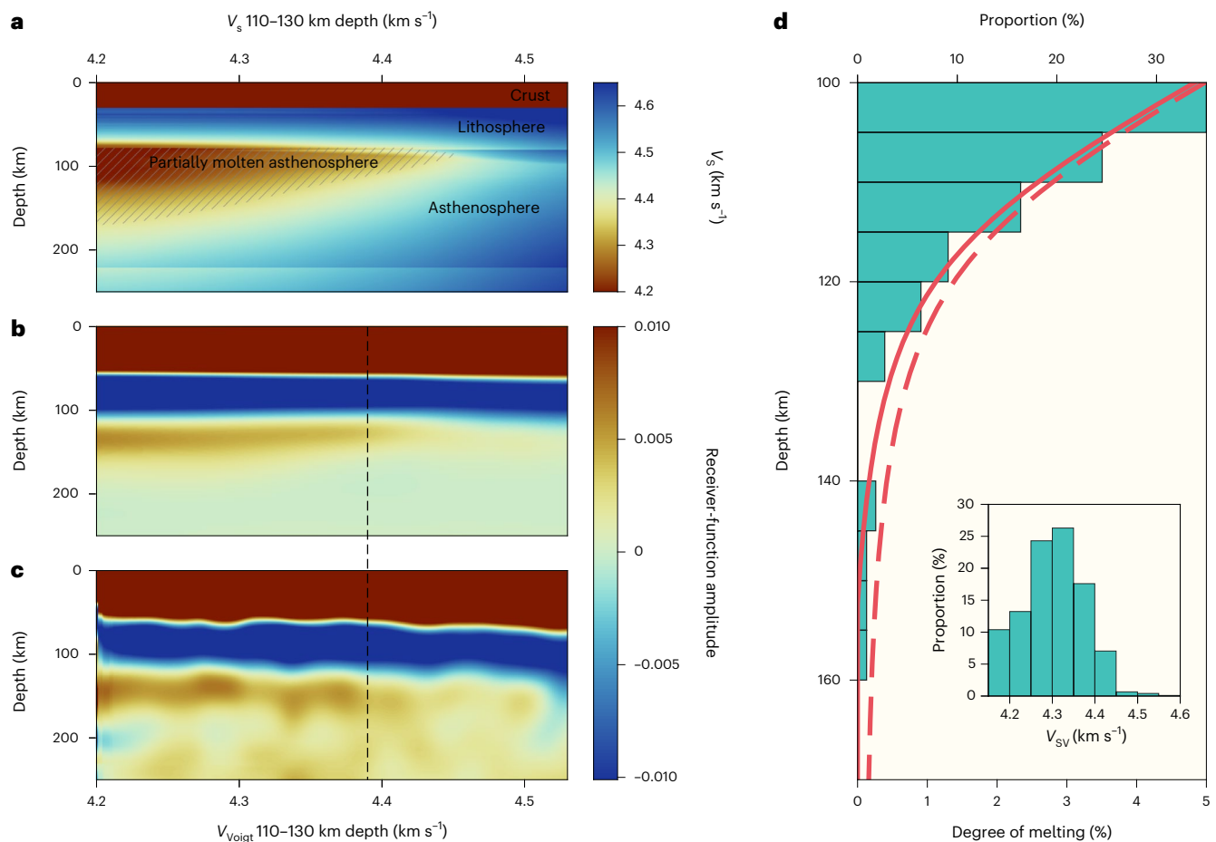
Fig. 3 | Modelling the PVG-150 with partial melt. a , Predicted seismic velocities for varying mantle conditions (Methods) binned by average isotropic V_s (110–130 km). Shading indicates average melt fraction >0.2\% . b , Binned synthetic receiver functions predicted for velocities in a . c , Observed receiver functions binned by V_{\text{Voigt}} (110–130 km) (ref. 22 ). Dashed line in b and c is V_s -equivalent
