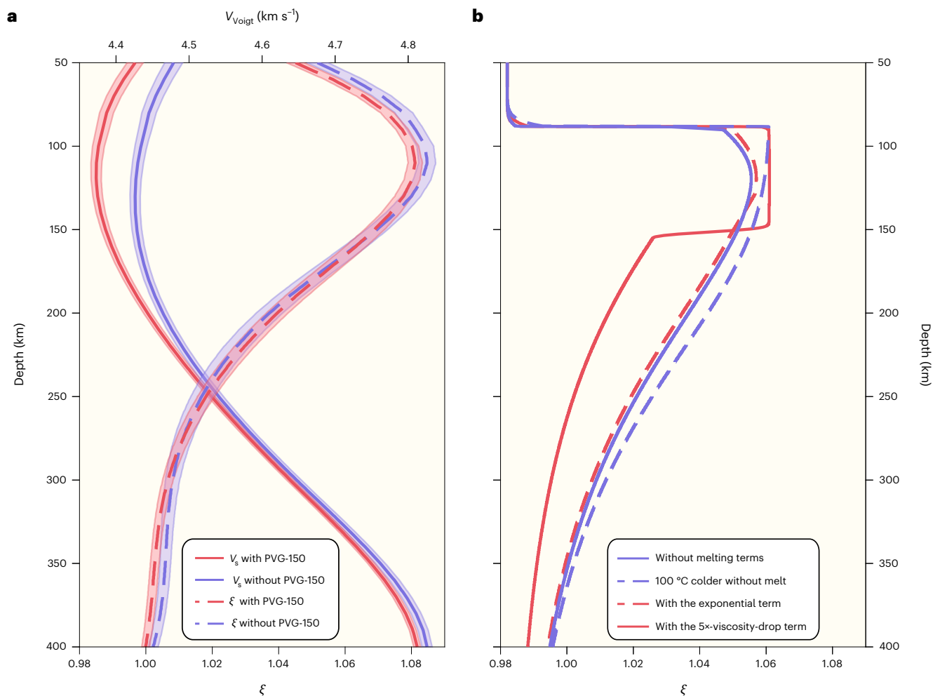
Fig. 4 | The PVG-150, anisotropy, melt and viscosity. a, Average V_{\text{Voigt}} (solid lines) and \xi (ref. 22 ) (dashed lines) for stations with and without the PVG-150. Transparent areas indicate one standard deviation. b, Predicted radial anisotropy \xi (ref. 13 ) for horizontal Couette flow (3 cm \text{yr}^{-1} surface velocity and 45 Myr duration). Blue solid/dashed line: no melt effects on viscosity for
