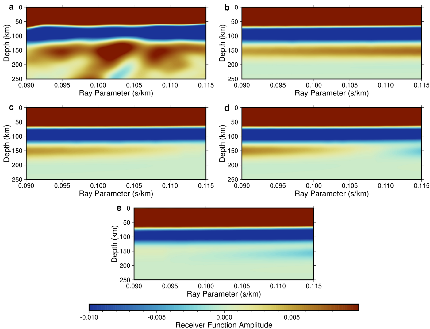
Extended Data Fig. 6 | Ray parameter dependence of the Sp receiver functions. a. Observed Sp receiver functions binned as a function of ray parameter. b. Synthetic Sp receiver functions for a mantle with an isotropic LVZ (LVZ V_s lower than the underlying mantle). c. Synthetic Sp receiver functions where the LVZ is radially anisotropic with \xi equal to 1.1 but has no P anisotropy, and its V_{\text{Voigt}} is the same as the underlying mantle. d. The LVZ contains P
