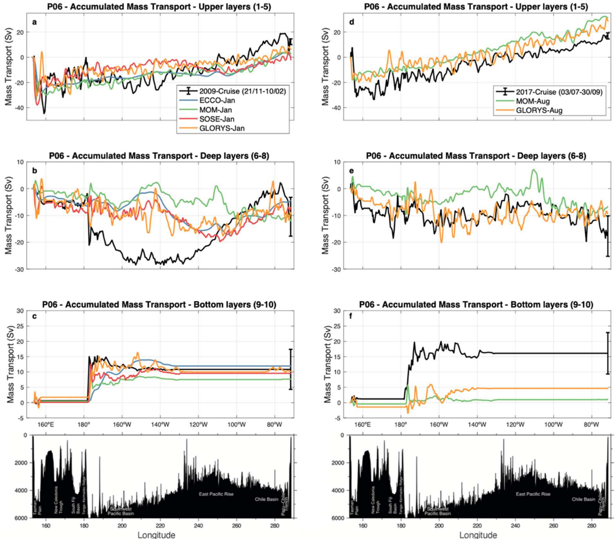
Fig. 11. Eastward accumulated mass transport (Sv) at 32°S in the Pacific Ocean for (a, d) upper, (b, e) deep, and (c, f) bottom layers for 2009 and 2017, respectively, estimated from hydrographic data and from the ocean models ECCO, SOSE, GLORYS, and MOM.
