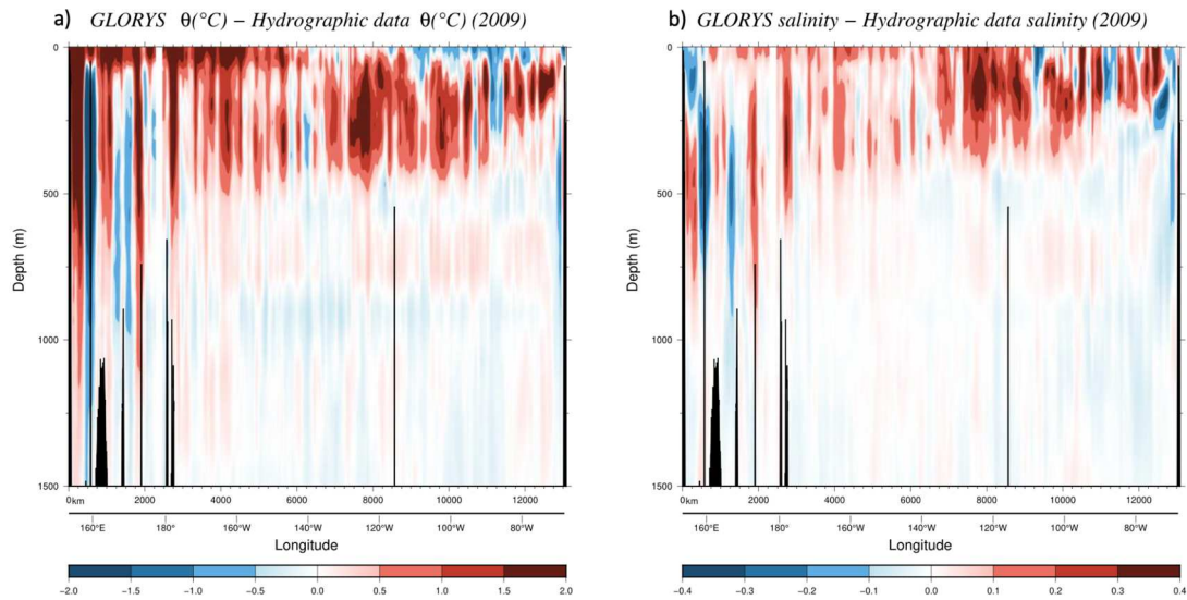
Fig. 15. Vertical sections for the GLORYS data and hydrographic data differences of (a) potential temperature (°C) and (b) salinity along section P06 in the Pacific Ocean.
