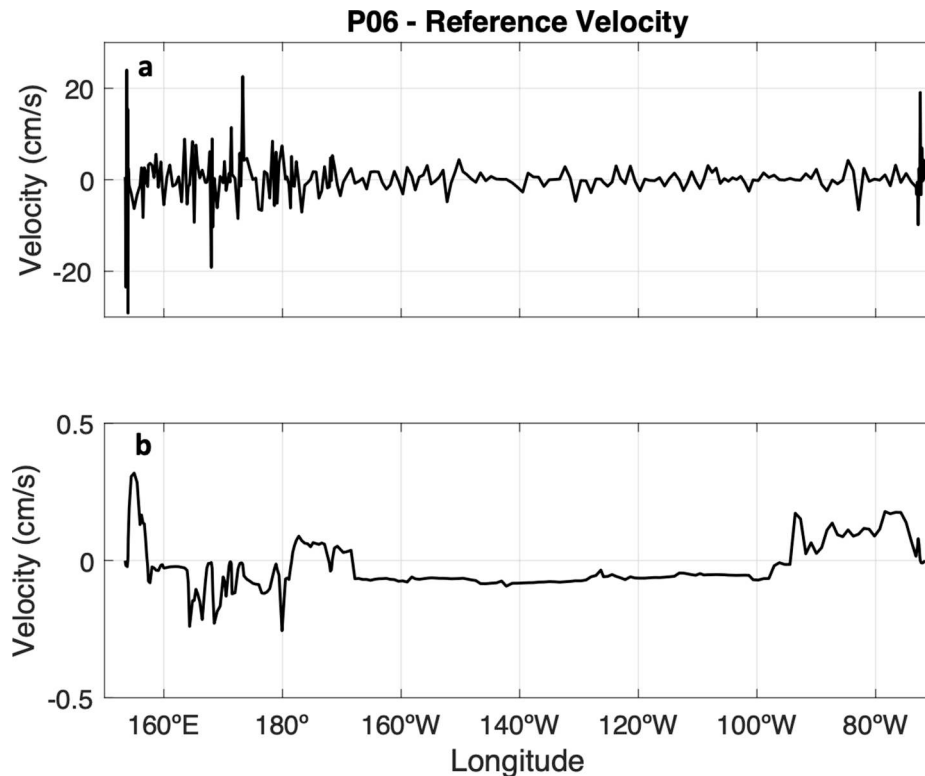
Fig. 5. Geostrophic velocity (cm/s) adjusted to the SADCP or LADCP data (a) and reference velocities from the inverse model (b) at each station pair for 2017 P06 section at nominally 32°S in the Pacific Ocean.
