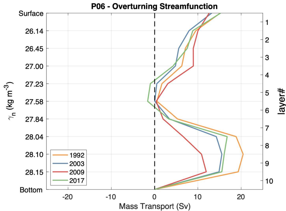
Fig. 7. Overturning mass transport streamfunction across 32°S in the Pacific Ocean for 1992, 2003, 2009 and 2017. This function is computed as the zonally- and vertically-integrated mass transports in isoneutral layers (along the entire section and from the seafloor to the sea surface).
