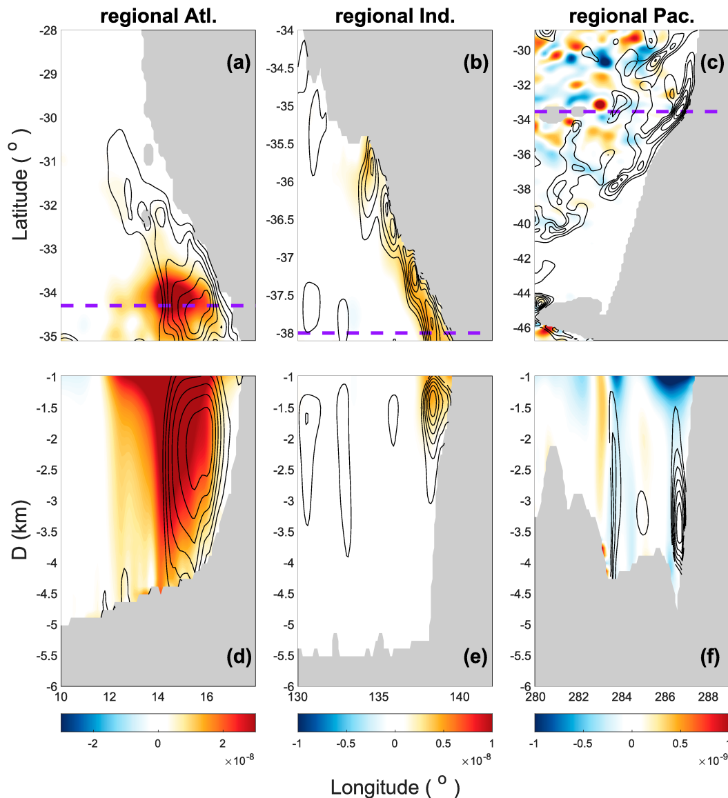
FIG. 10. Eddy momentum flux divergence in the meridional momentum equation ( -\nabla_h \cdot \overline{\mathbf{u}\mathbf{v}} , including both diagonal and off-diagonal eddy stress elements) for the regional MITgcm experiments for (top) horizontal and (bottom) vertical sections for the (a),(d) southeastern Atlantic Ocean (depth: 2.5 km; latitude: 34°S); (b),(e) southeastern Indian Ocean (depth: 1.3 km; latitude: 38°S); and (c),(f) southeastern Pacific Ocean (depth: 3.2 km; latitude: 33.5°S). The dashed purple lines in (a)–(c) indicate the latitude at which the vertical sections are taken. Different color ranges are used for different regional simulations.
