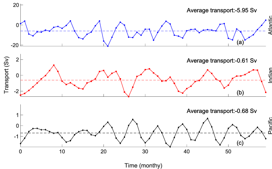
FIG. 12. Time series of the meridional transport in the region where time-averaged DEBCs emerge in the regional MITgcm experiments for the (a) Atlantic Ocean east of 14^{\circ}\text{E} , at 34^{\circ}\text{S} , and between 2- and 4-km depth; (b) Indian Ocean east of 138^{\circ}\text{E} , at 37.95^{\circ}\text{S} , and between 1- and 2-km depth; and (c) Pacific Ocean east of 286^{\circ}\text{E} , at 33.5^{\circ}\text{S} , and between 2- and 4-km depth. Dashed lines show the time-averaged transports.
