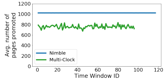
Fig. 8. The average amount of pages promoted in each scan over time. Y-axis is the average number of pages that are promoted in 20 seconds window. X-axis presents the time window IDs.
