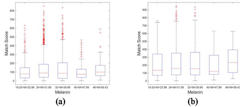
Figure 2 Match Scores VS Melanin Contactless (a) Contactless-1 (b) Contactless-2
