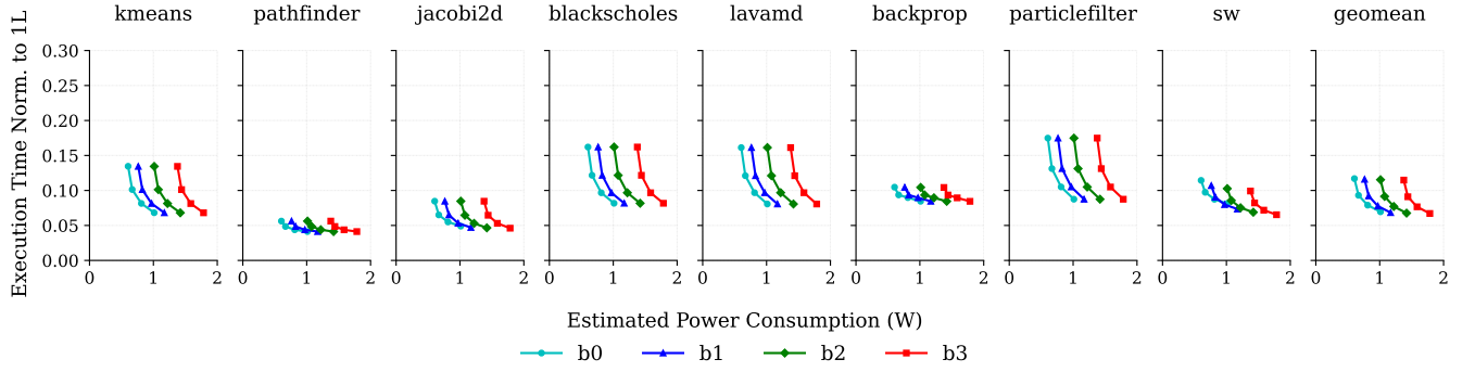
Figure 10. Execution Time and Estimated Power Consumption of 1b-4VL at Different Voltage/Frequency Levels - Each performance-power data point corresponds to a combination of big and little core's voltage/frequency levels shown in Table VII.
