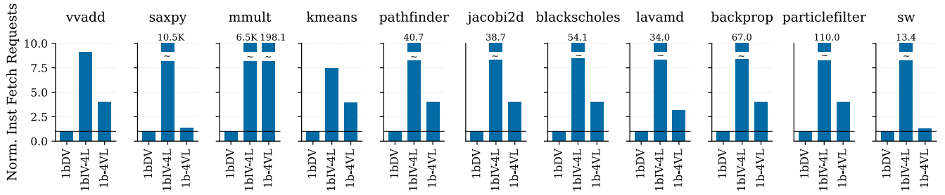
Figure 5. Number of Instruction Fetch Requests to Memory - All numbers are normalized to 1bDV .
