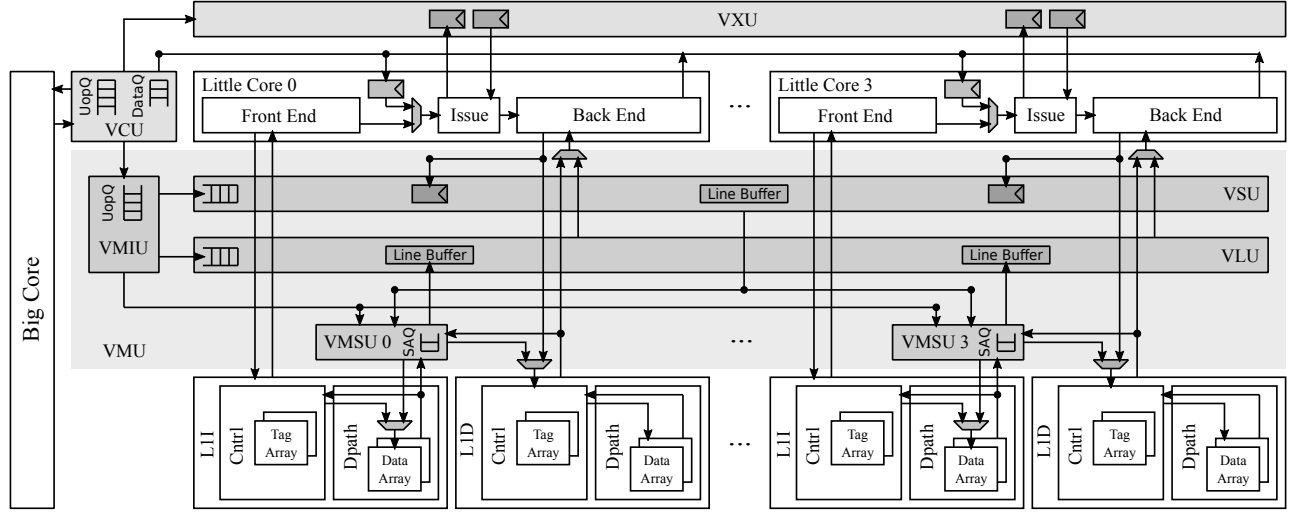
Figure 1. A big.VLITTLE system with One Big and Four LITTLE Cores – VCU = vector control unit; VXU = vector cross-element unit; VMU = vector memory unit; VMIU = vector memory issue unit; VMSU = vector memory slice unit; VLU = vector load unit; VSU = vector store unit; UopQ = micro-operation queue; DataQ = scalar data queue; SAQ = store-address queue. Components added to support the vector mode are shaded.
