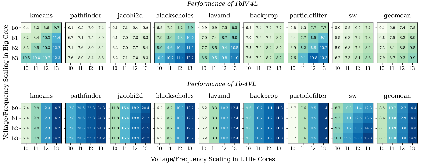
Figure 9. Performance of 1bIV-4L and 1b-4VL at Different Voltage/Frequency Scaling Levels for Big and Little Cores - All studied voltage/frequency levels (i.e., \{b0, b1, b2, b3\} and \{l0, l1, l2, l3\} ) are shown in Table VII. The performance numbers show speedup over 1L system running at 1GHz. The color scaling for each application is the same for both 1bIV-4L and 1b-4VL.
