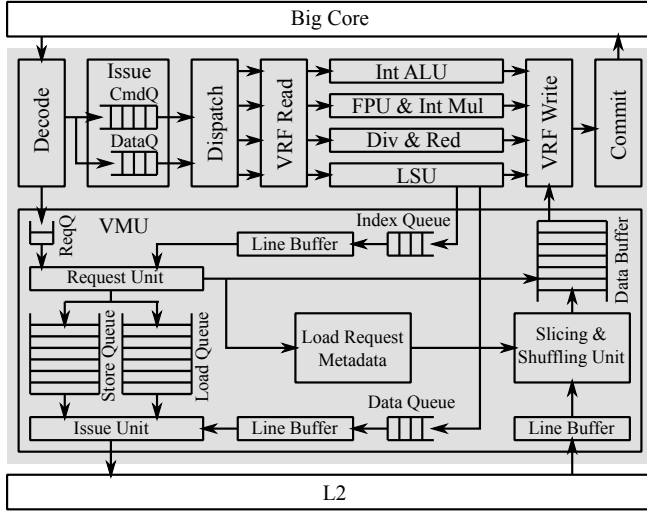
Figure 3. A Decoupled Vector Engine – CmdQ = command queue; DataQ = scalar data queue; VRF = vector register file; Int ALU = integer arithmetic & logic unit; FPU = floating-point unit; Int Mul = integer multiplication unit; Div = division unit; Red = reduction unit; LSU = load store unit; ReqQ = request queue.
