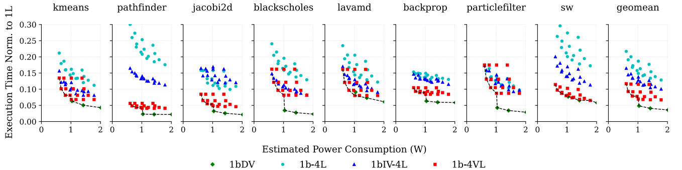
Figure 11. Execution Time and Estimated Power Consumption of Multiple Designs at Different Frequencies - The dotted lines show Pareto frontier curves. Each performance-power data point corresponds to a combination of big and little core's voltage/frequency levels shown in Table VII.
