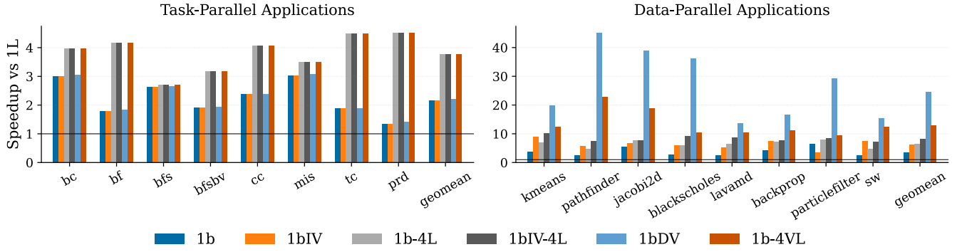
Figure 4. Speedup over 1L - 1L = one little core; 1b = one big core; 1bIV = one big core with an integrated vector unit; 1b-4L = one big & four little cores; 1bIV-4L = one big core with an integrated vector unit & four little cores; 1bDV = one big core with a decoupled vector engine; 1b-4VL = big.VLITTLE system with one big and a VLITTLE engine of four little cores.
