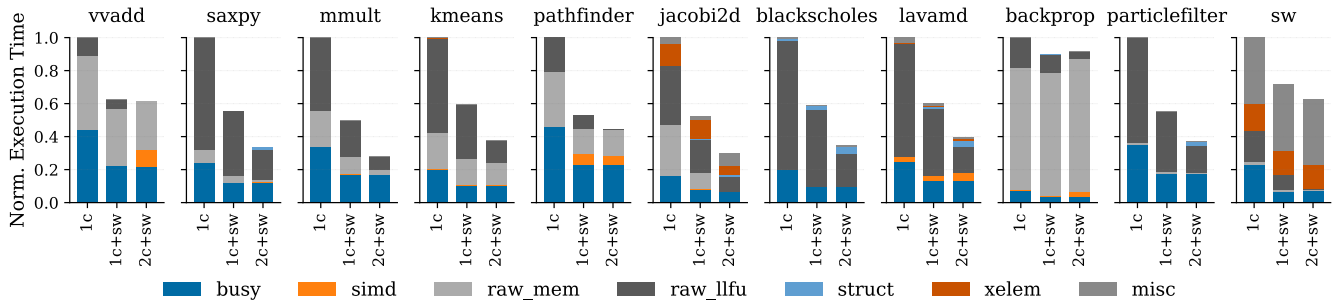
Figure 7. Average Execution Time Breakdown of Four Little Cores in 1b-4VL - 1c = 1b-4VL with one chime (vector element group); 1c+sw = 1b-4VL with one chime & packed vector elements; 2c+sw = 1b-4VL with two chimes & packed vector elements; busy = cycles in which little cores are not stalled; simd = stalled cycles due to lock-step issuing of micro-ops in the VCU; raw_mem = stalled cycles due to waiting for memory; raw_llfu = stalled cycles due to little cores waiting for long-latency micro-ops to complete; struct = stalled cycles due to structural hazards; xelem = stalled cycles due to cross-element micro-ops; misc = other stalled cycles (e.g., no micro-op from the VCU).
