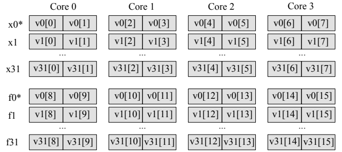
Figure 2. Mapping of 32-bit Vector Elements to Scalar 64-bit Registers in Four Little Cores – xN = scalar integer registers. fN = scalar floating point registers. vN[m] = m -th element in a vector register. Elements of the vector register 0 are mapped to newly added physical registers x0^* and f0^* in little cores.
