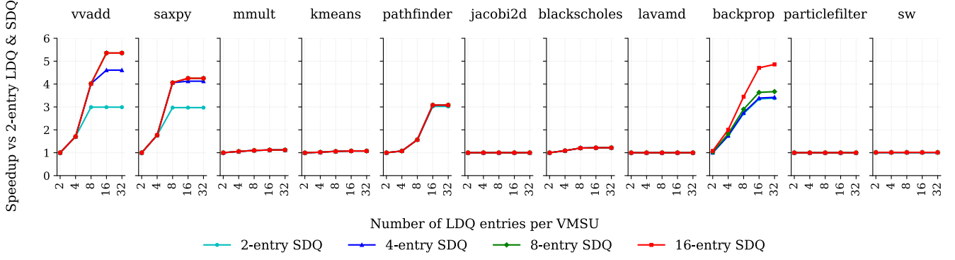
Figure 8. Performance Impacts of VMU's Load Data Queue (LDQ) and Store Data Queue (SDQ)
